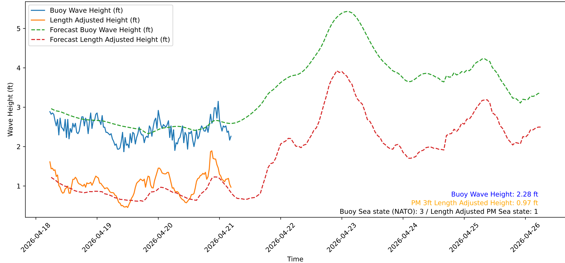
Wave Heights over Time for Green Beach at 2026-04-21 05:31:13
