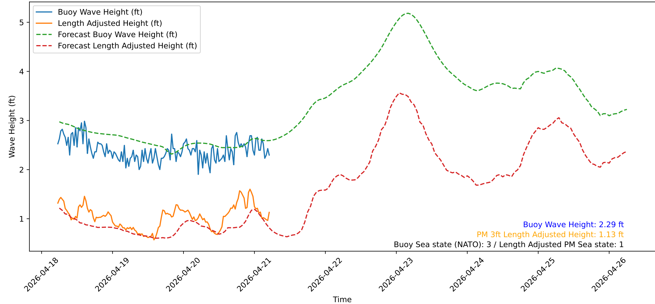
Wave Heights over Time for Oceanside Harbor at 2026-04-21 05:30:32
