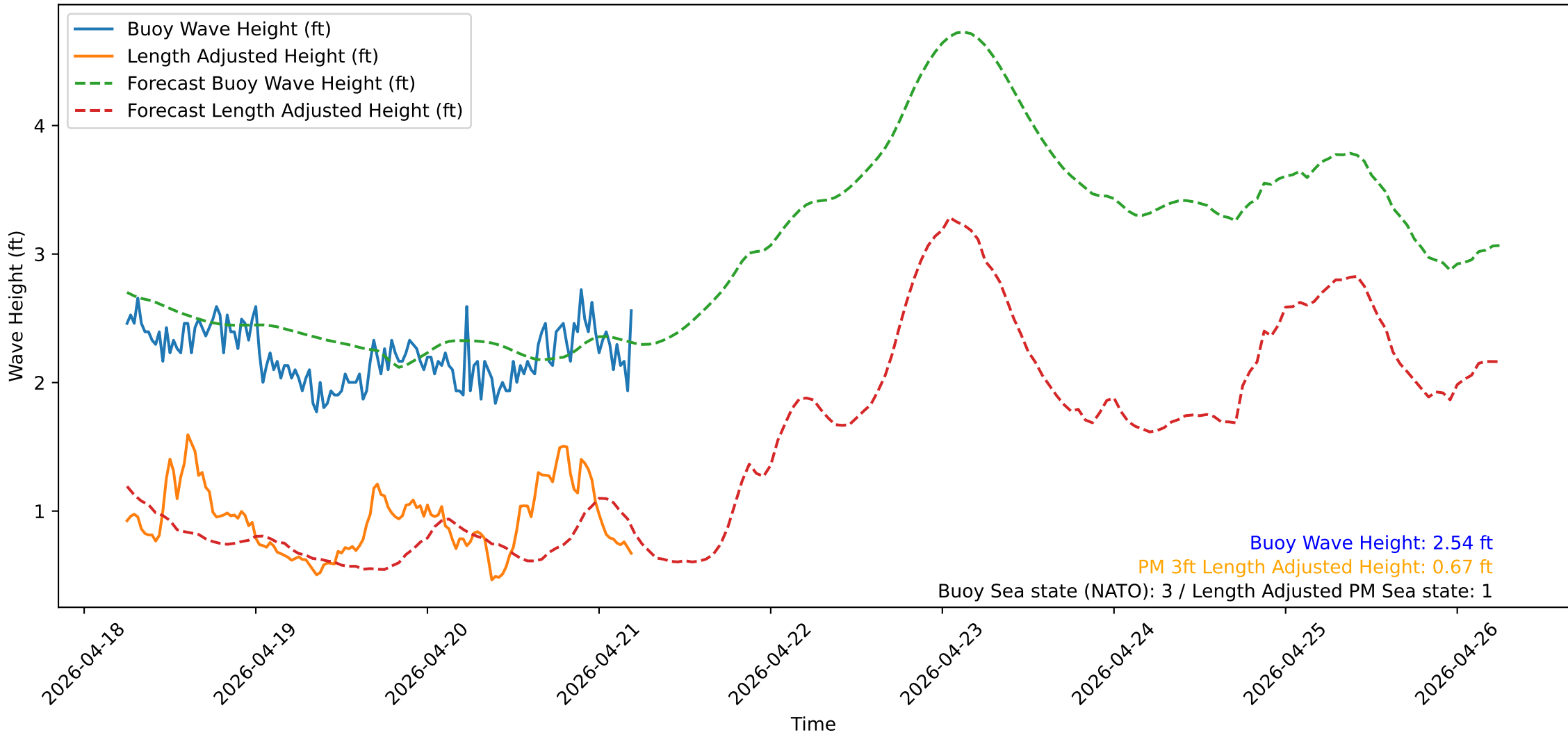
Wave Heights over Time for Red Beach at 2026-04-21 05:30:51
