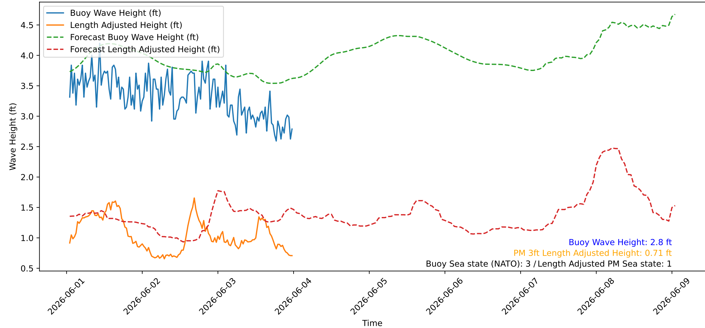
Wave Heights over Time for Red Beach at 2026-06-04 00:30:45
