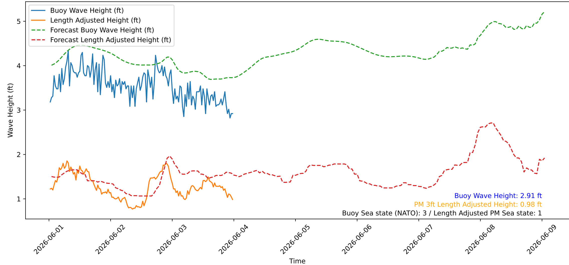
Wave Heights over Time for Green Beach at 2026-06-04 00:31:07
