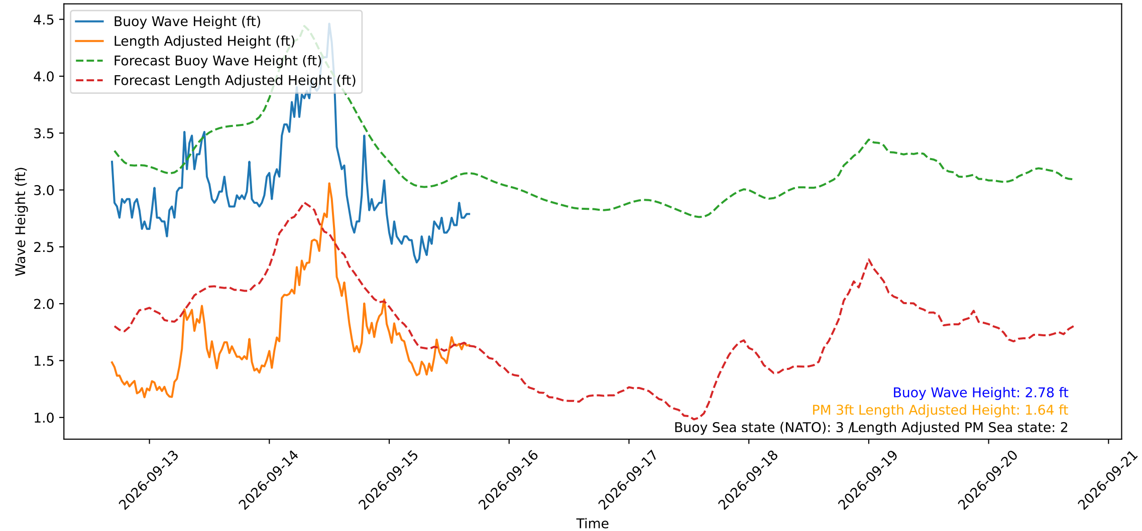
Wave Heights over Time for Oceanside Harbor at 2026-09-15 16:30:30
