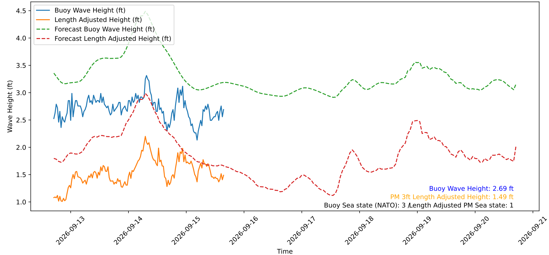
Wave Heights over Time for Green Beach at 2026-09-15 16:31:11
