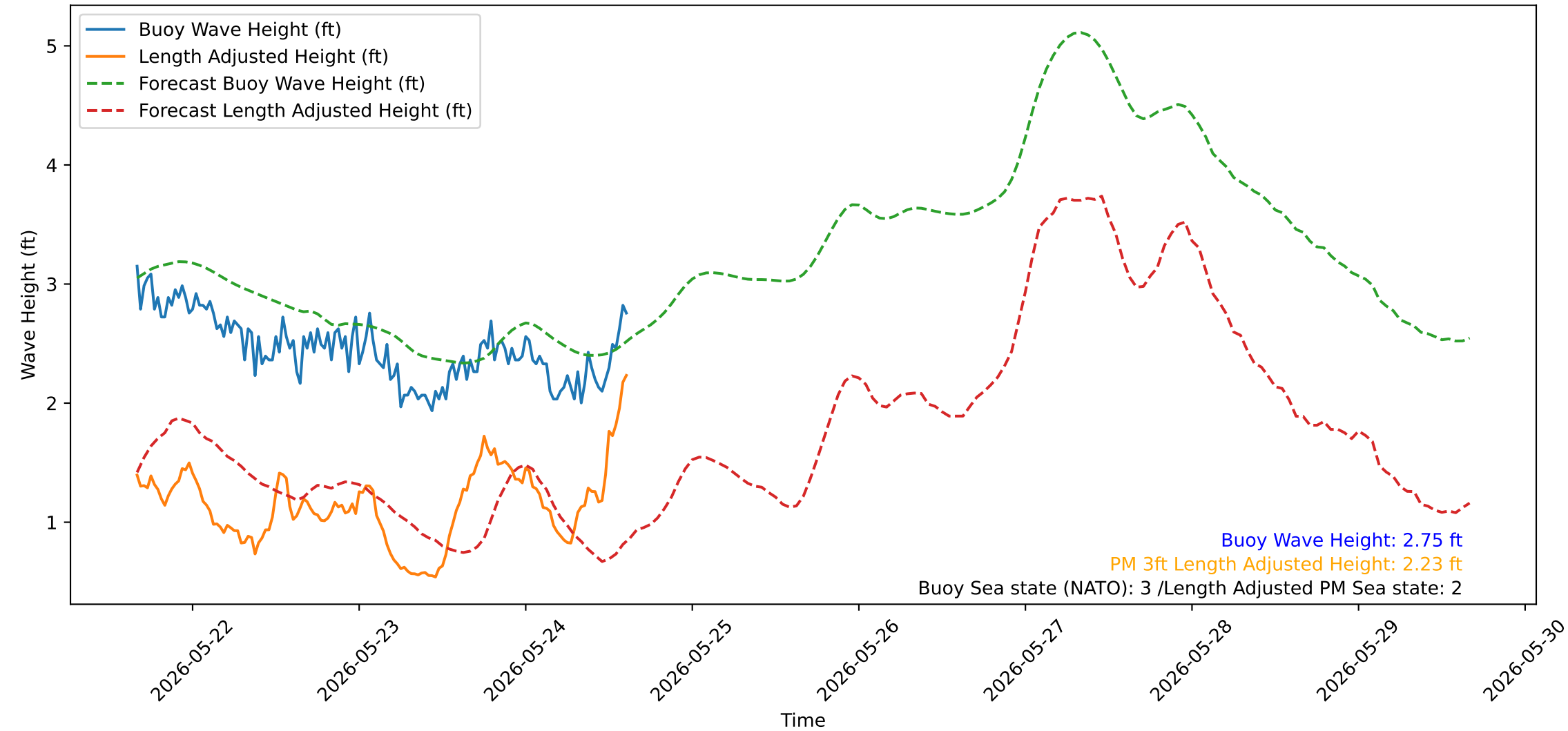
Wave Heights over Time for Red Beach at 2026-05-24 15:30:52
