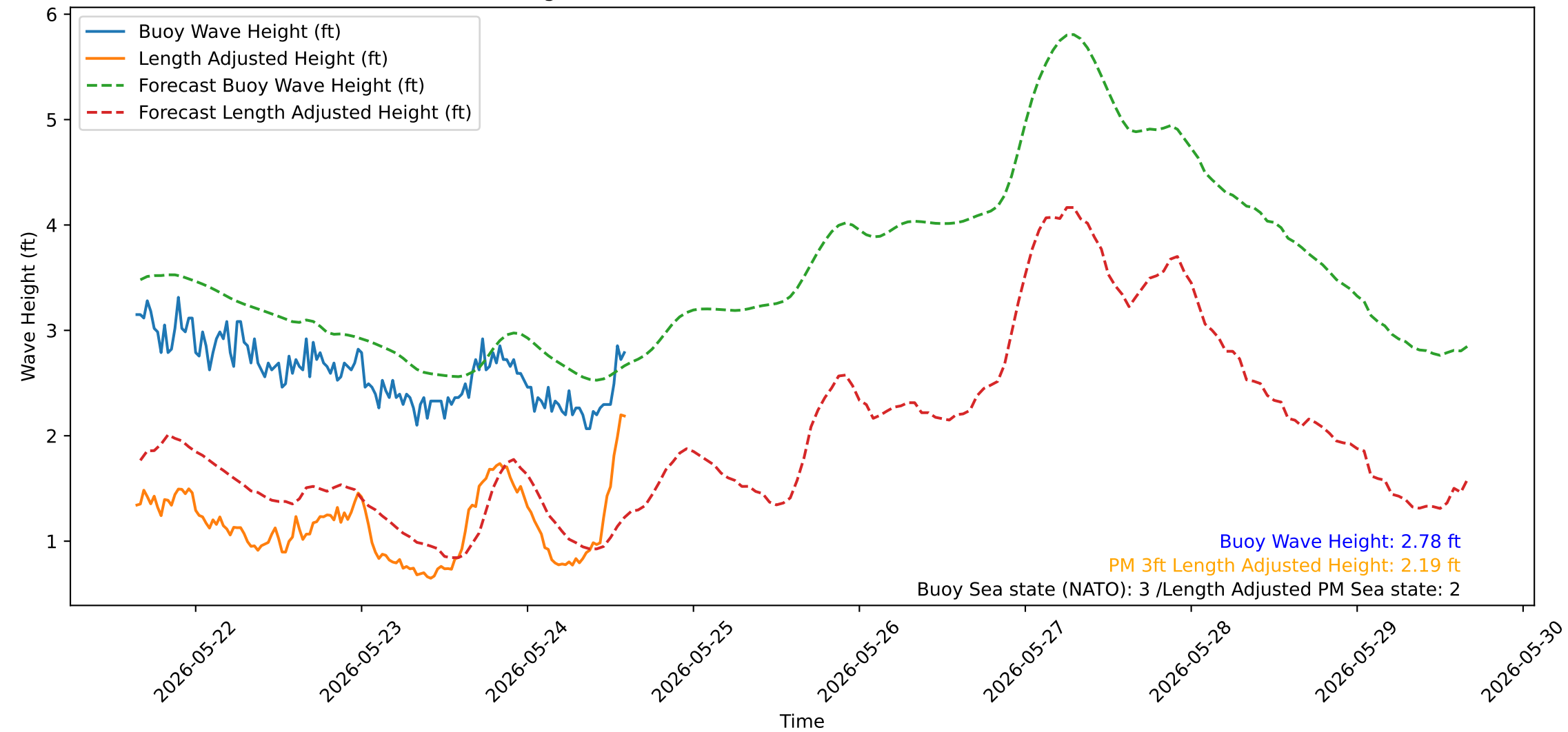
Wave Heights over Time for Green Beach at 2026-05-24 15:31:15
