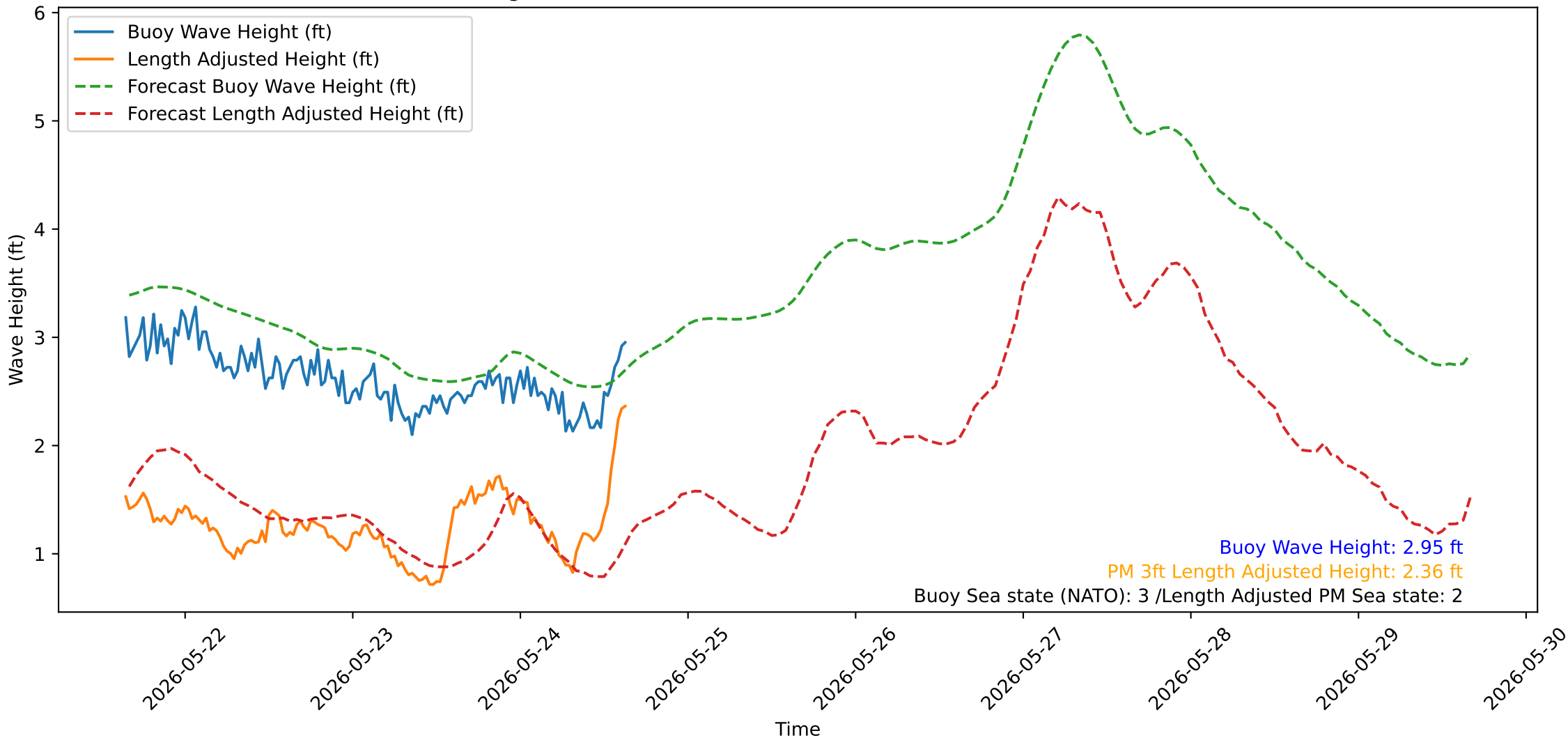
Wave Heights over Time for Oceanside Harbor at 2026-05-24 15:30:32
