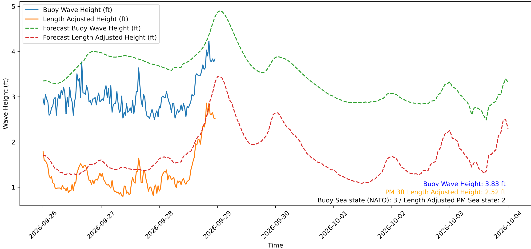
Wave Heights over Time for Oceanside Harbor at 2026-09-28 23:50:29
