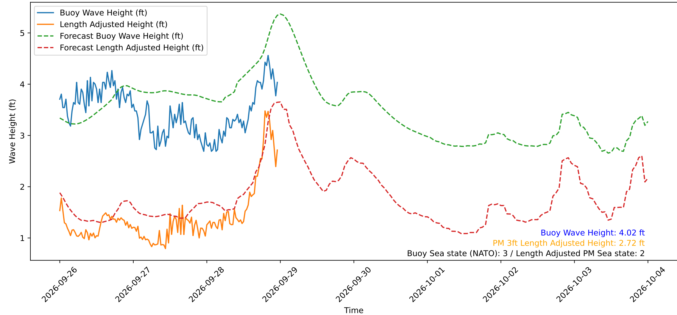
Wave Heights over Time for Green Beach at 2026-09-28 23:51:14
