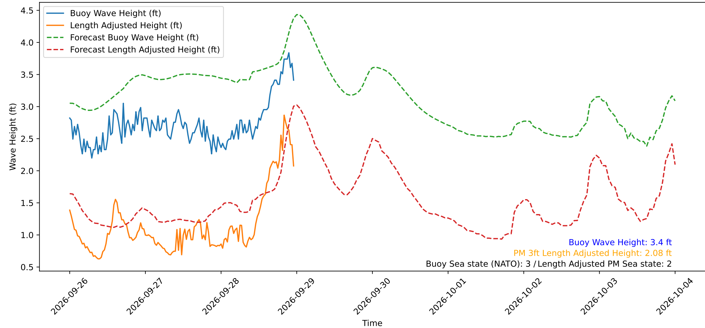
Wave Heights over Time for Red Beach at 2026-09-28 23:50:50
