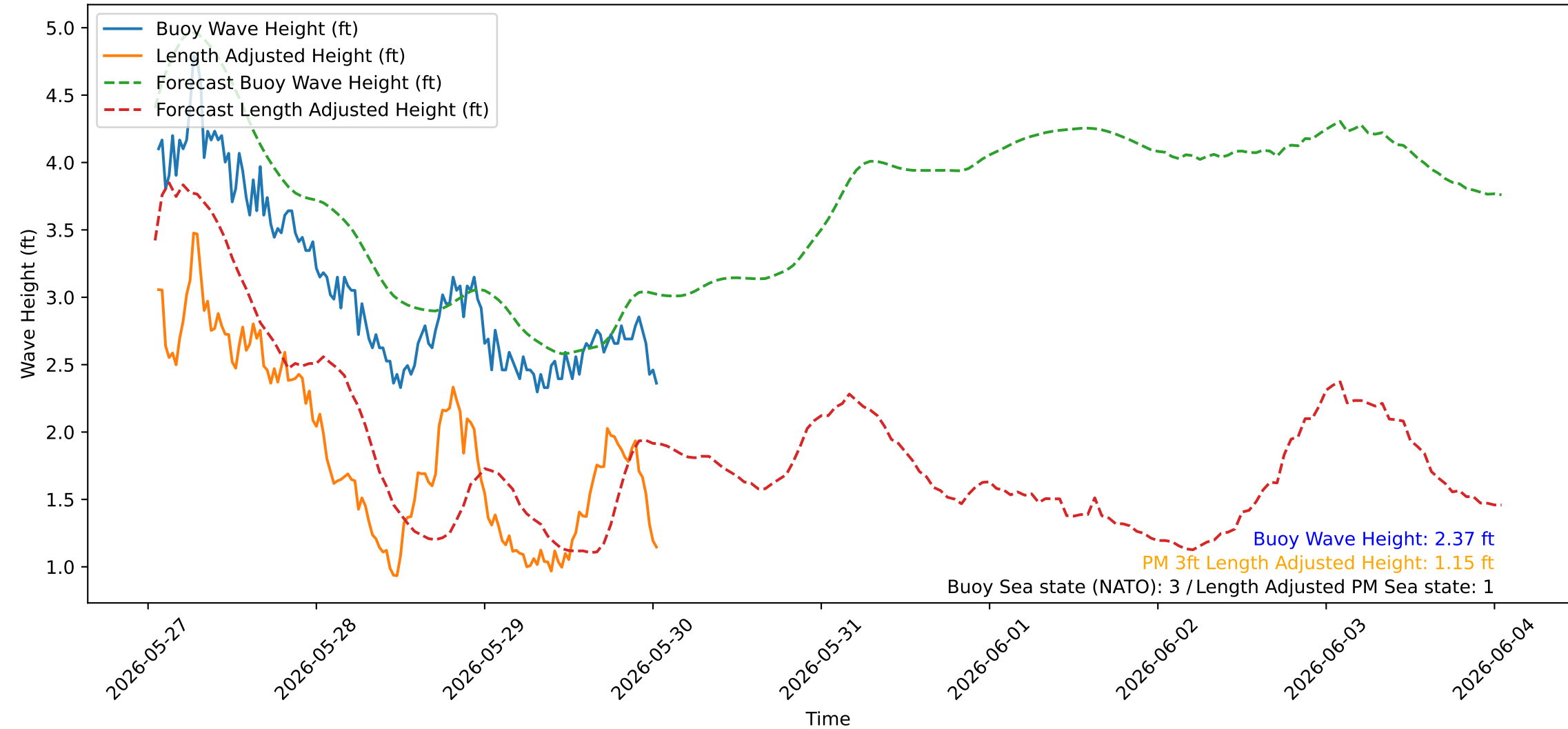
Wave Heights over Time for Red Beach at 2026-05-30 01:10:42
