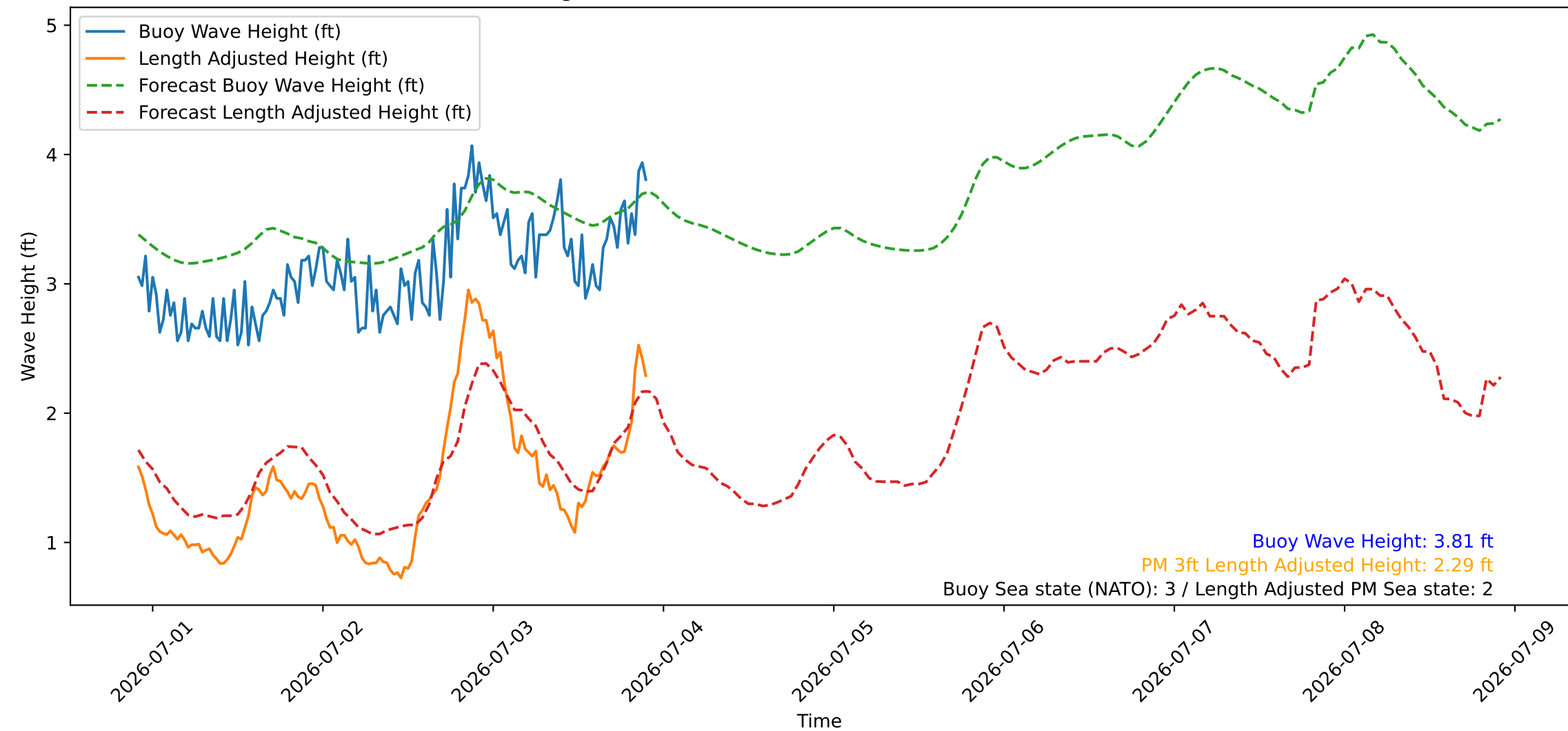
Wave Heights over Time for Green Beach at 2026-07-03 22:11:08
