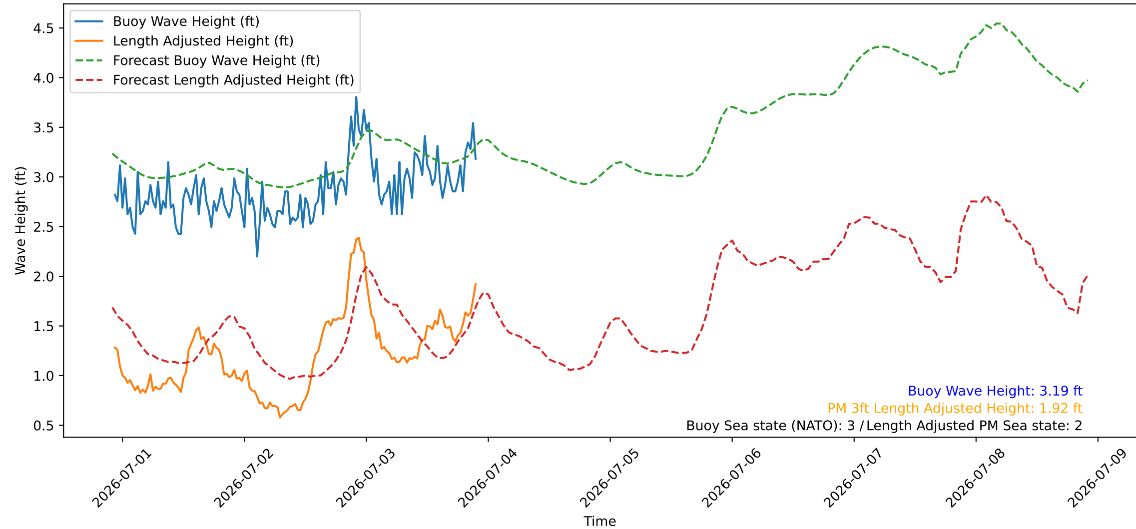
Wave Heights over Time for Red Beach at 2026-07-03 22:10:46
