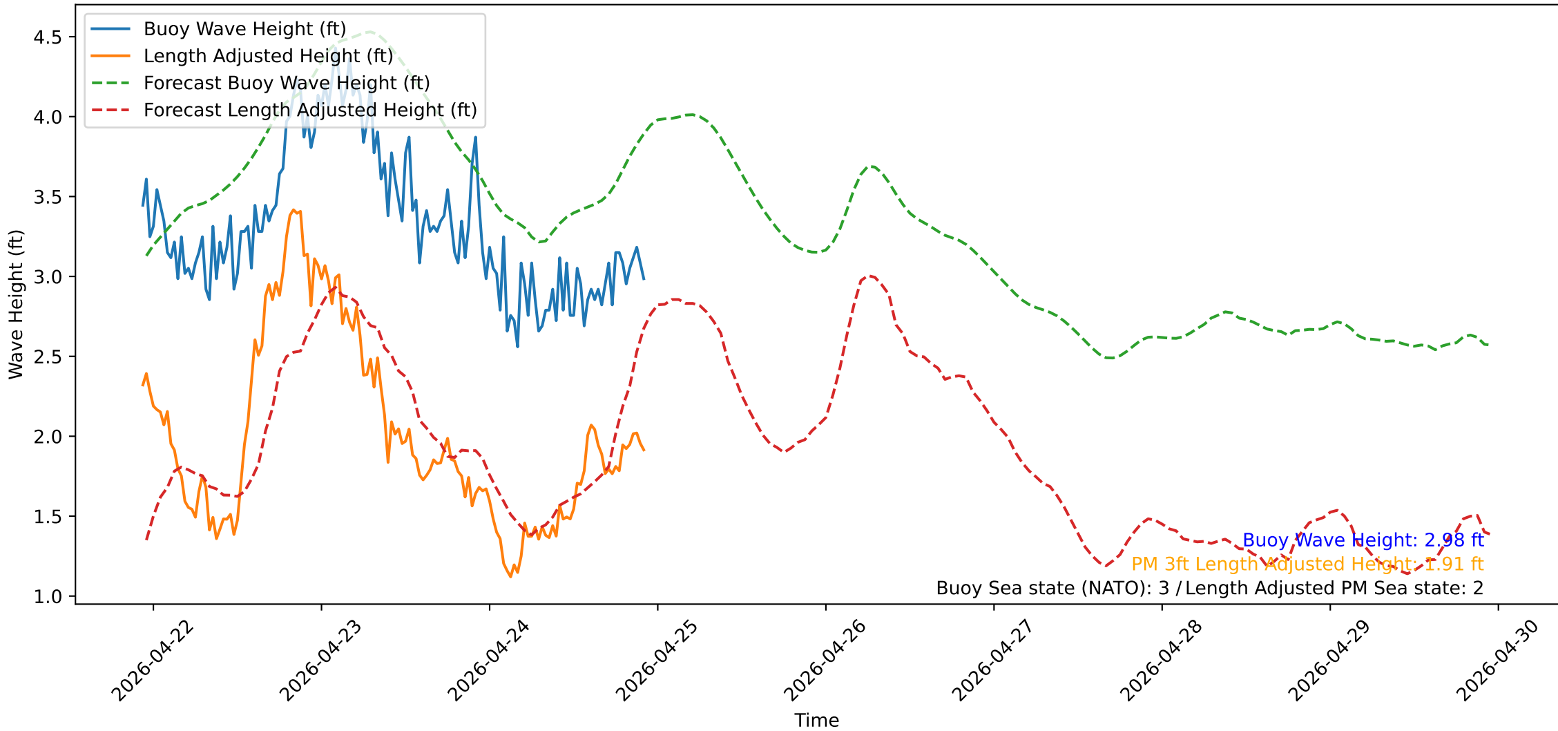
Wave Heights over Time for Oceanside Harbor at 2026-04-24 22:40:31
