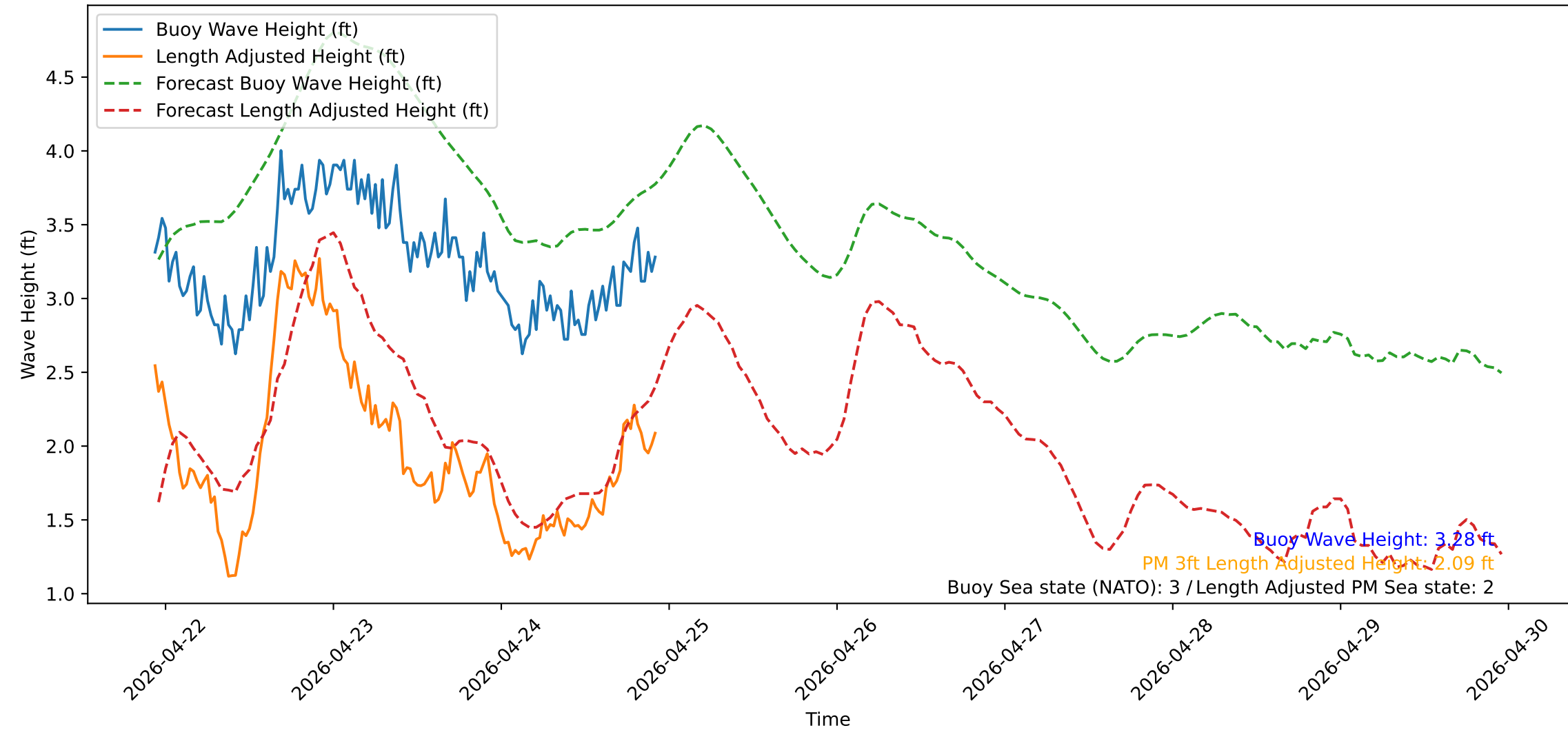
Wave Heights over Time for Green Beach at 2026-04-24 22:41:13
