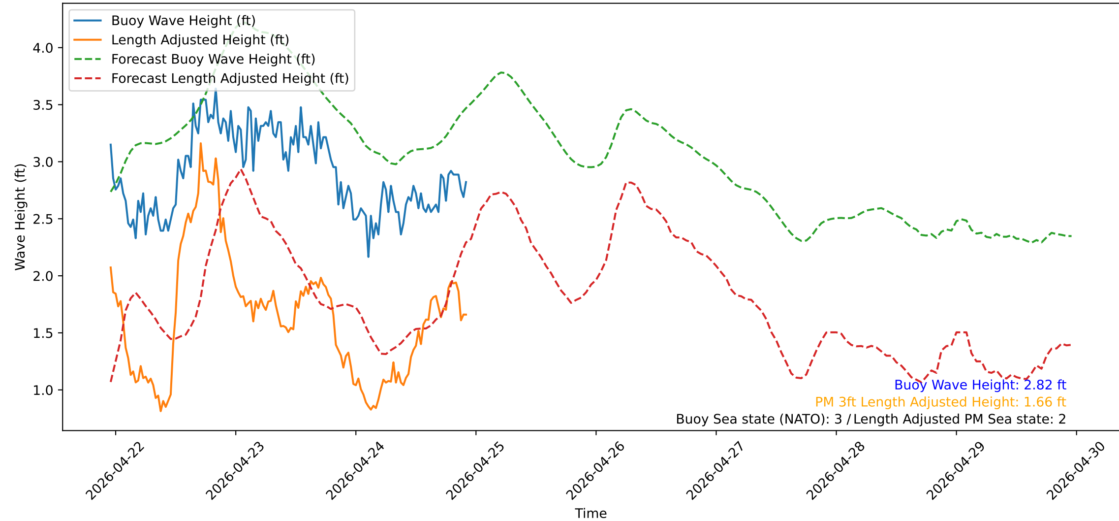
Wave Heights over Time for Red Beach at 2026-04-24 22:40:50
