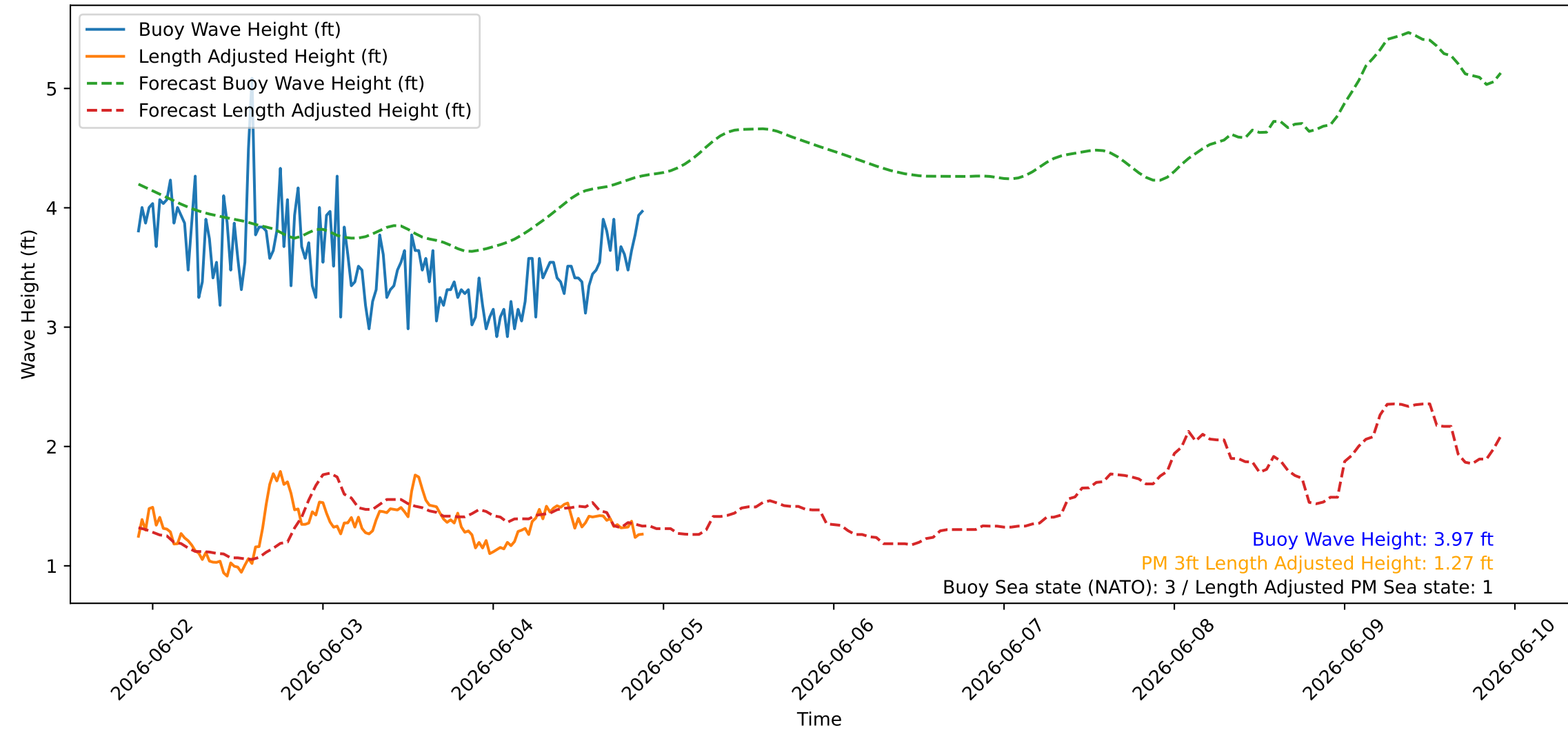
Wave Heights over Time for Oceanside Harbor at 2026-06-04 22:00:26
