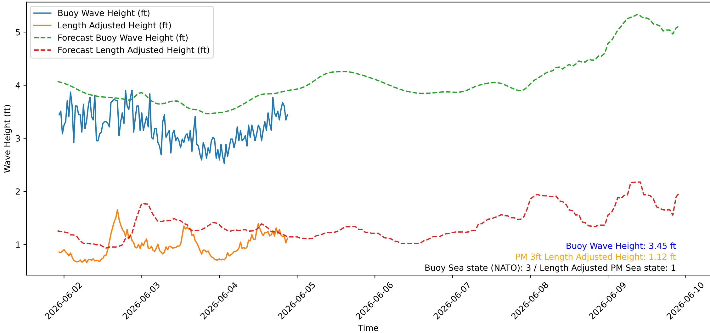
Wave Heights over Time for Red Beach at 2026-06-04 22:00:45
