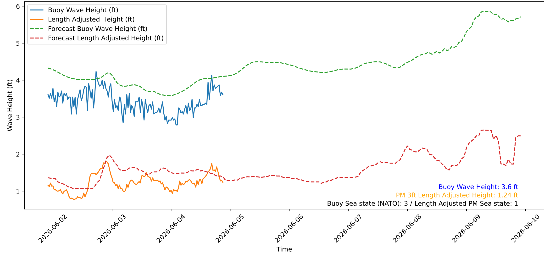
Wave Heights over Time for Green Beach at 2026-06-04 22:01:07
