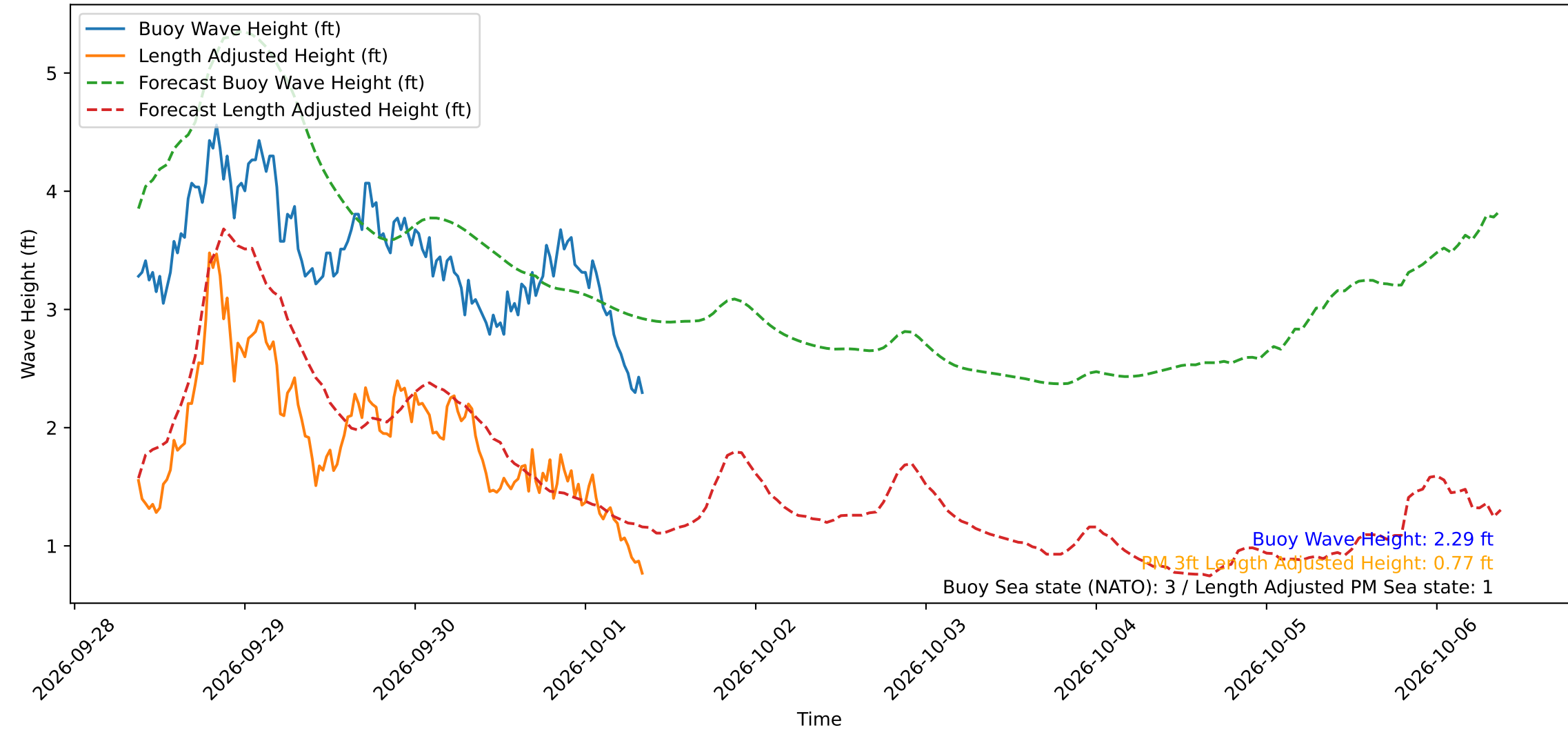
Wave Heights over Time for Green Beach at 2026-10-01 08:41:13
