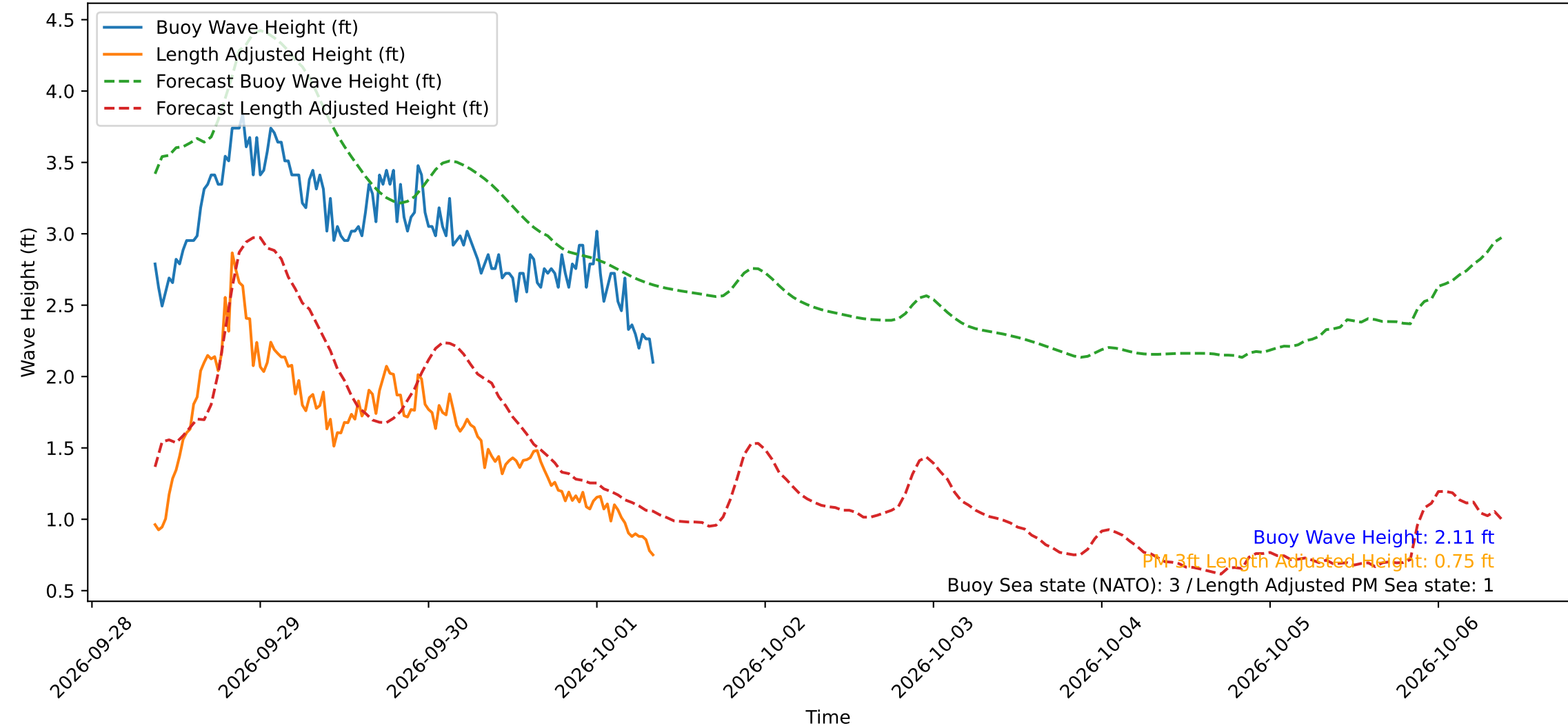
Wave Heights over Time for Red Beach at 2026-10-01 08:40:50
