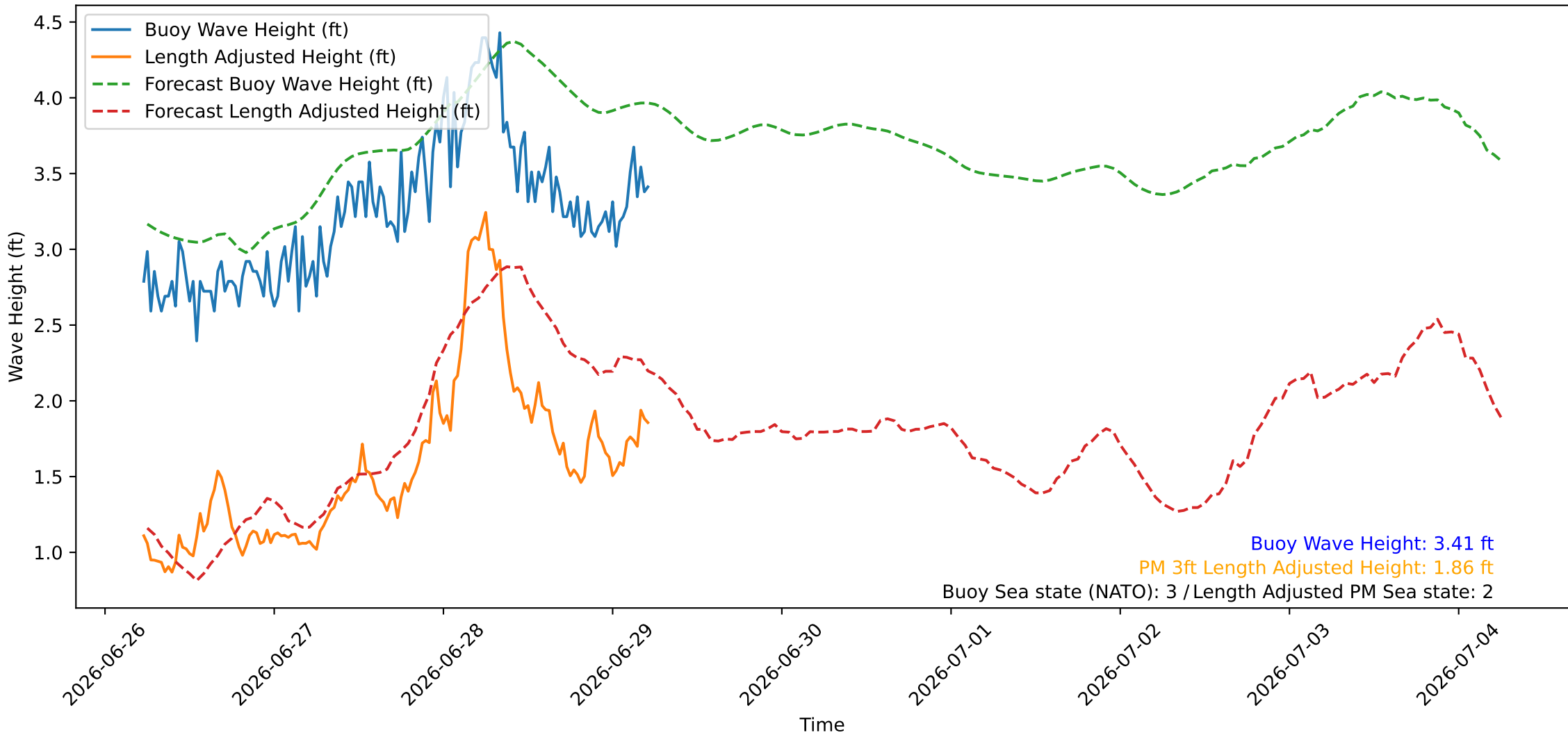
Wave Heights over Time for Oceanside Harbor at 2026-06-29 05:40:25
