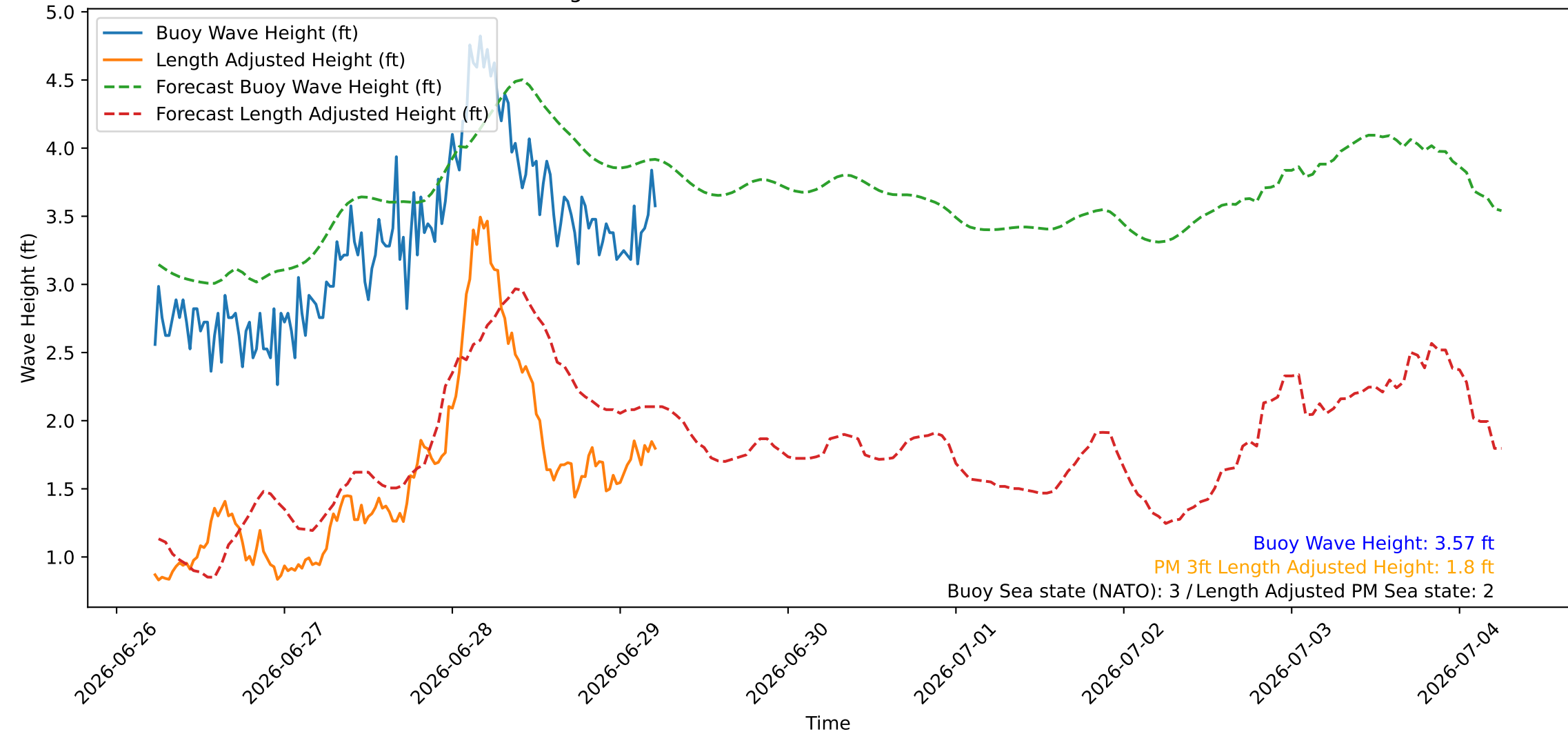
Wave Heights over Time for Green Beach at 2026-06-29 05:41:07
