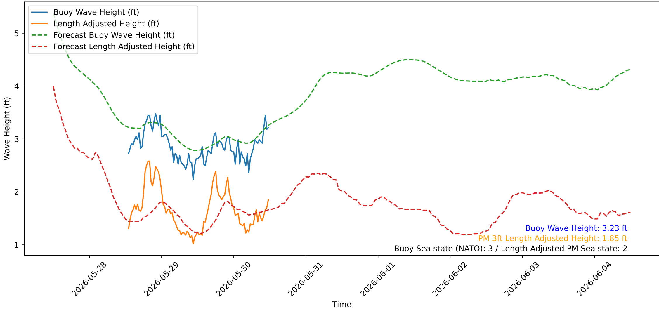
Wave Heights over Time for Oceanside Harbor at 2026-05-30 12:20:24
