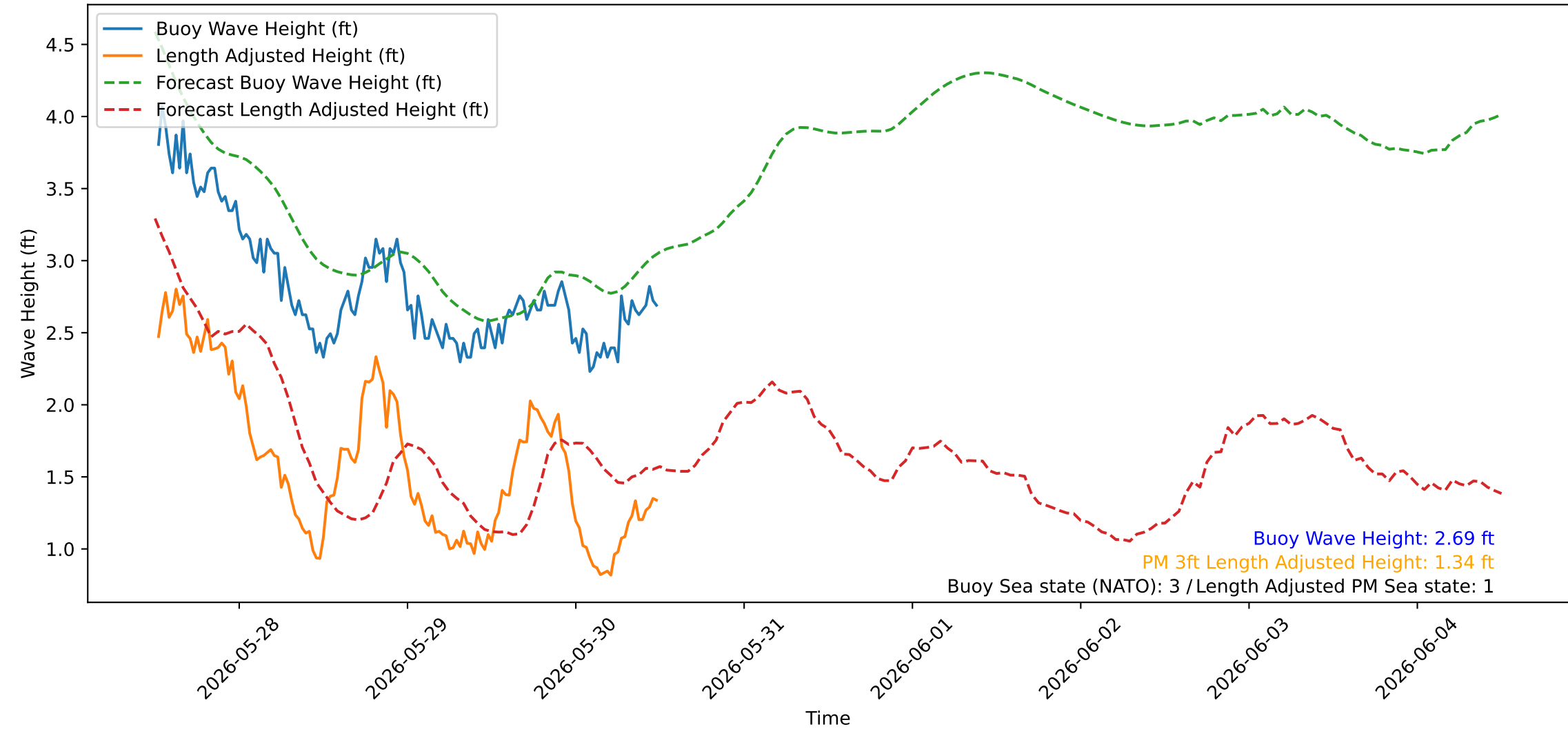
Wave Heights over Time for Red Beach at 2026-05-30 12:20:44
