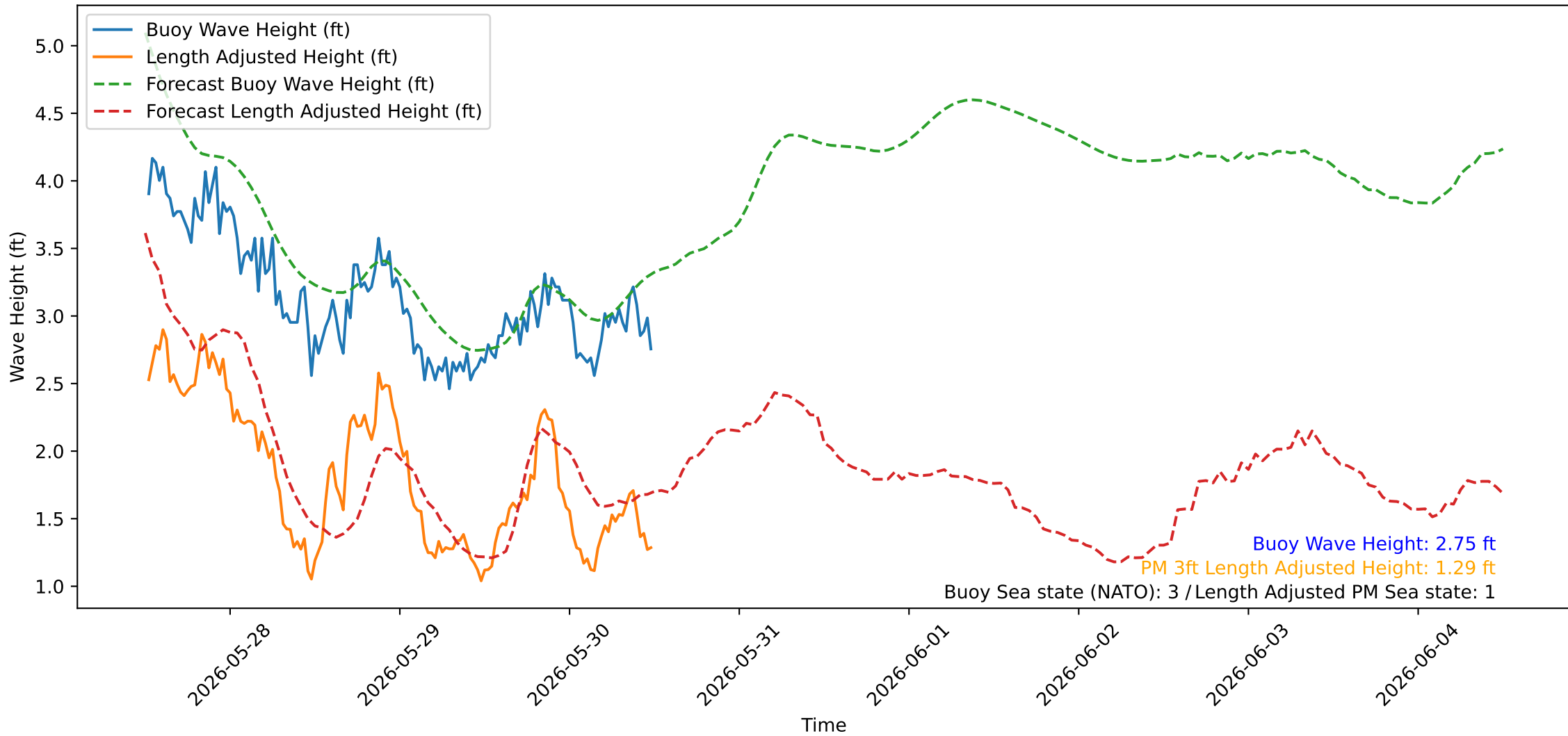
Wave Heights over Time for Green Beach at 2026-05-30 12:21:07
