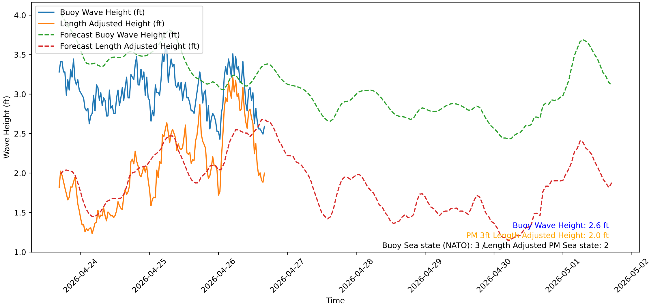
Wave Heights over Time for Green Beach at 2026-04-26 16:41:12
