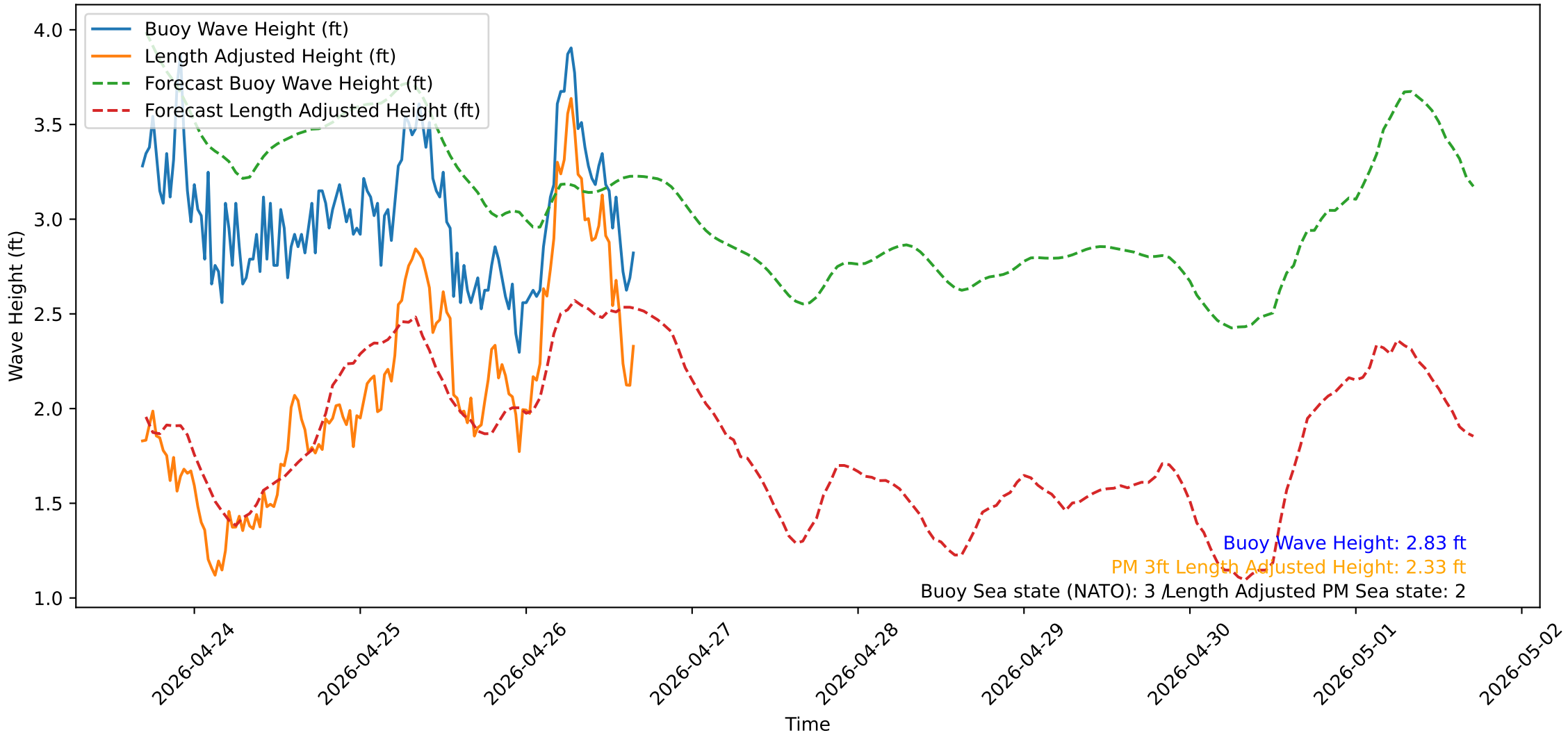
Wave Heights over Time for Oceanside Harbor at 2026-04-26 16:40:31
