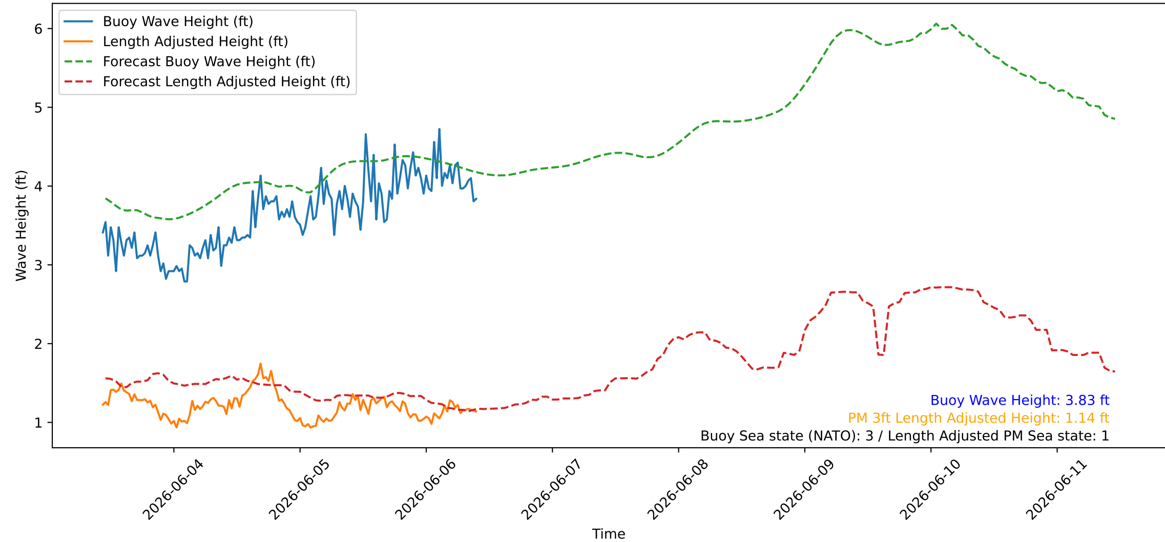
Wave Heights over Time for Green Beach at 2026-06-06 10:31:06
