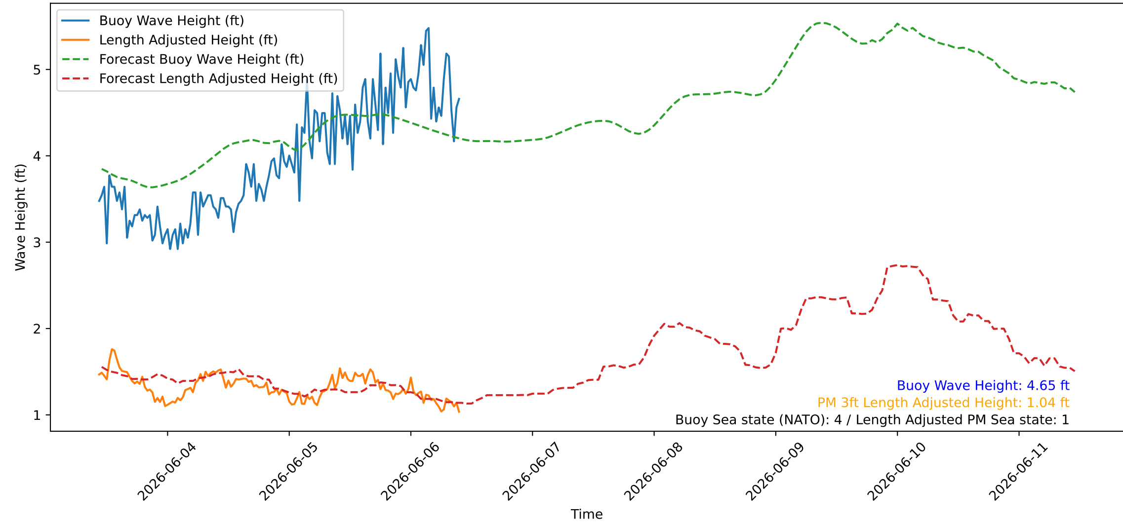
Wave Heights over Time for Oceanside Harbor at 2026-06-06 10:30:26
