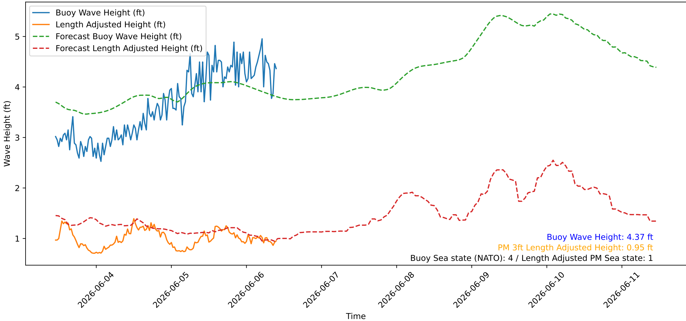
Wave Heights over Time for Red Beach at 2026-06-06 10:30:44
