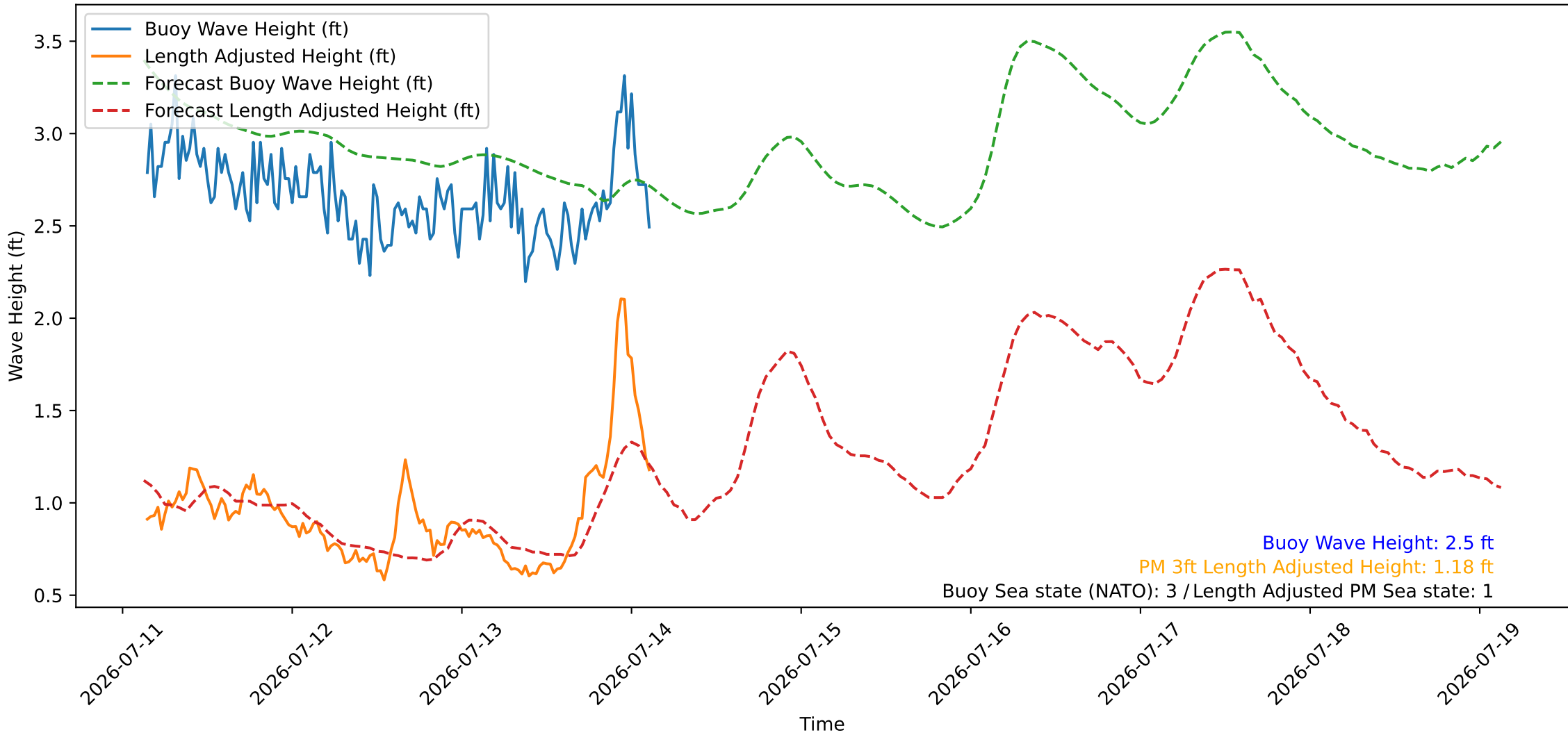
Wave Heights over Time for Green Beach at 2026-07-14 03:21:09
