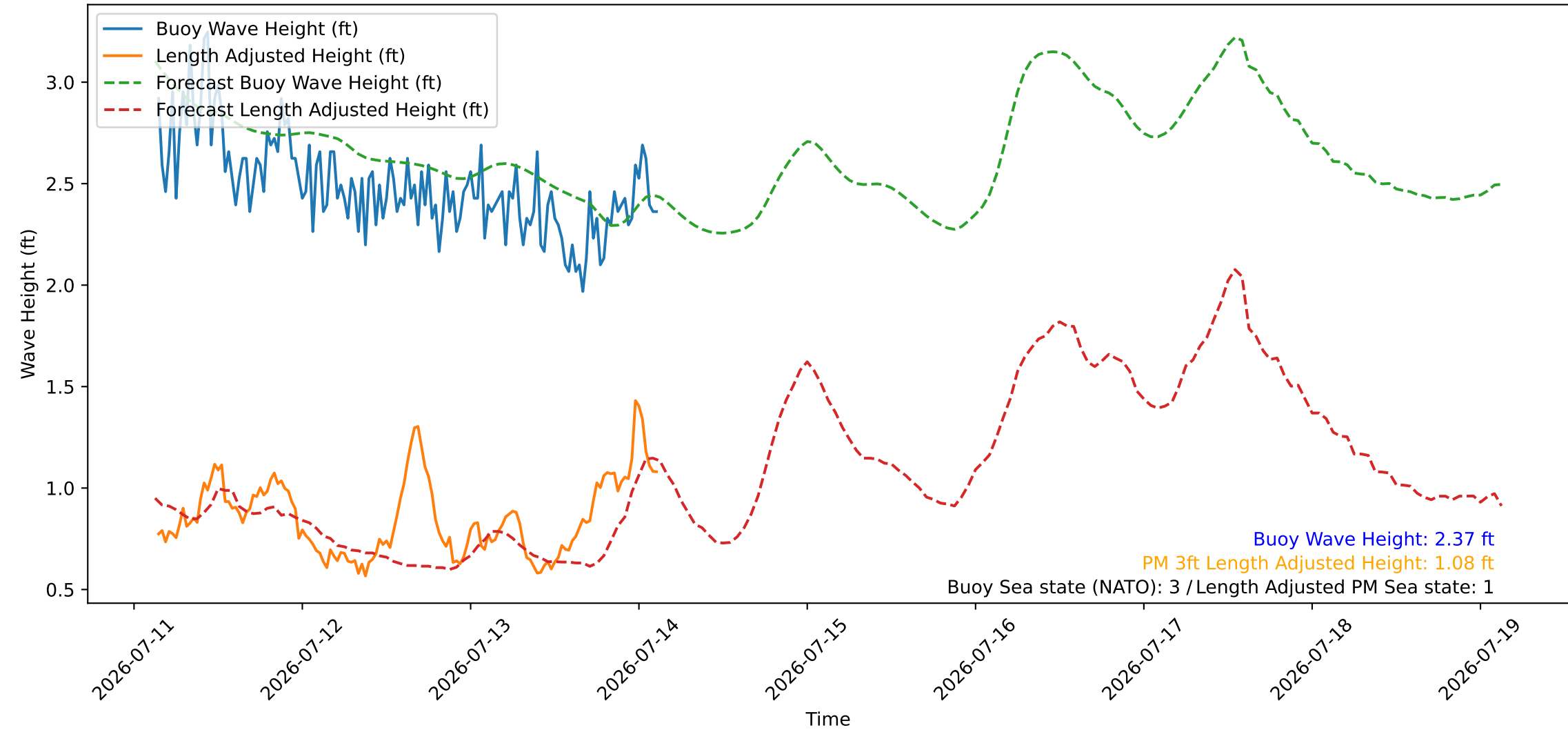
Wave Heights over Time for Red Beach at 2026-07-14 03:20:47
