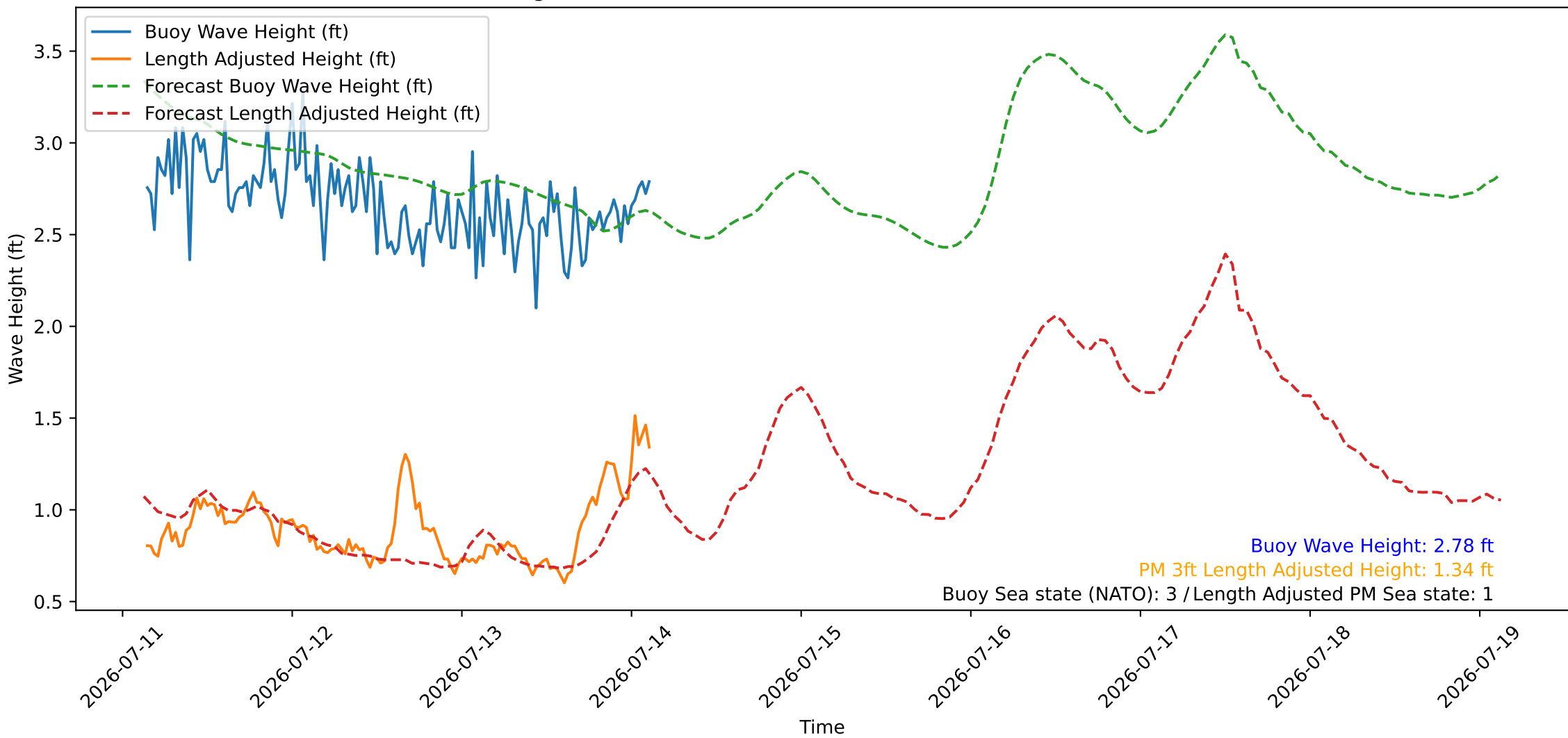
Wave Heights over Time for Oceanside Harbor at 2026-07-14 03:20:26
