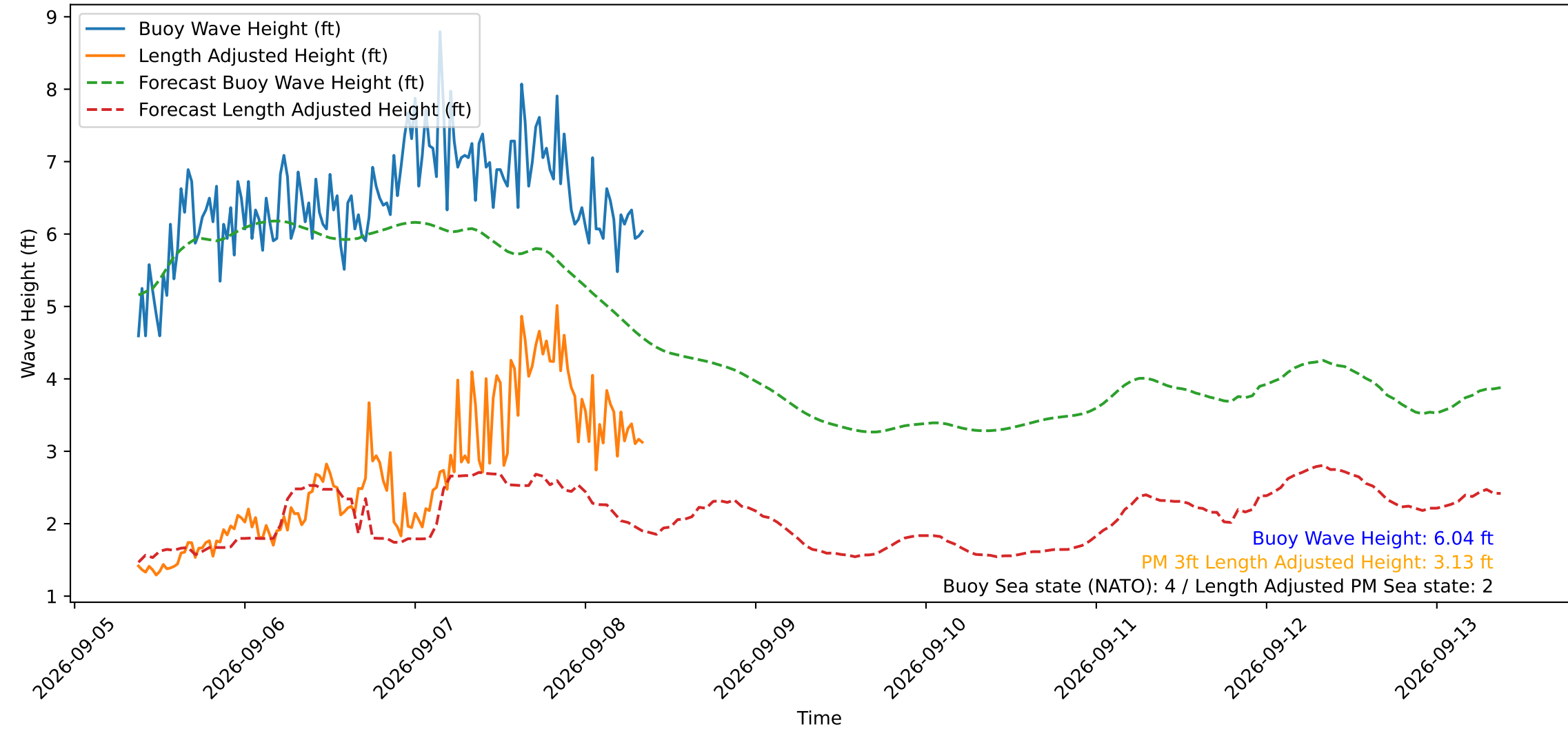
Wave Heights over Time for Green Beach at 2026-09-08 08:51:15
