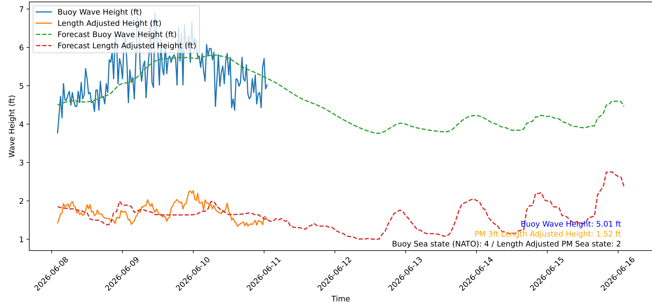
Wave Heights over Time for Green Beach at 2026-06-11 01:51:12
