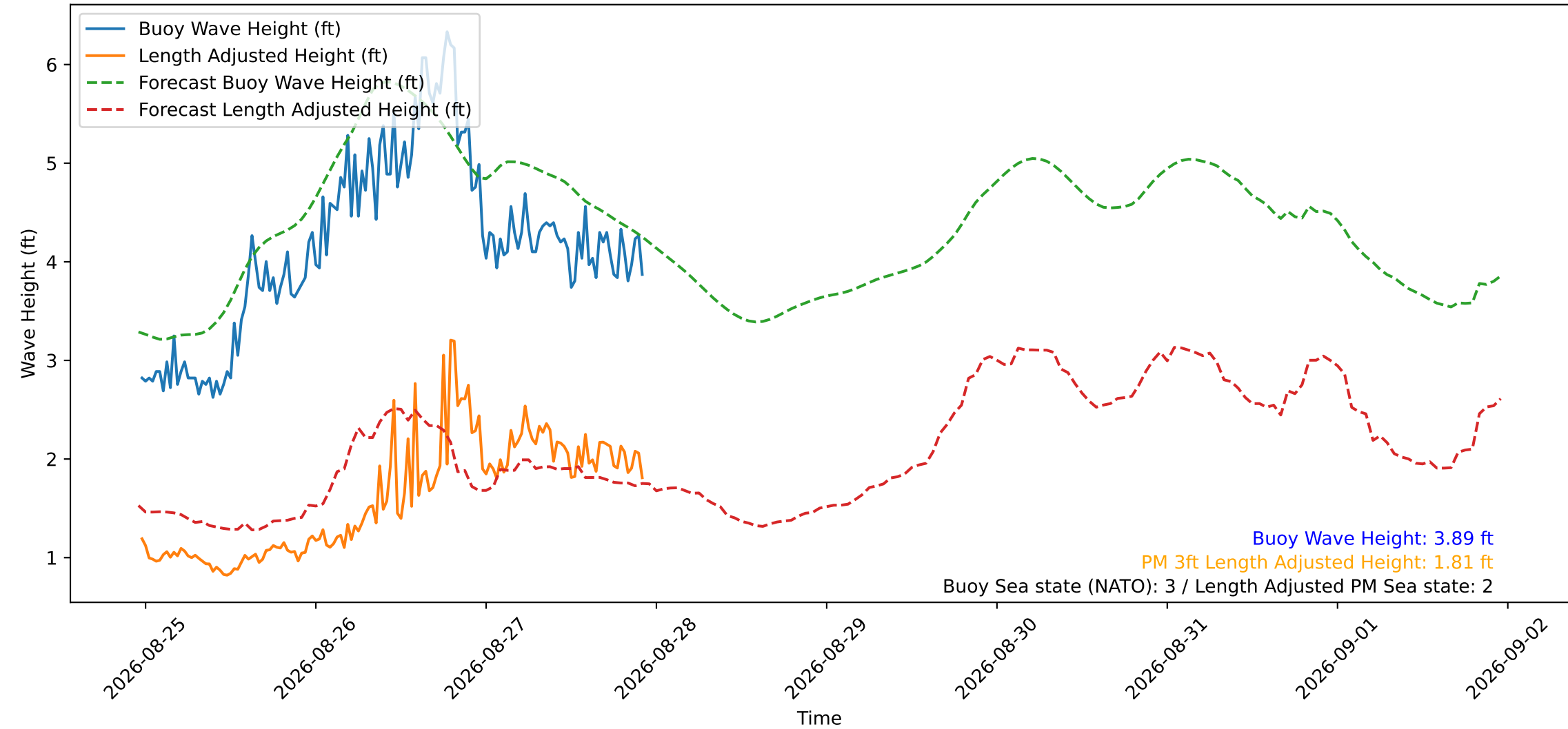
Wave Heights over Time for Green Beach at 2026-08-27 23:01:12
