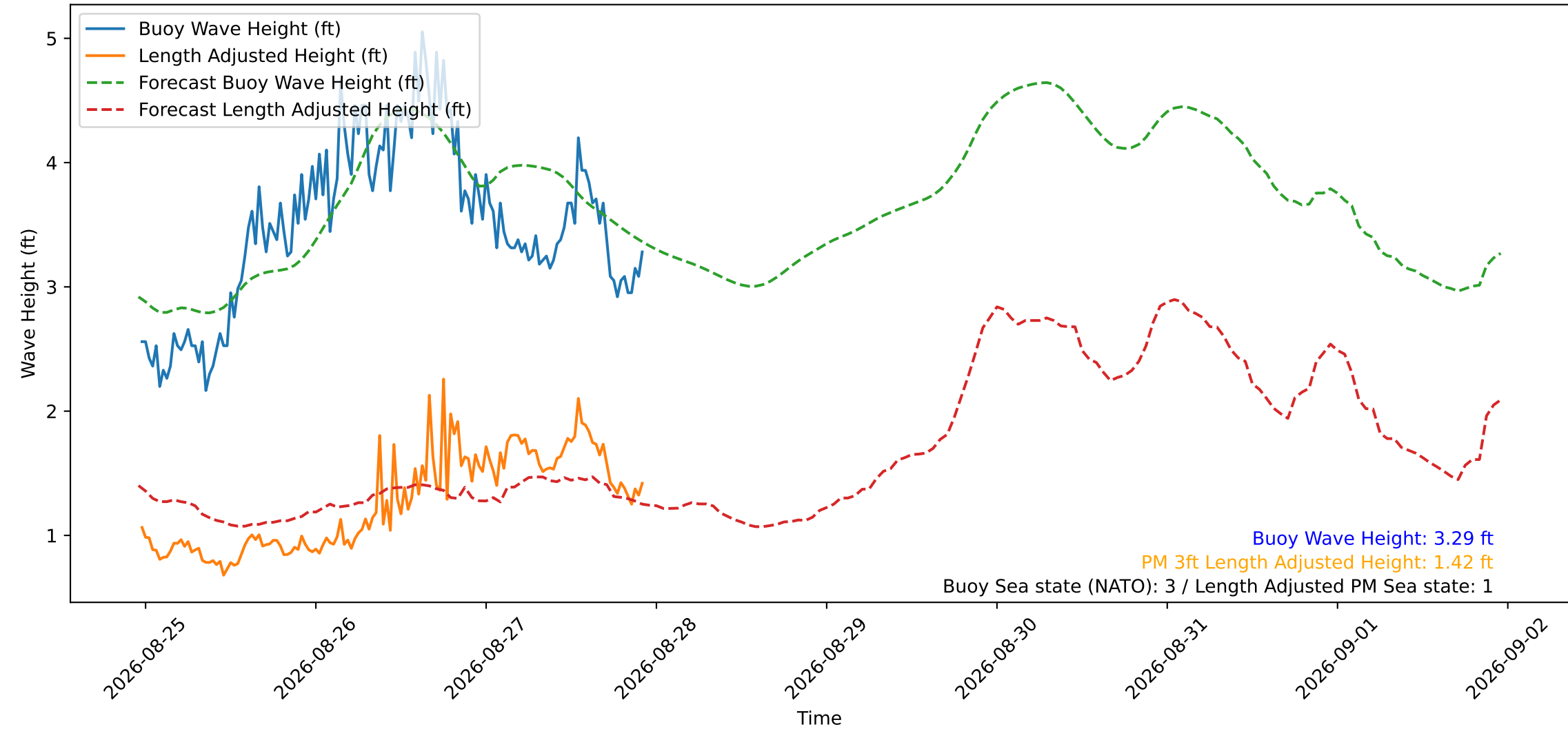
Wave Heights over Time for Red Beach at 2026-08-27 23:00:50
