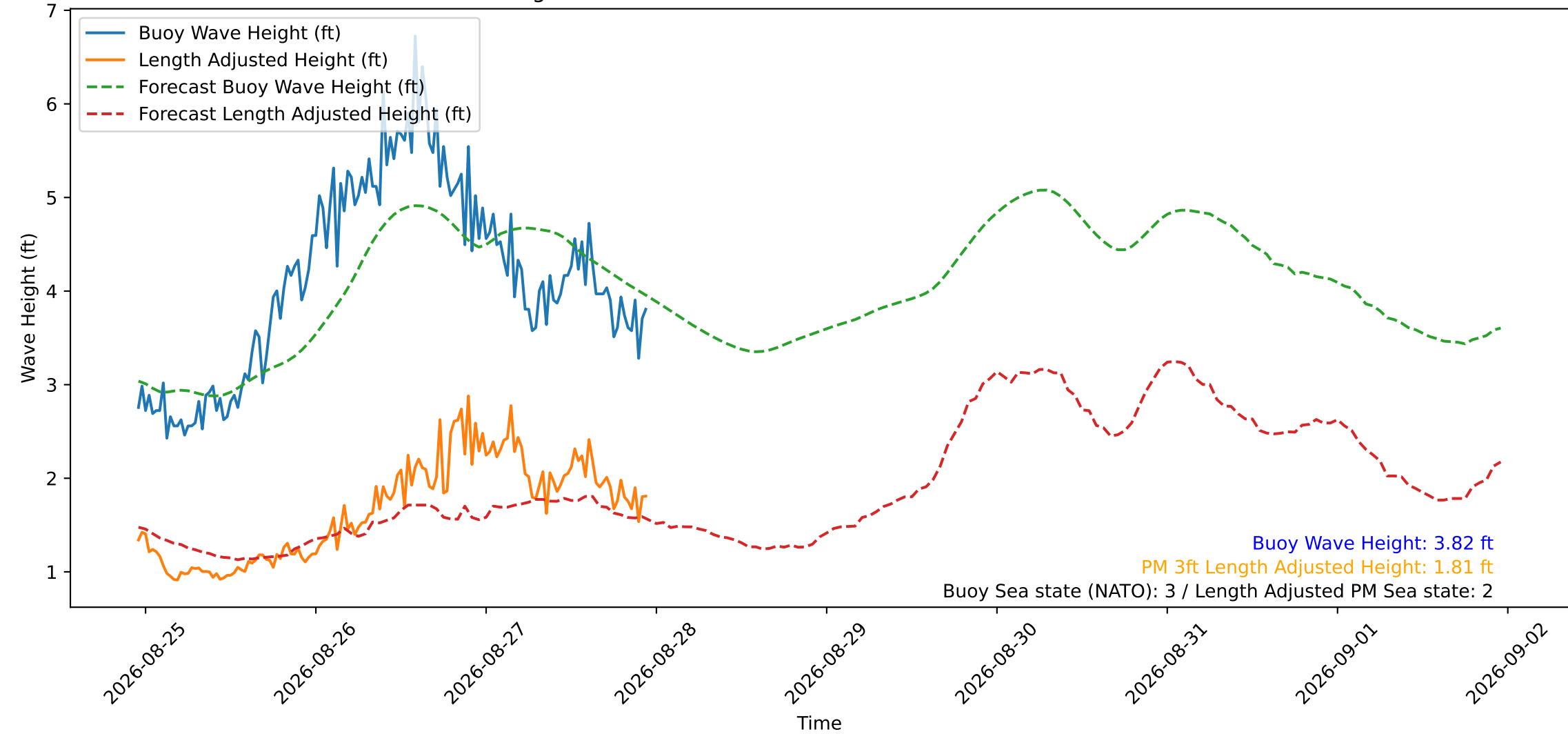
Wave Heights over Time for Oceanside Harbor at 2026-08-27 23:00:30
