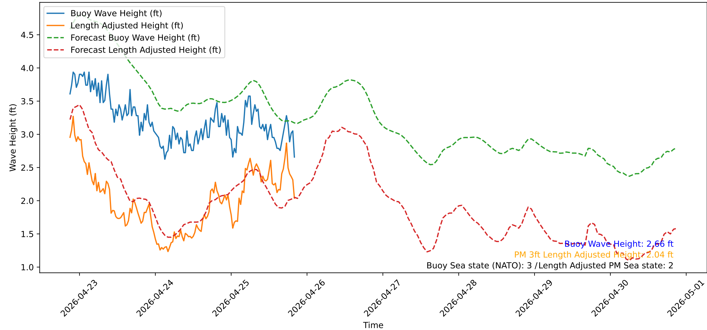
Wave Heights over Time for Green Beach at 2026-04-25 20:51:14
