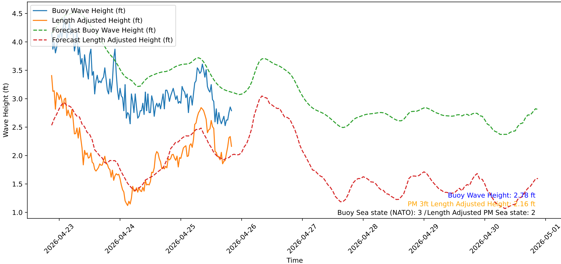
Wave Heights over Time for Oceanside Harbor at 2026-04-25 20:50:31
