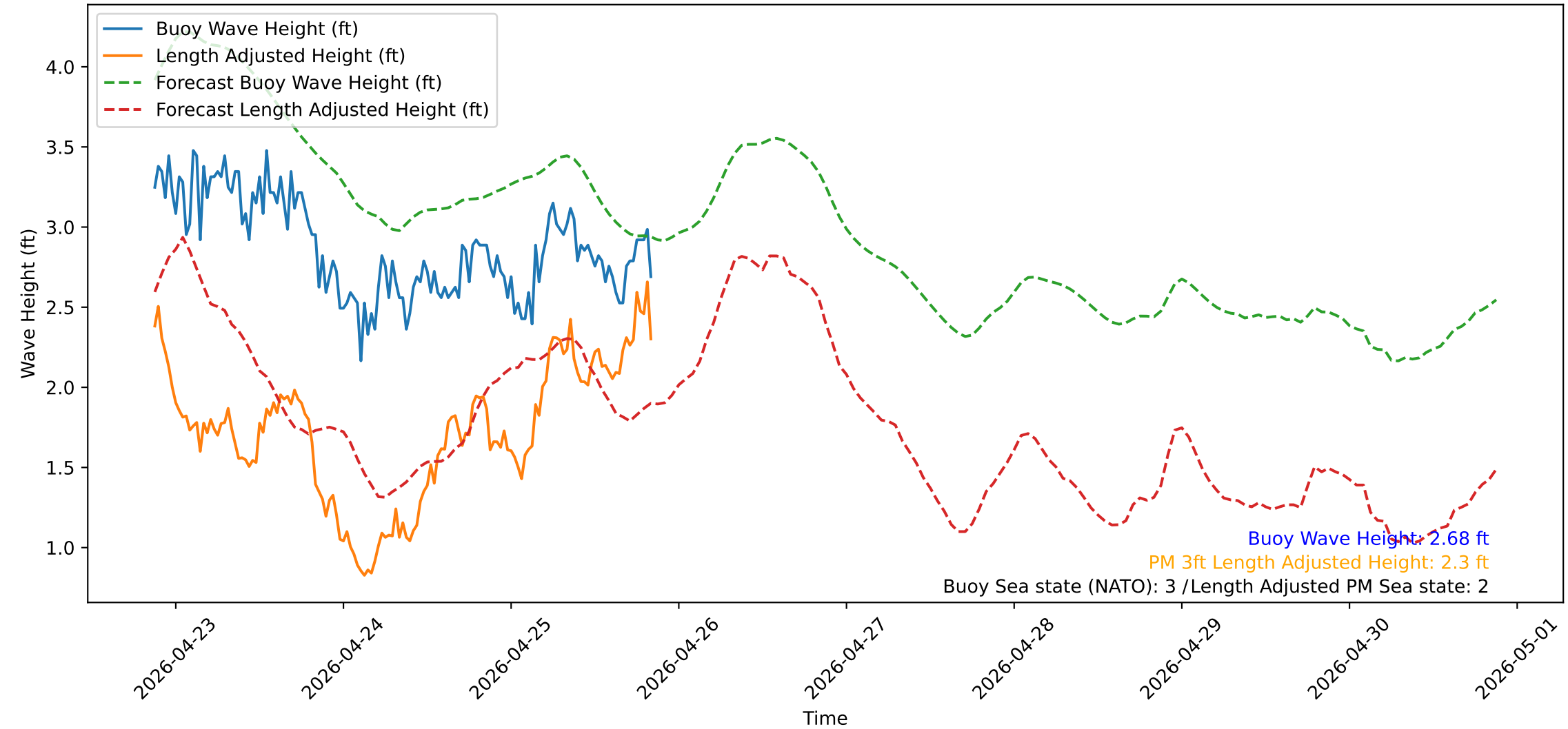
Wave Heights over Time for Red Beach at 2026-04-25 20:50:52
