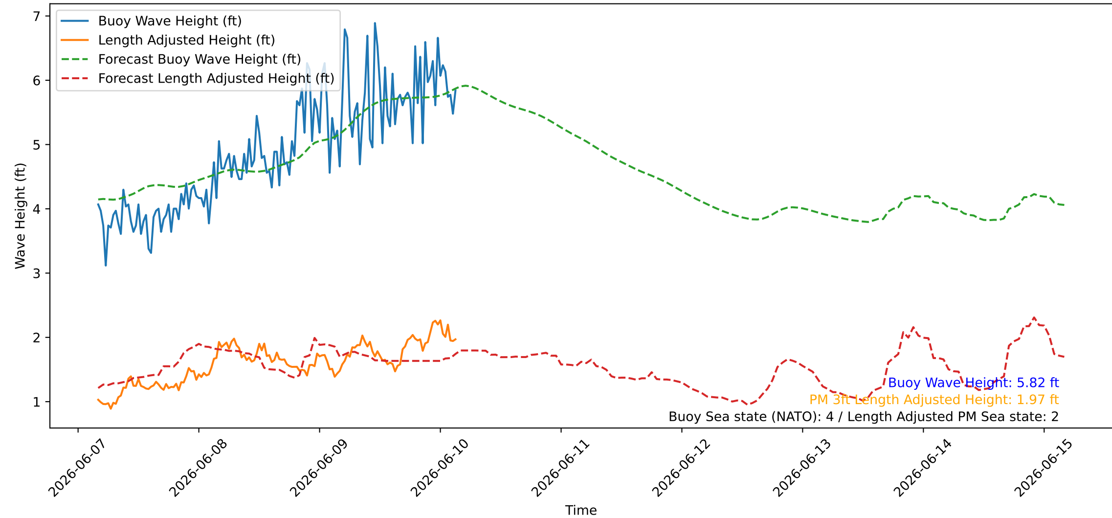
Wave Heights over Time for Green Beach at 2026-06-10 03:51:11
