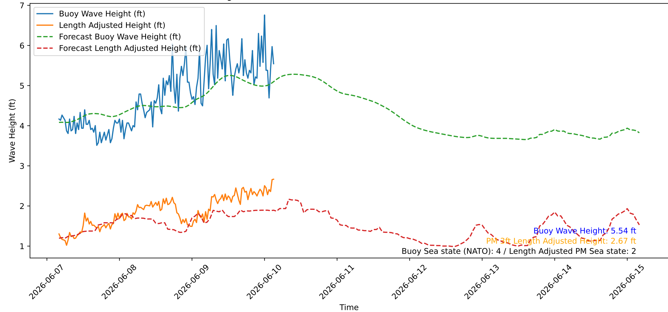
Wave Heights over Time for Oceanside Harbor at 2026-06-10 03:50:26
