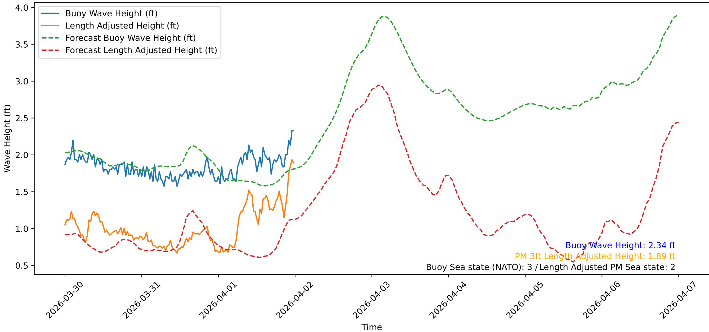
Wave Heights over Time for Oceanside Harbor at 2026-04-02 00:00:31
