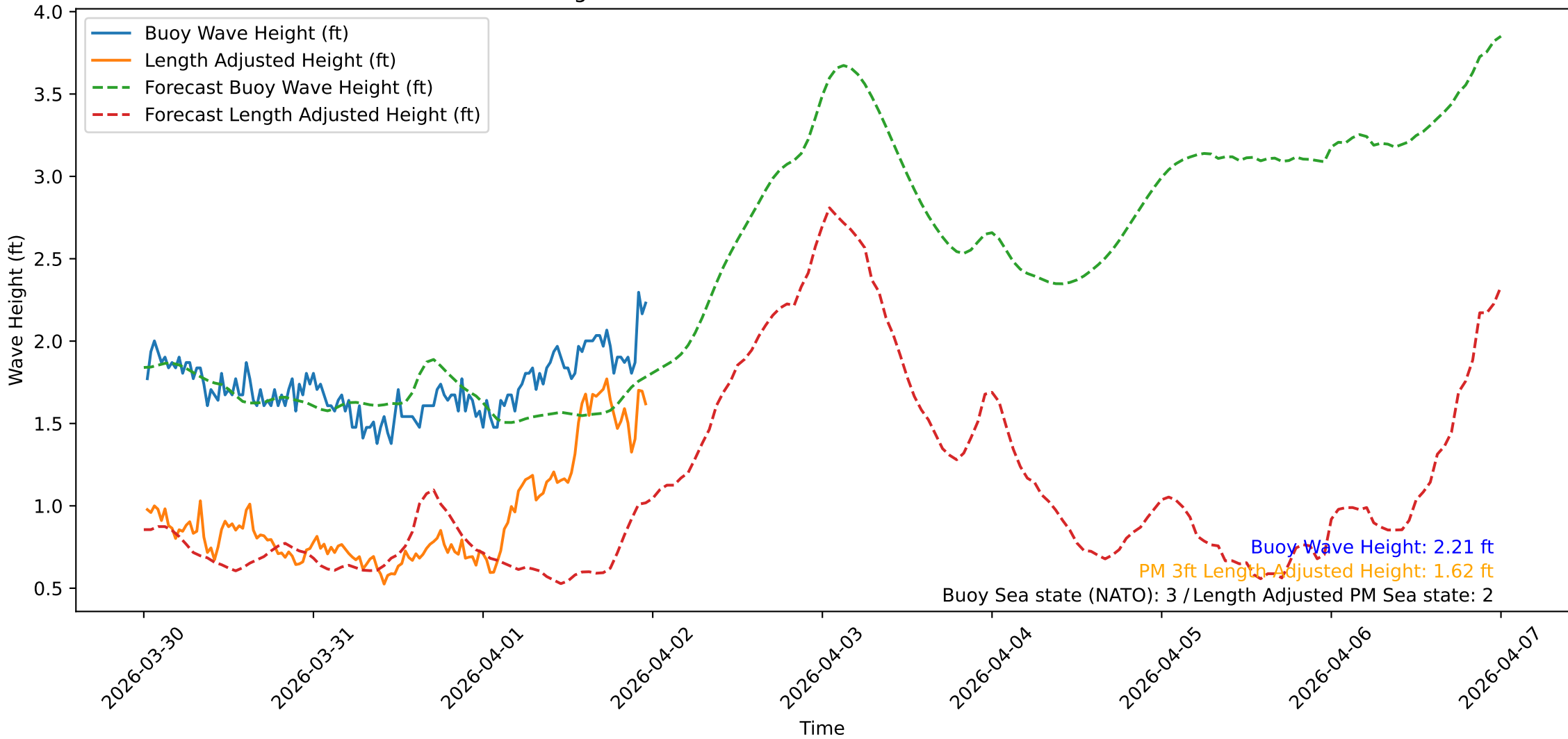
Wave Heights over Time for Red Beach at 2026-04-02 00:00:47
