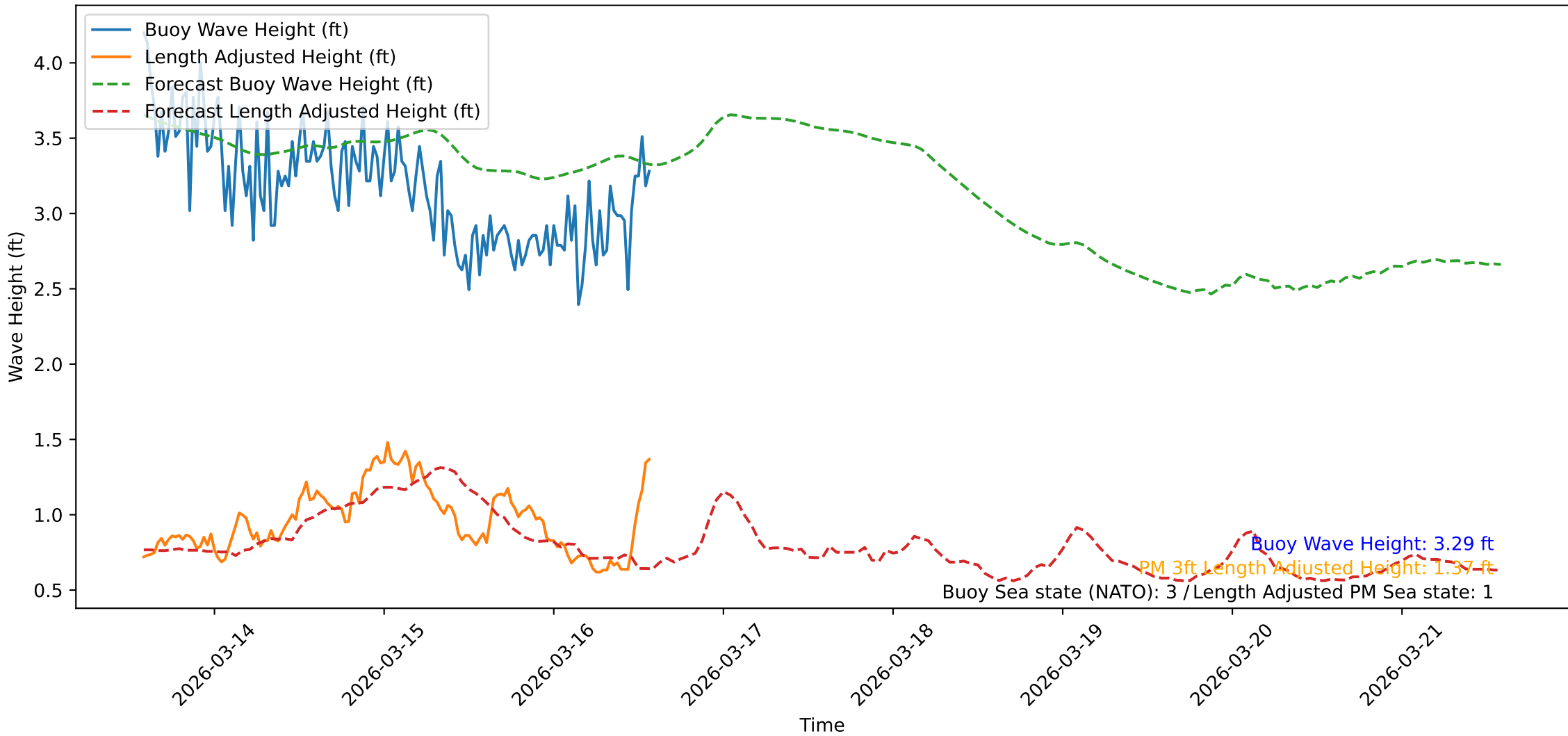
Wave Heights over Time for Oceanside Harbor at 2026-03-16 14:10:43
