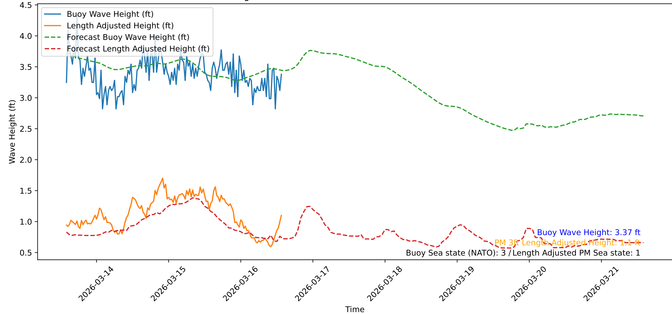
Wave Heights over Time for Green Beach at 2026-03-16 14:11:38
