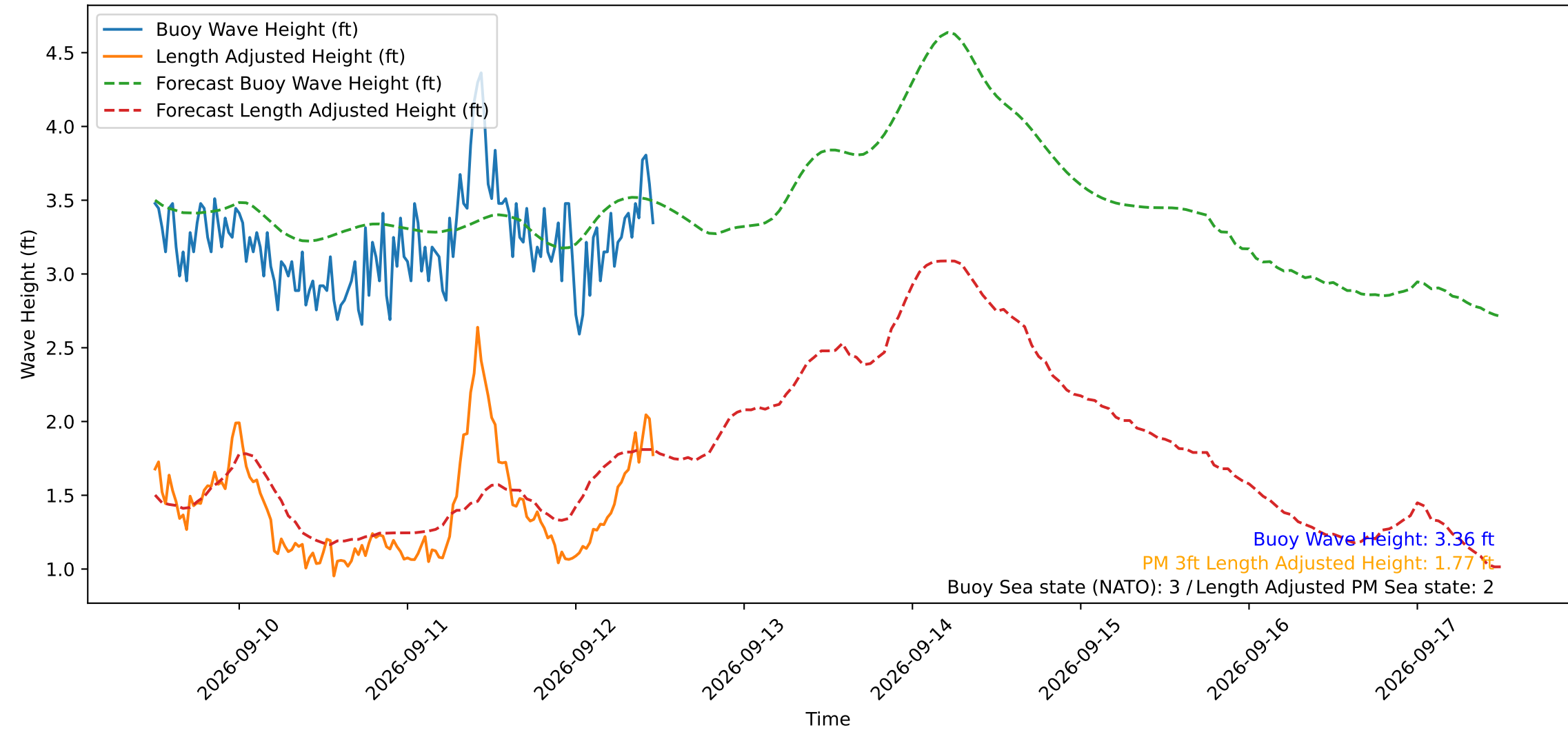
Wave Heights over Time for Oceanside Harbor at 2026-09-12 12:00:29
