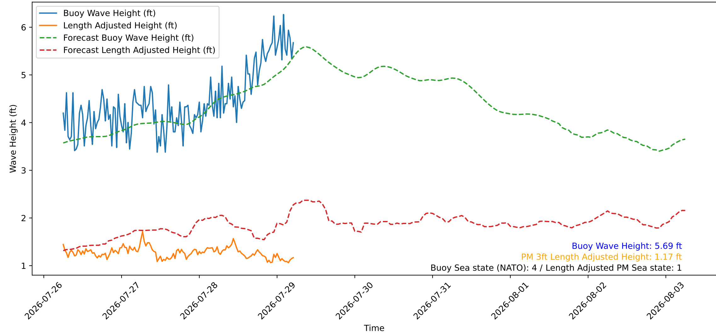
Wave Heights over Time for Green Beach at 2026-07-29 06:01:08
