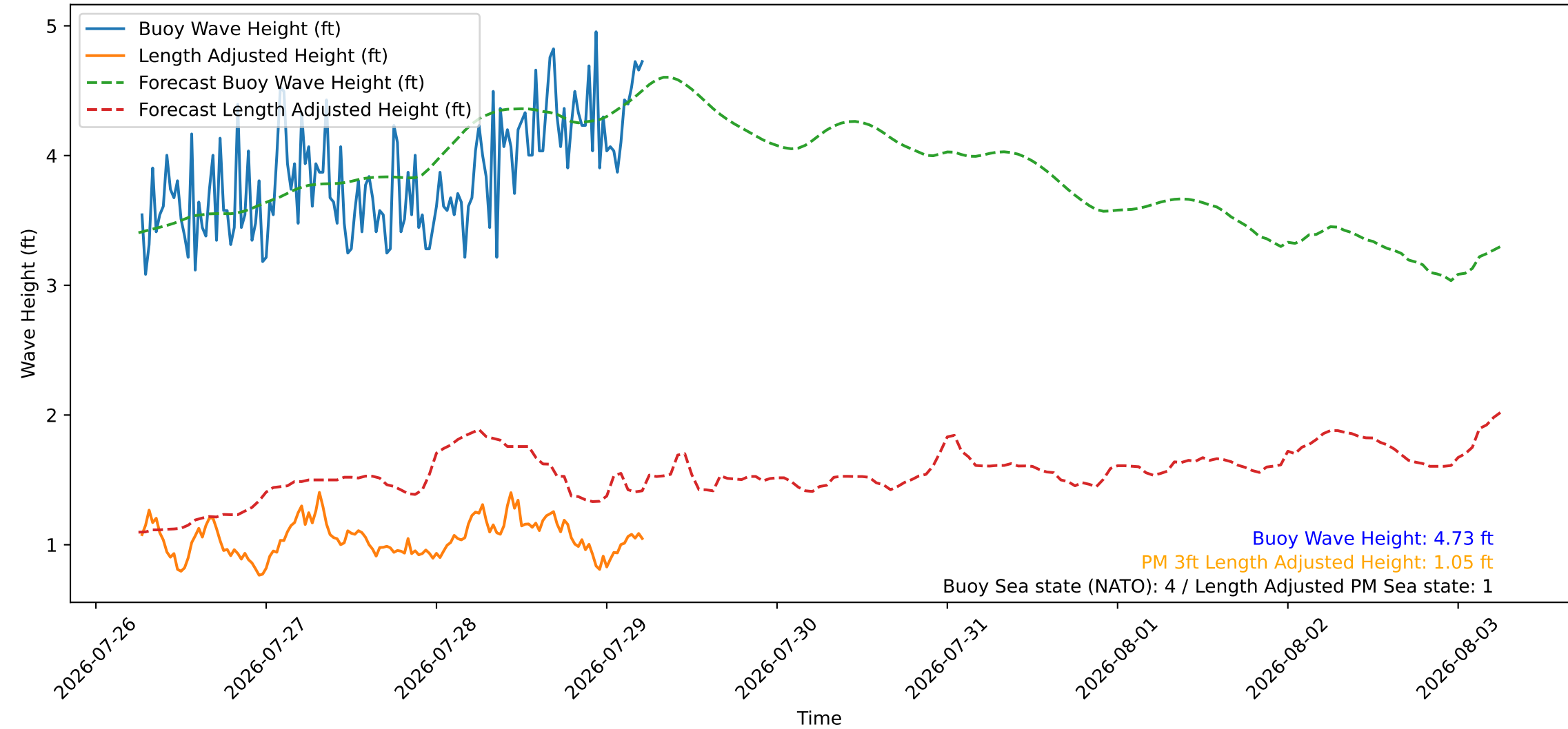
Wave Heights over Time for Red Beach at 2026-07-29 06:00:45
