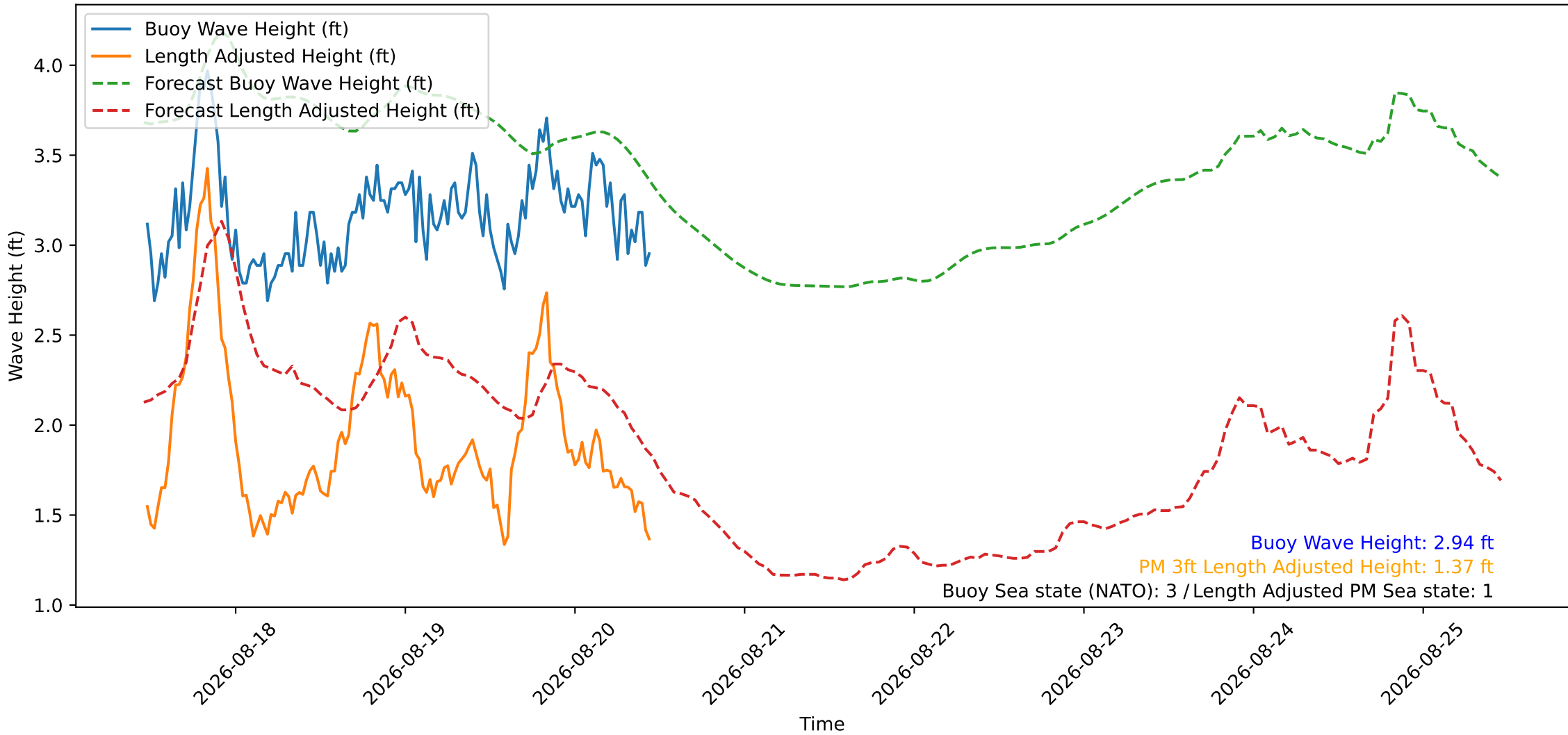
Wave Heights over Time for Green Beach at 2026-08-20 11:11:09
