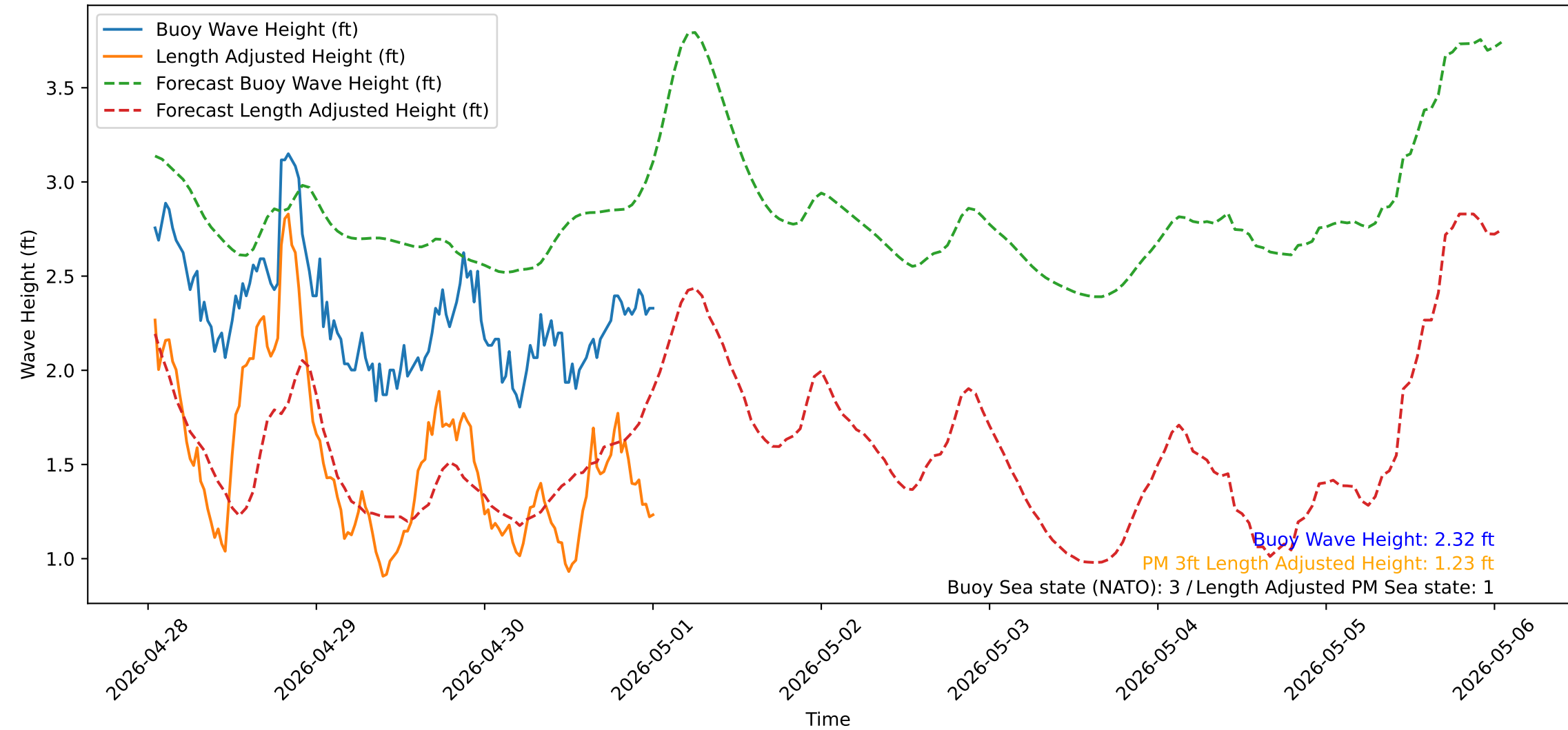
Wave Heights over Time for Green Beach at 2026-05-01 01:01:13
