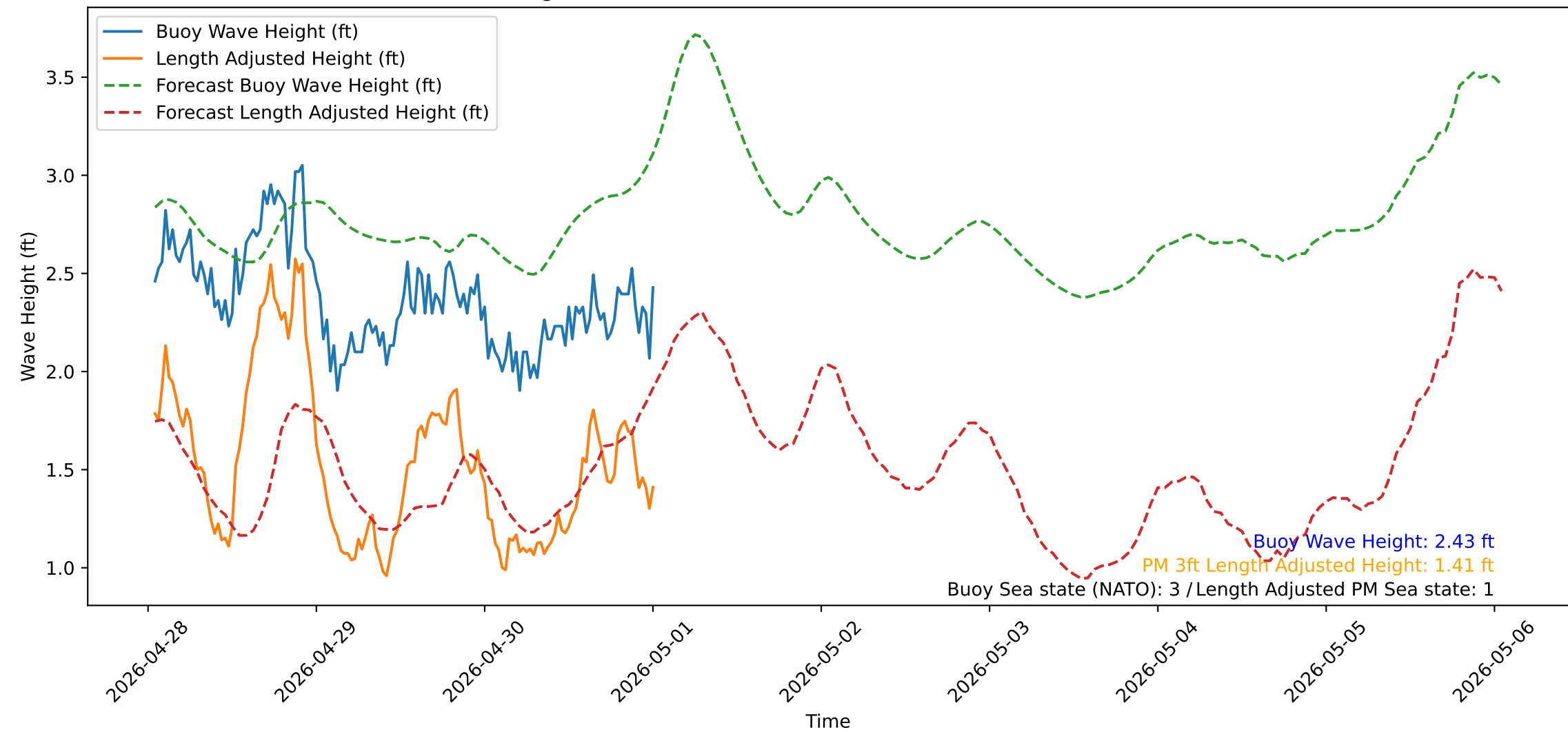
Wave Heights over Time for Oceanside Harbor at 2026-05-01 01:00:32
