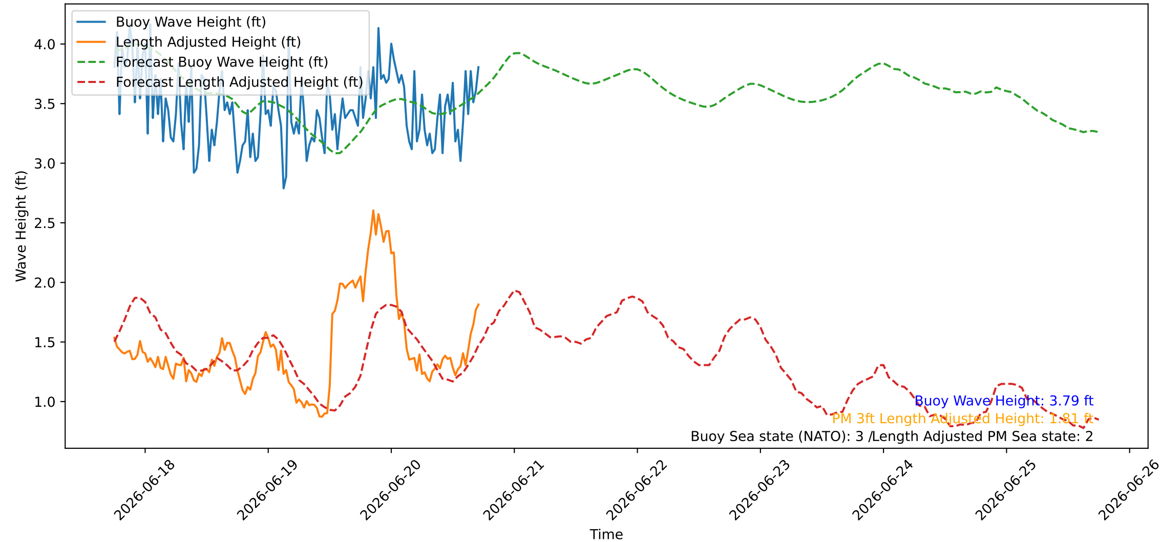
Wave Heights over Time for Oceanside Harbor at 2026-06-20 17:50:26
