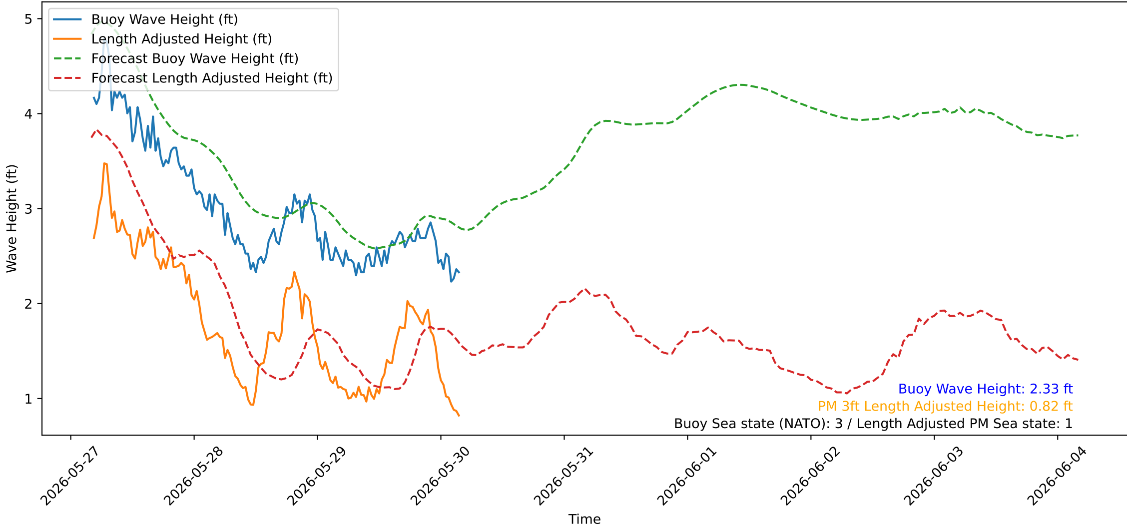
Wave Heights over Time for Red Beach at 2026-05-30 04:20:43
