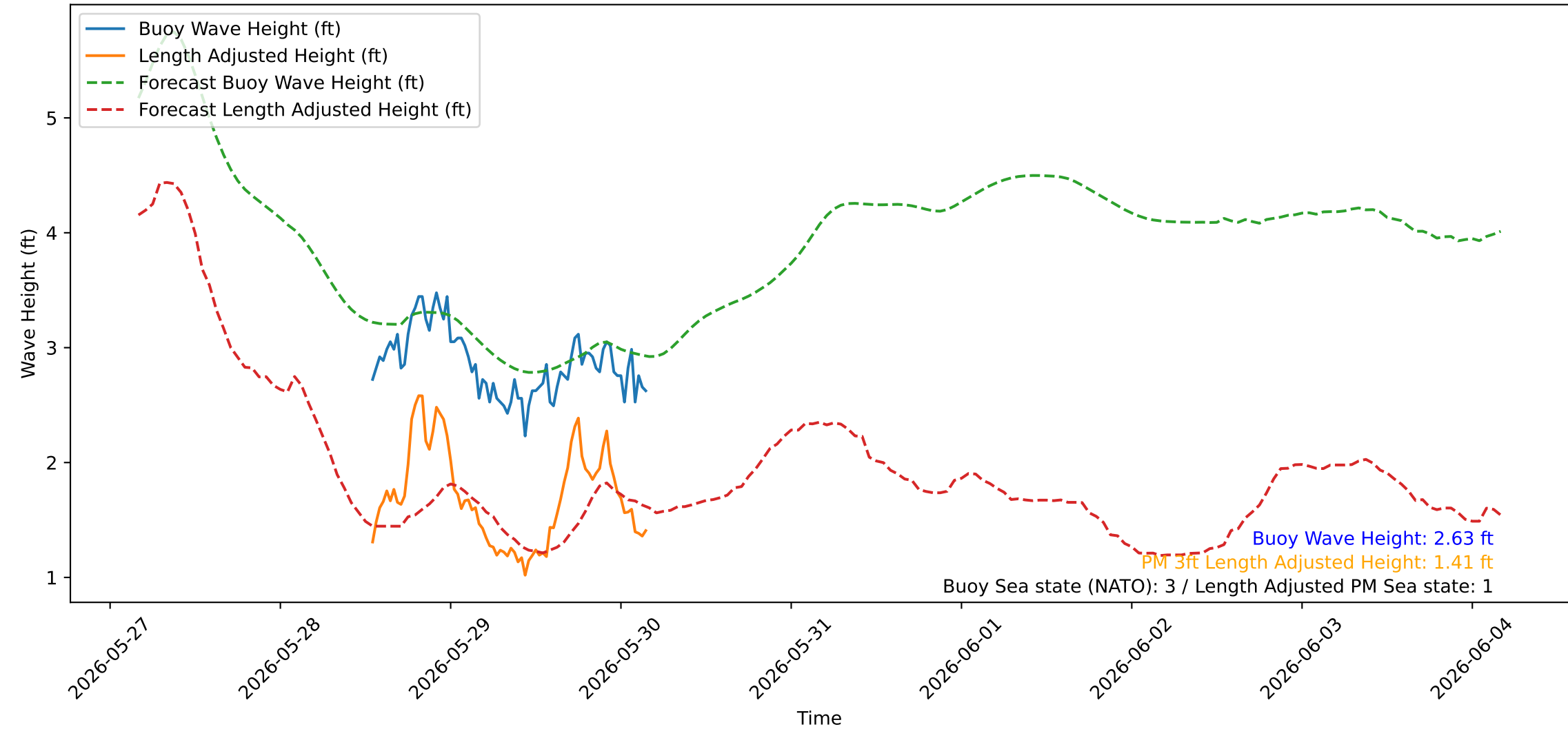
Wave Heights over Time for Oceanside Harbor at 2026-05-30 04:20:22
