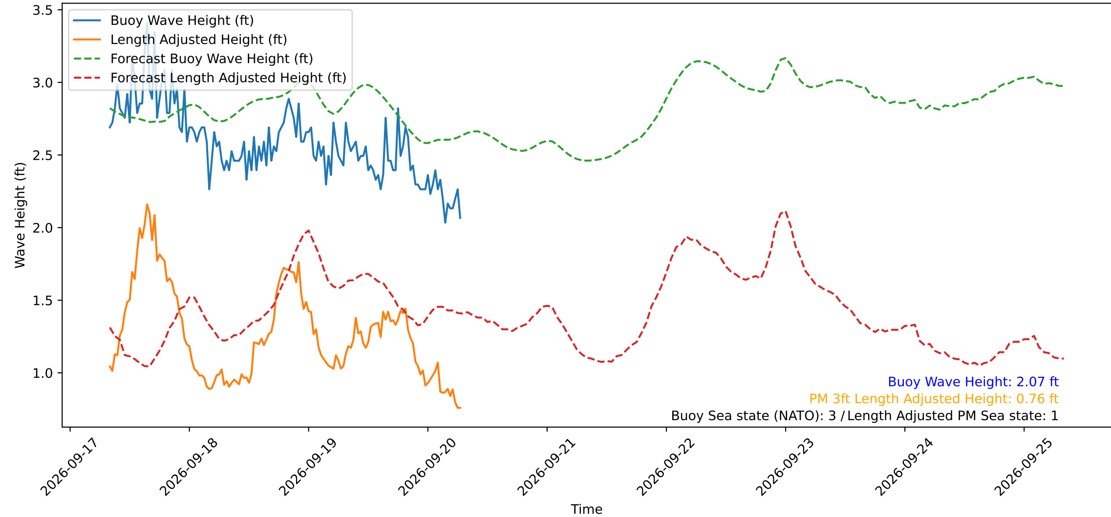
Wave Heights over Time for Red Beach at 2026-09-20 07:30:49
