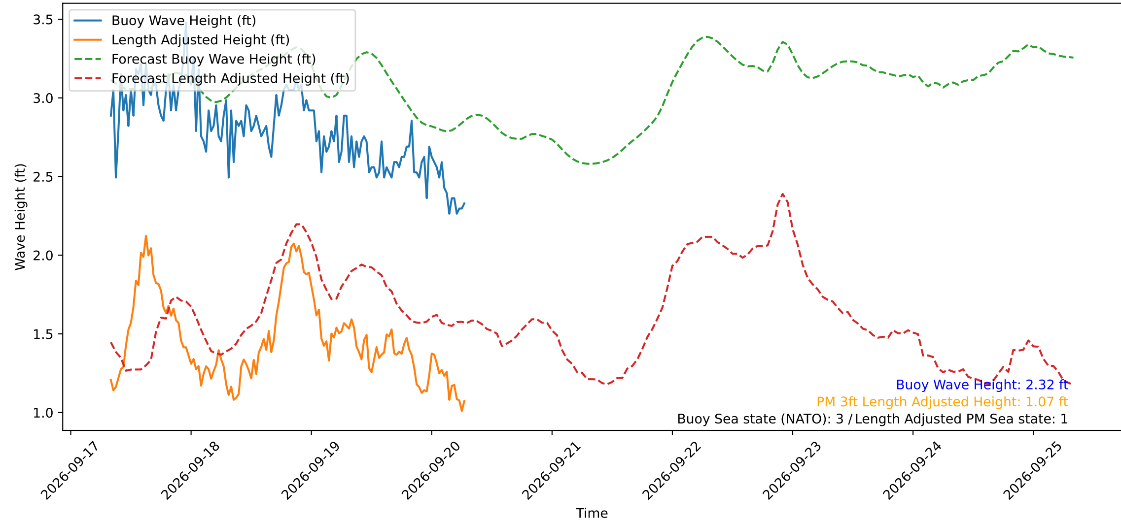
Wave Heights over Time for Green Beach at 2026-09-20 07:31:11
