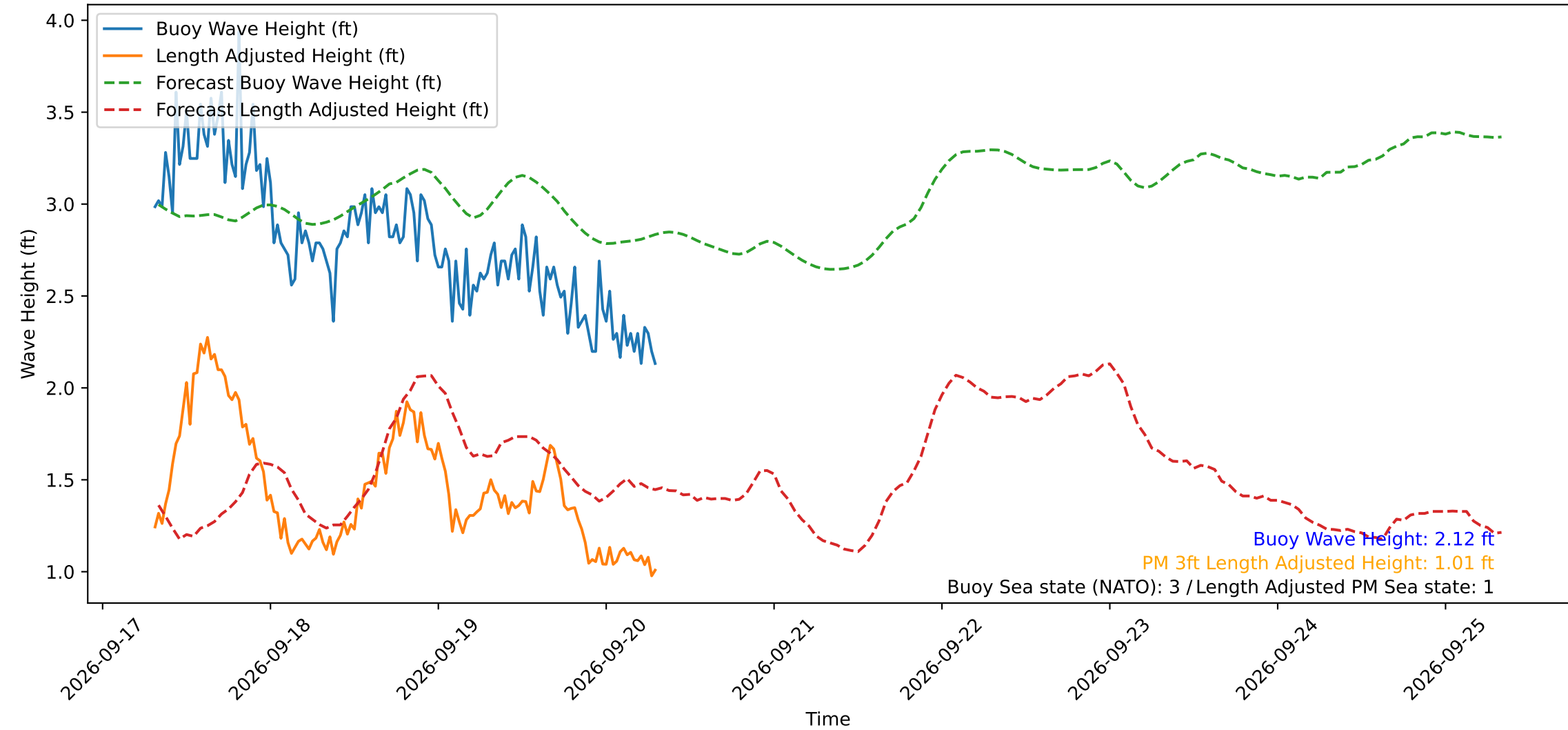
Wave Heights over Time for Oceanside Harbor at 2026-09-20 07:30:30
