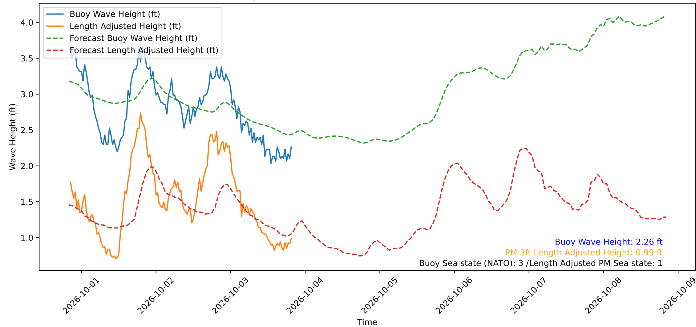
Wave Heights over Time for Green Beach at 2026-10-03 20:21:15
