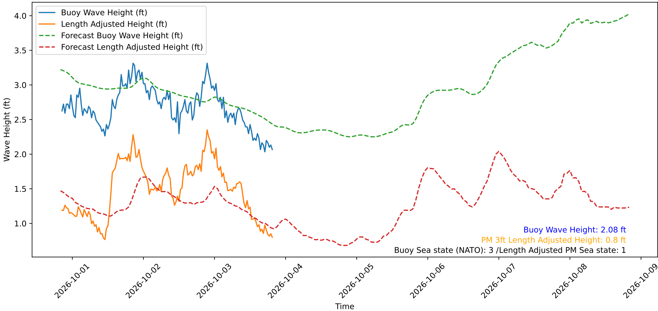
Wave Heights over Time for Oceanside Harbor at 2026-10-03 20:20:30
