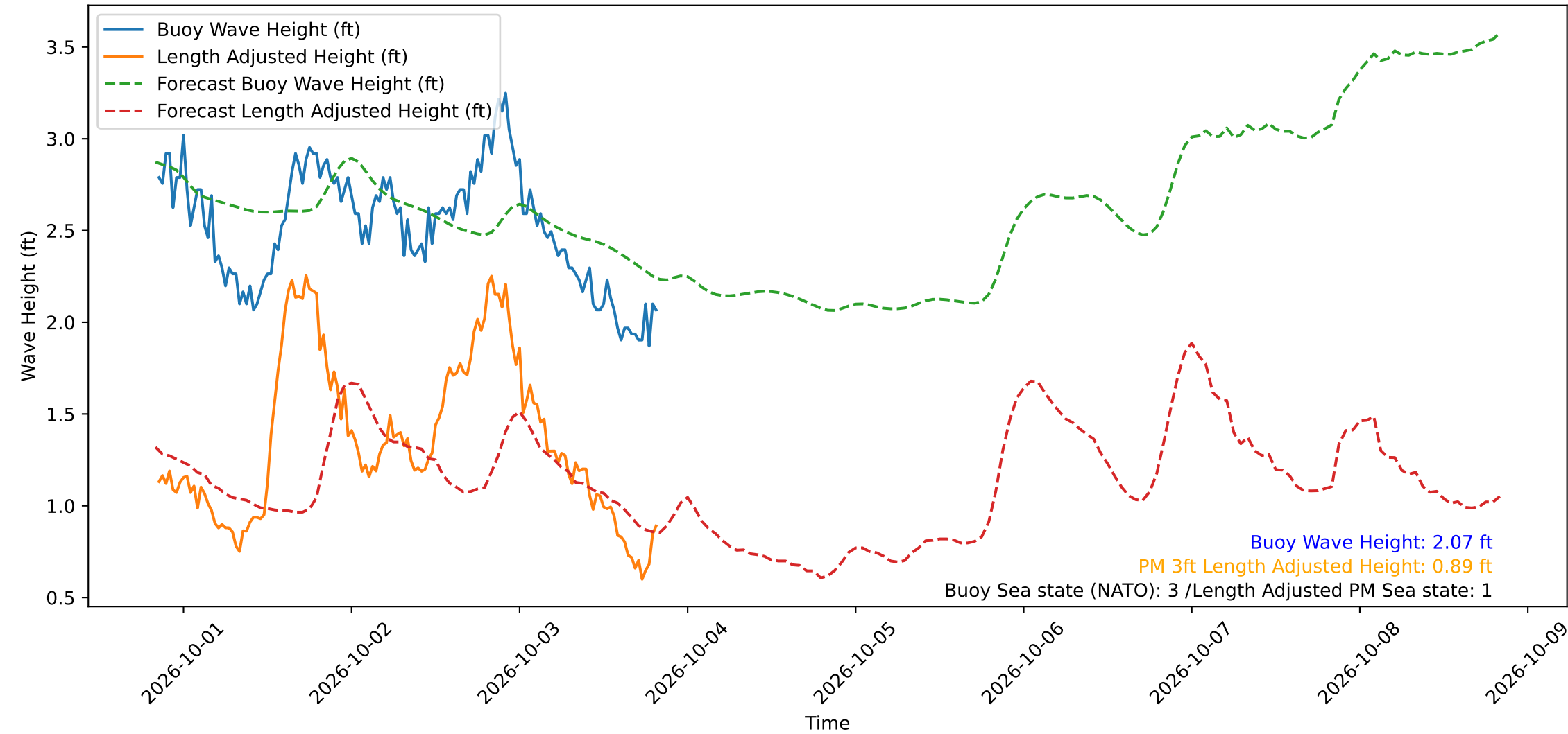
Wave Heights over Time for Red Beach at 2026-10-03 20:20:51
