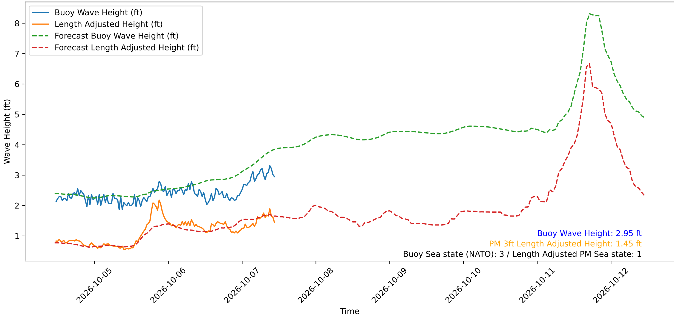
Wave Heights over Time for Oceanside Harbor at 2026-10-07 11:20:29
