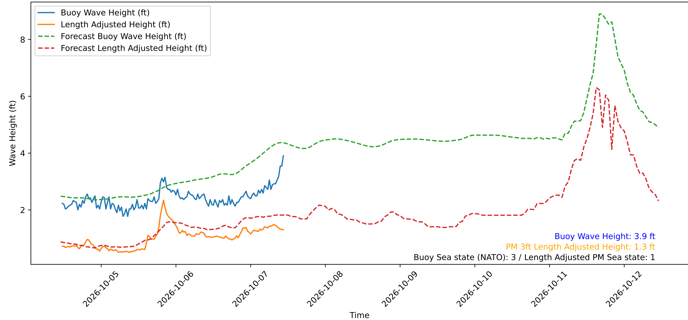
Wave Heights over Time for Green Beach at 2026-10-07 11:21:16
