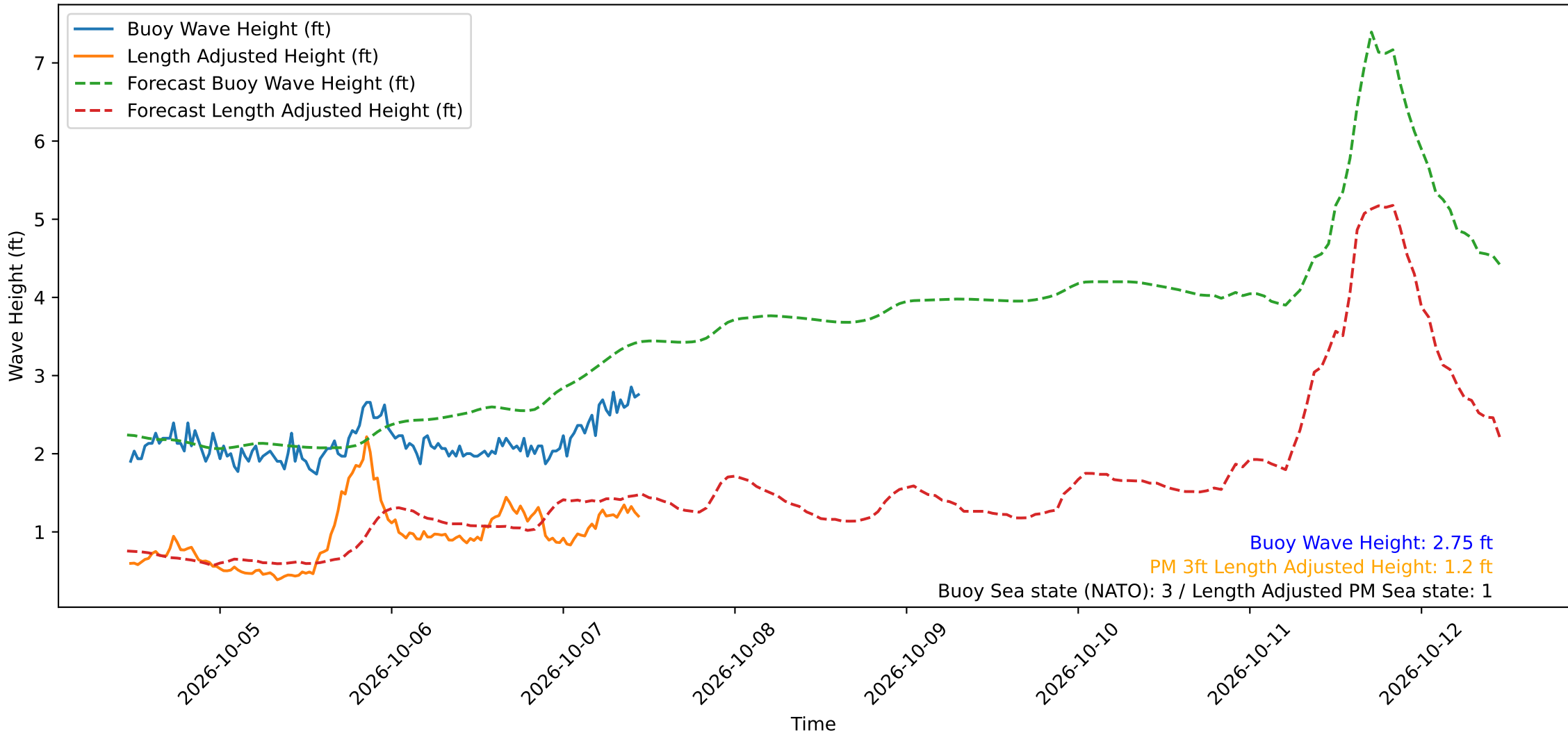
Wave Heights over Time for Red Beach at 2026-10-07 11:20:52
