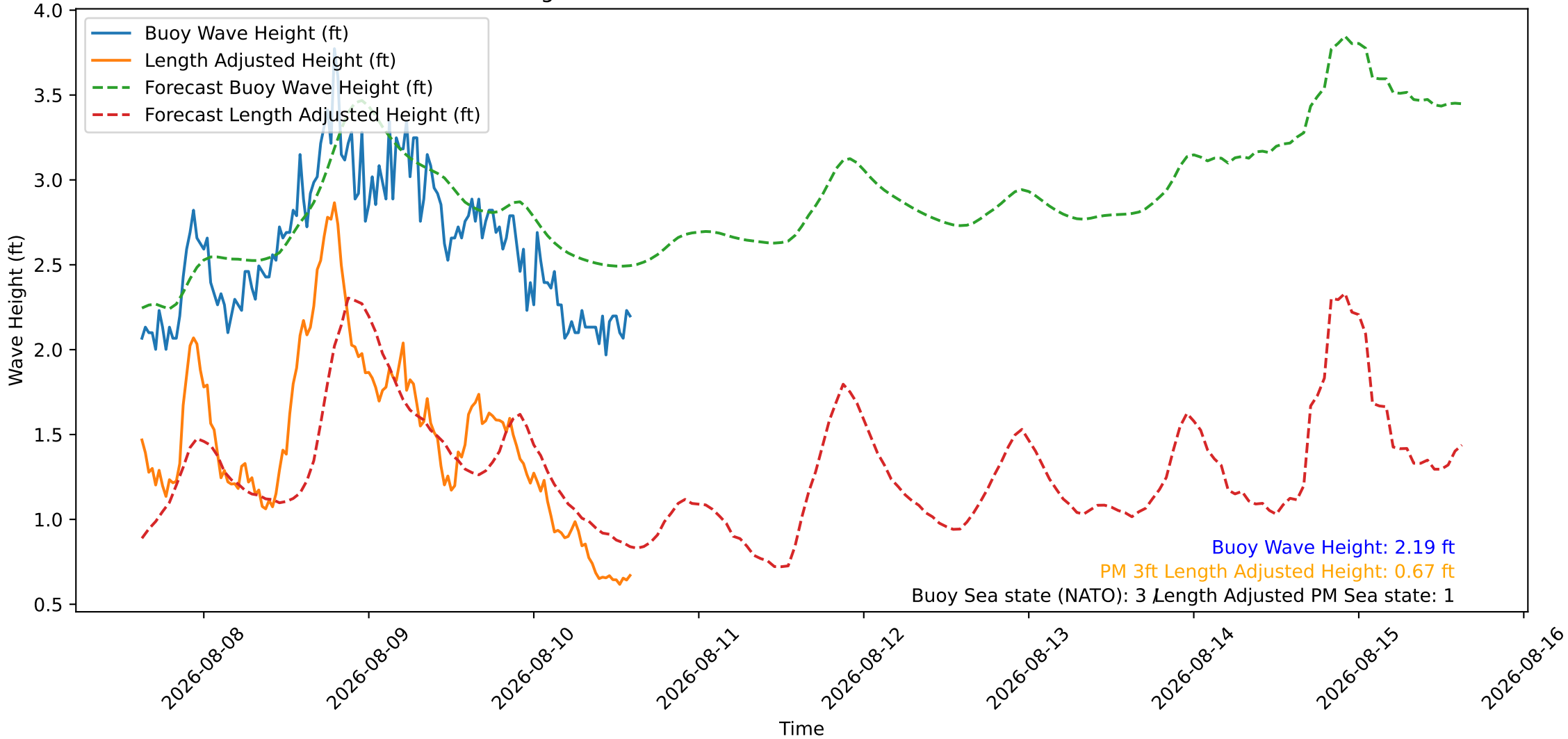
Wave Heights over Time for Green Beach at 2026-08-10 14:51:10
