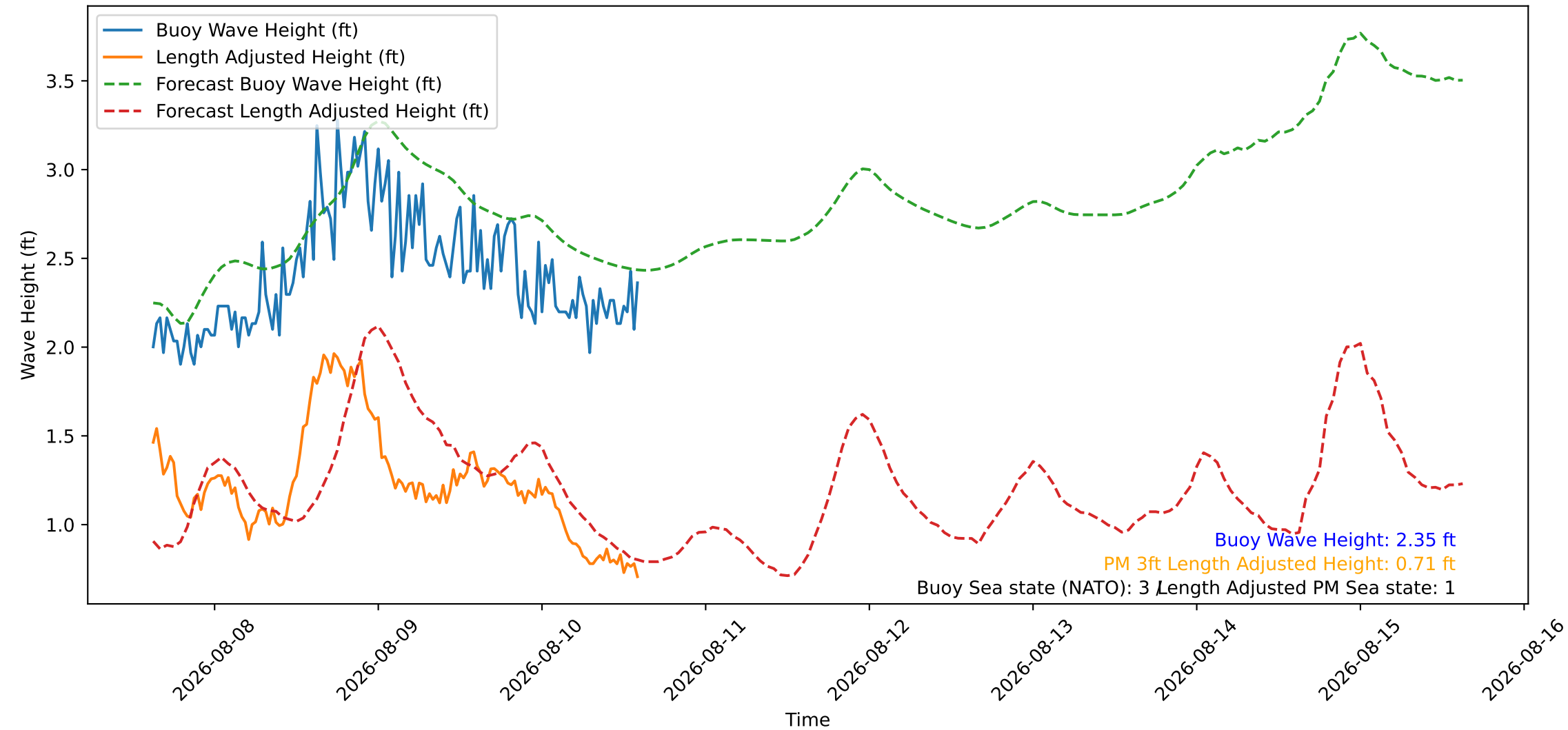
Wave Heights over Time for Oceanside Harbor at 2026-08-10 14:50:27
