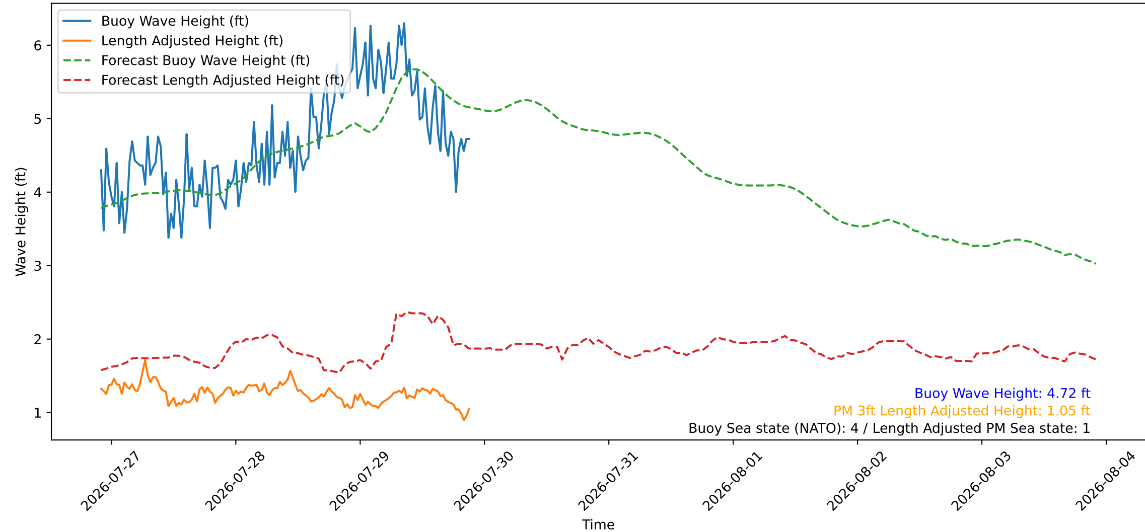
Wave Heights over Time for Green Beach at 2026-07-29 22:01:08
