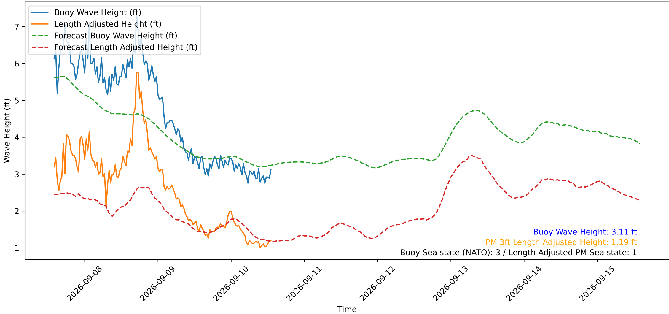
Wave Heights over Time for Oceanside Harbor at 2026-09-10 14:00:29
