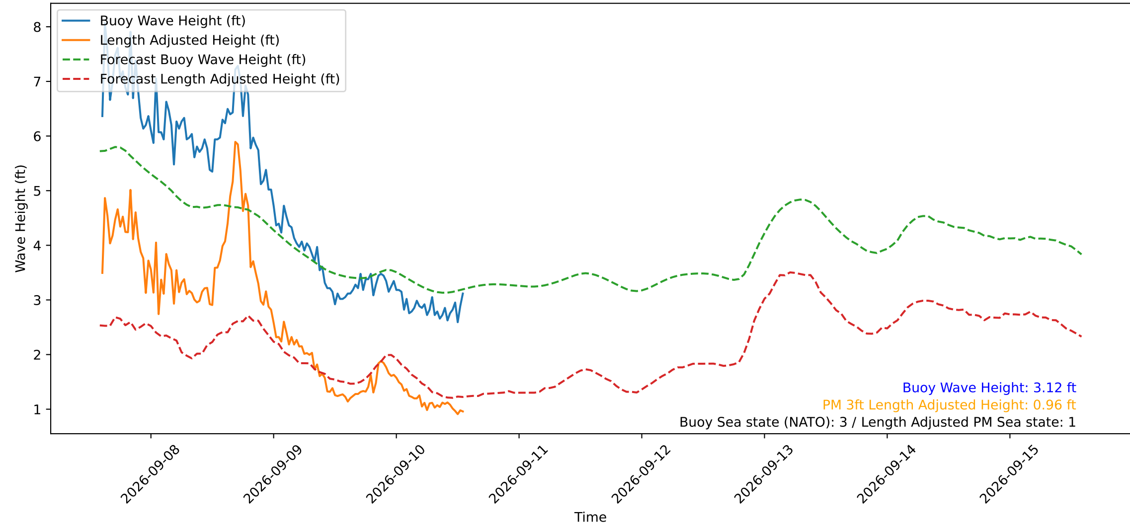
Wave Heights over Time for Green Beach at 2026-09-10 14:01:12
