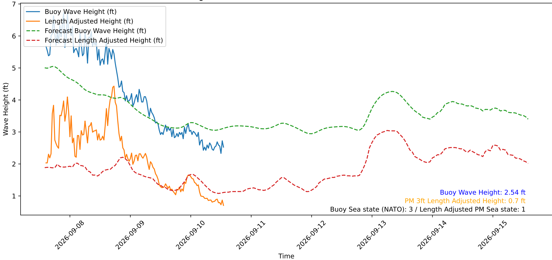
Wave Heights over Time for Red Beach at 2026-09-10 14:00:49
