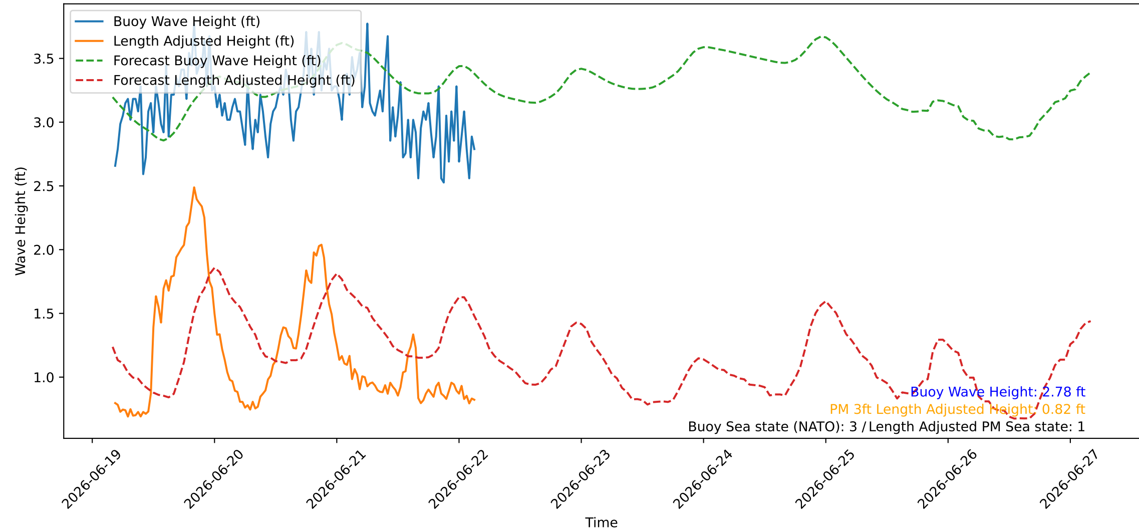
Wave Heights over Time for Red Beach at 2026-06-22 04:00:45
