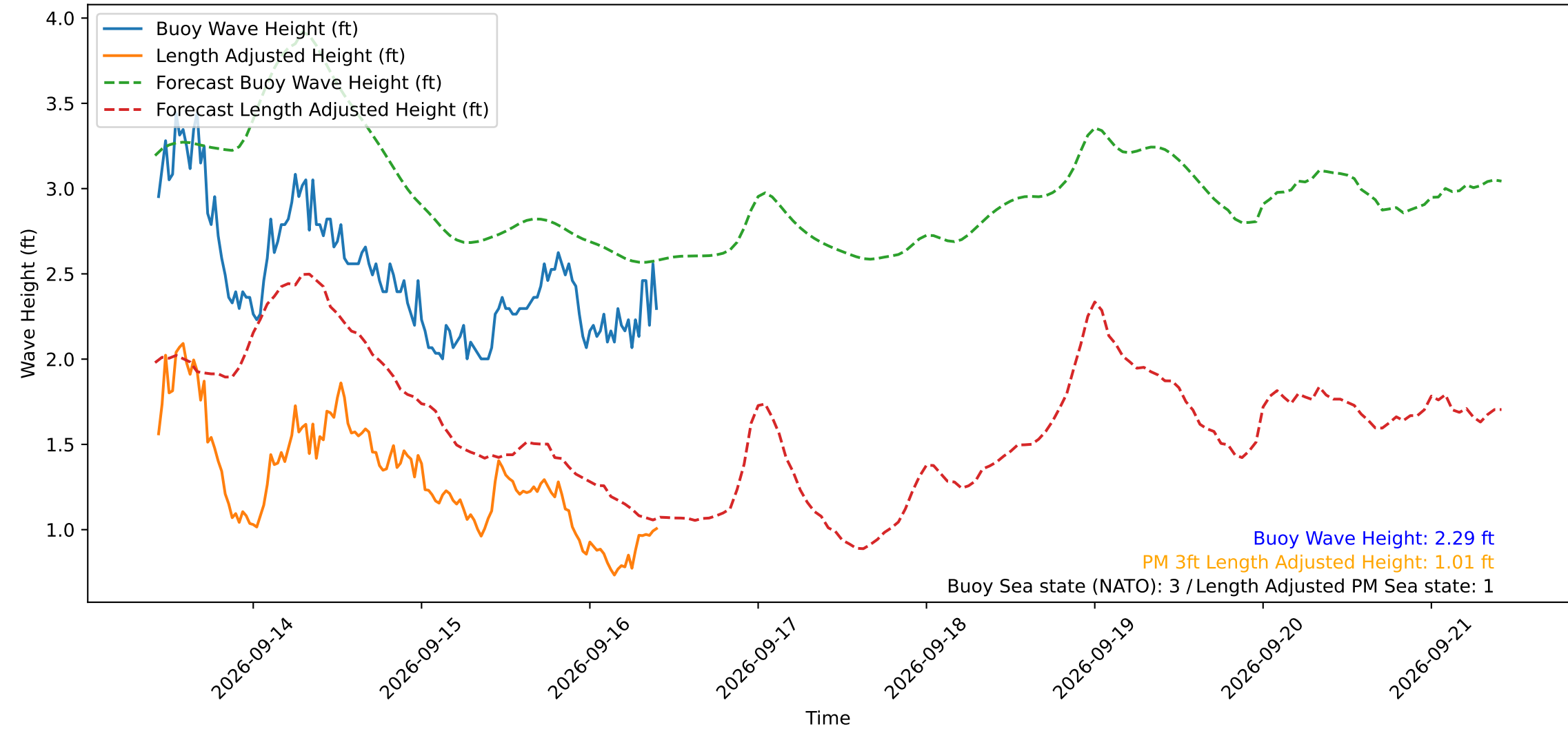
Wave Heights over Time for Red Beach at 2026-09-16 10:20:50
