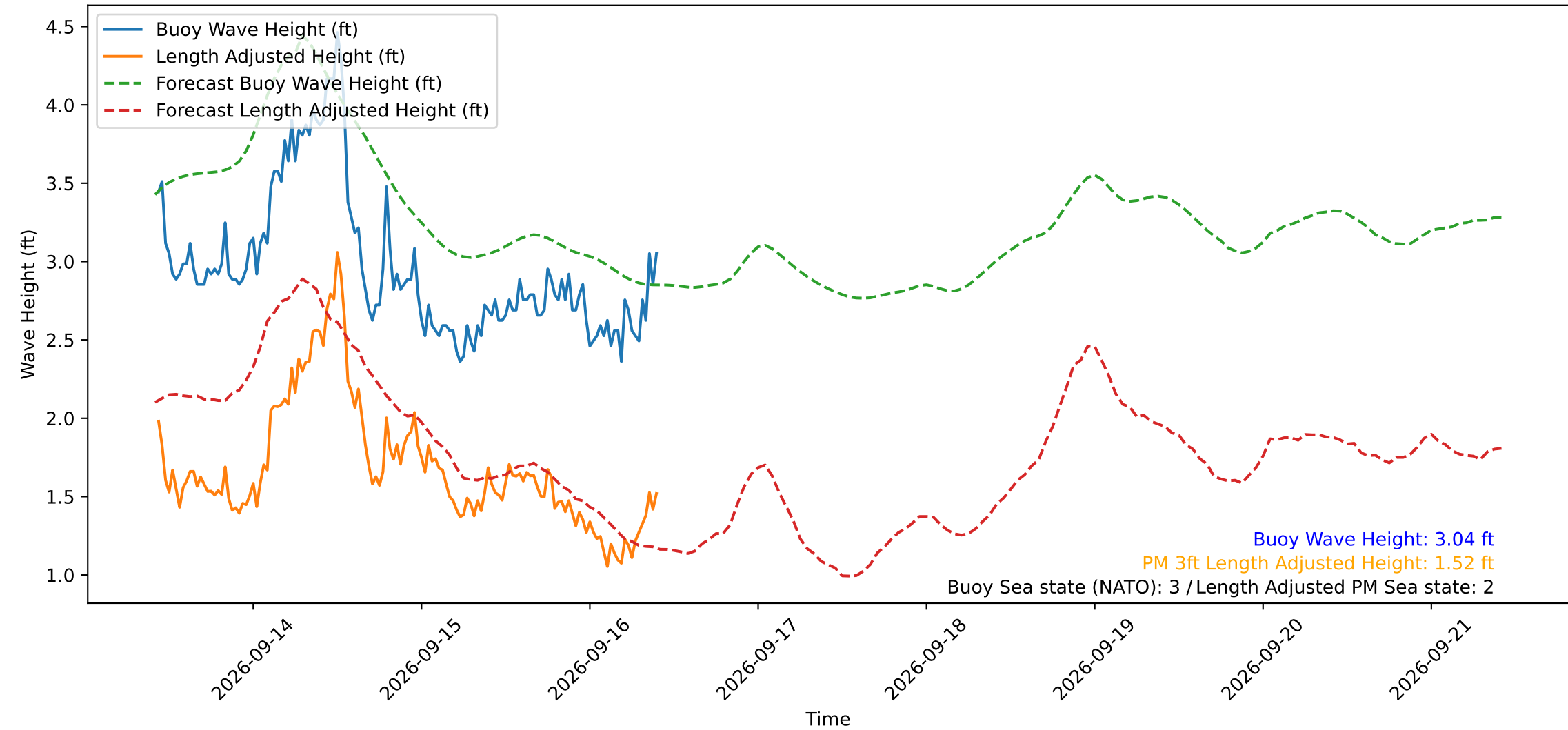
Wave Heights over Time for Oceanside Harbor at 2026-09-16 10:20:30
