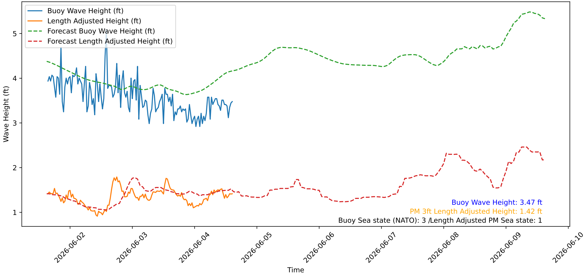
Wave Heights over Time for Oceanside Harbor at 2026-06-04 15:20:25
