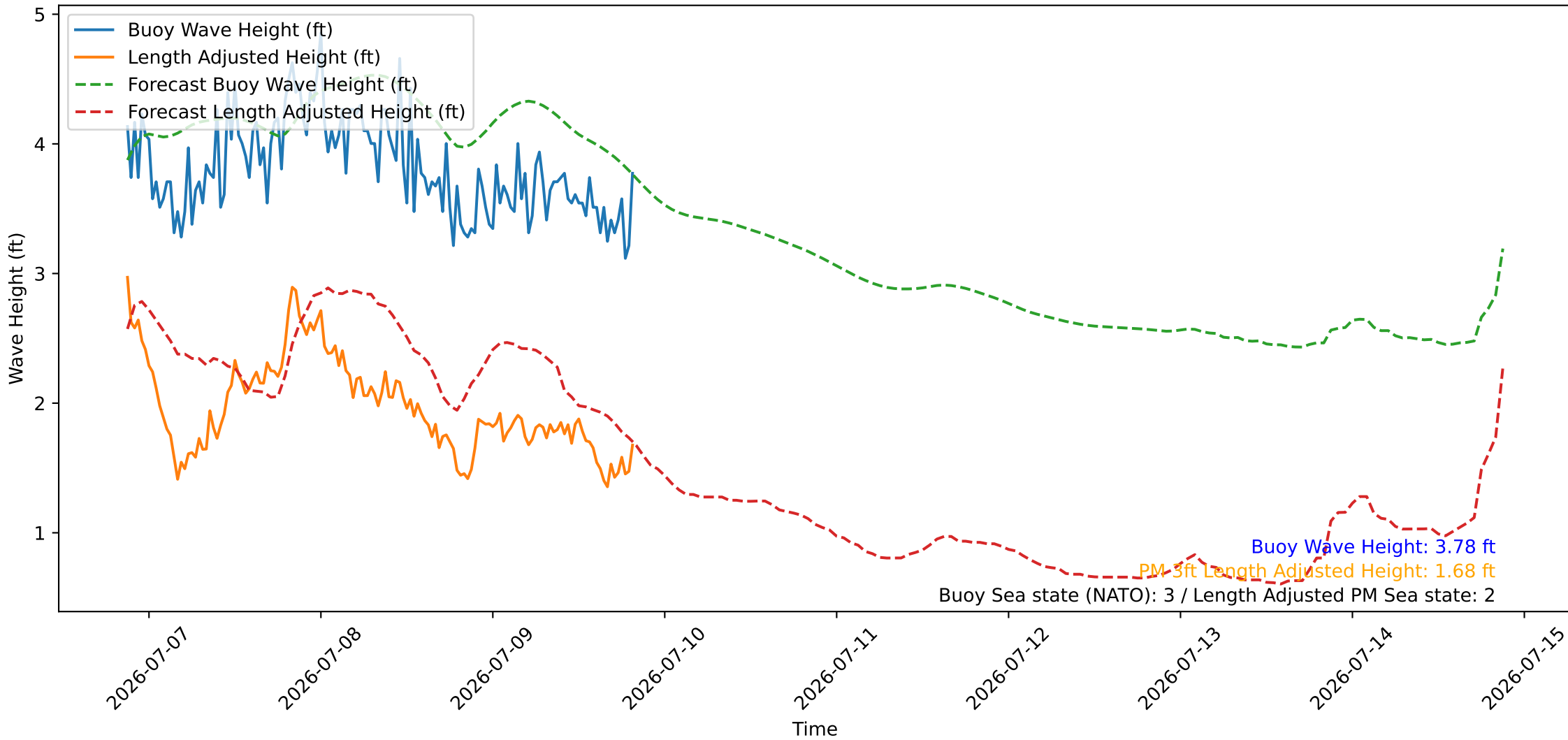
Wave Heights over Time for Red Beach at 2026-07-09 20:30:46
