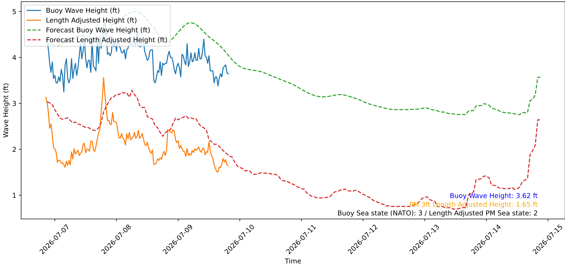
Wave Heights over Time for Green Beach at 2026-07-09 20:31:08
