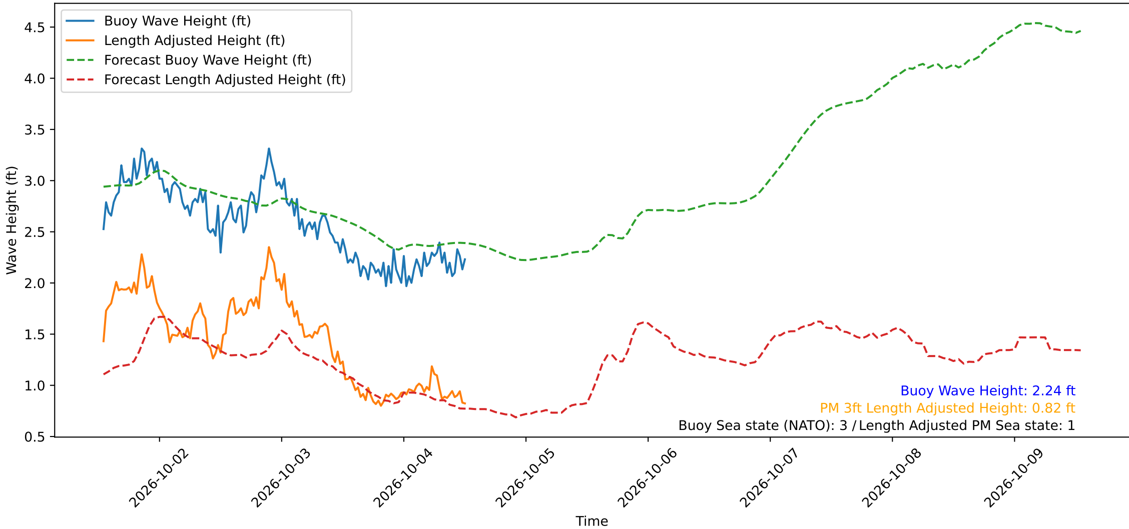
Wave Heights over Time for Oceanside Harbor at 2026-10-04 13:00:30
