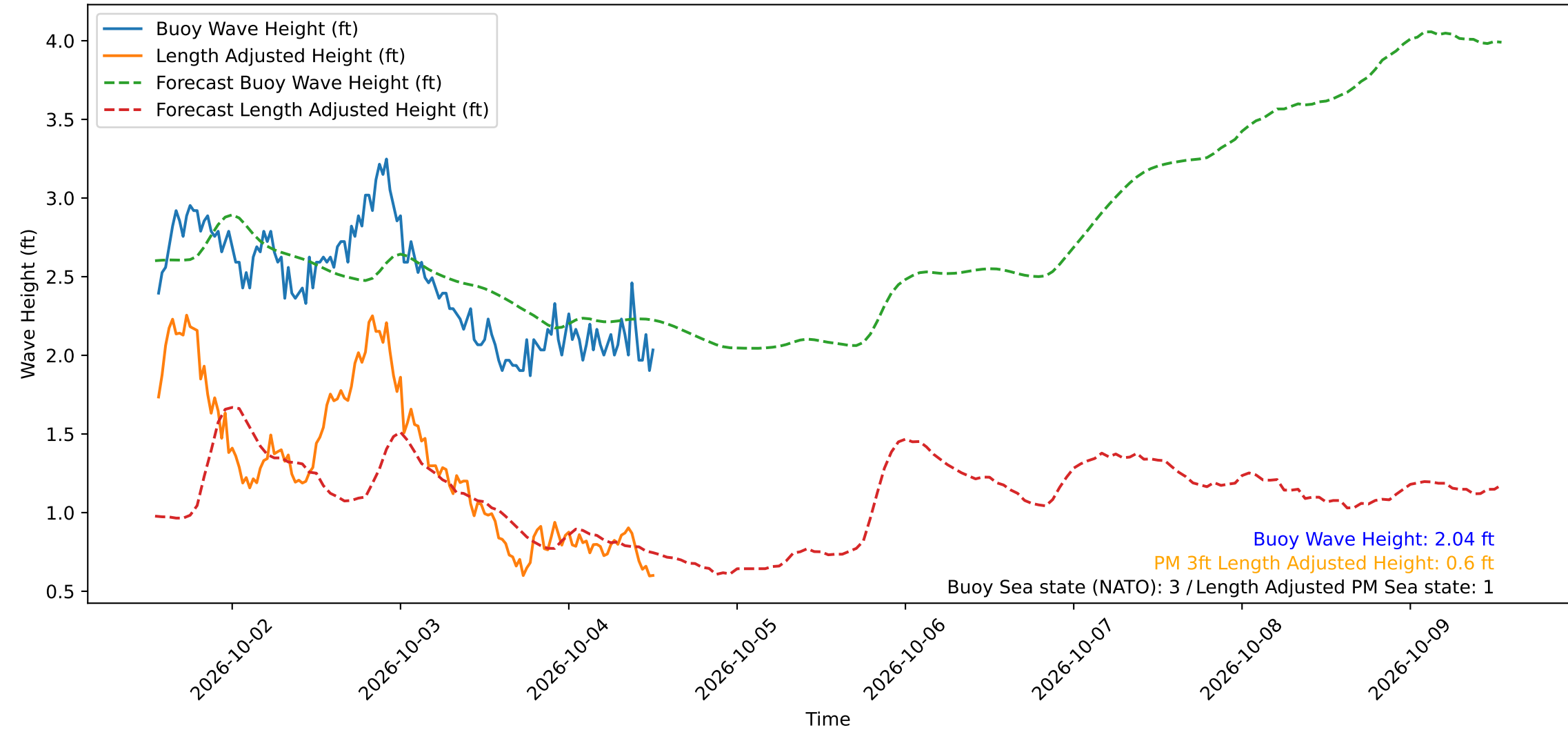
Wave Heights over Time for Red Beach at 2026-10-04 13:00:49
