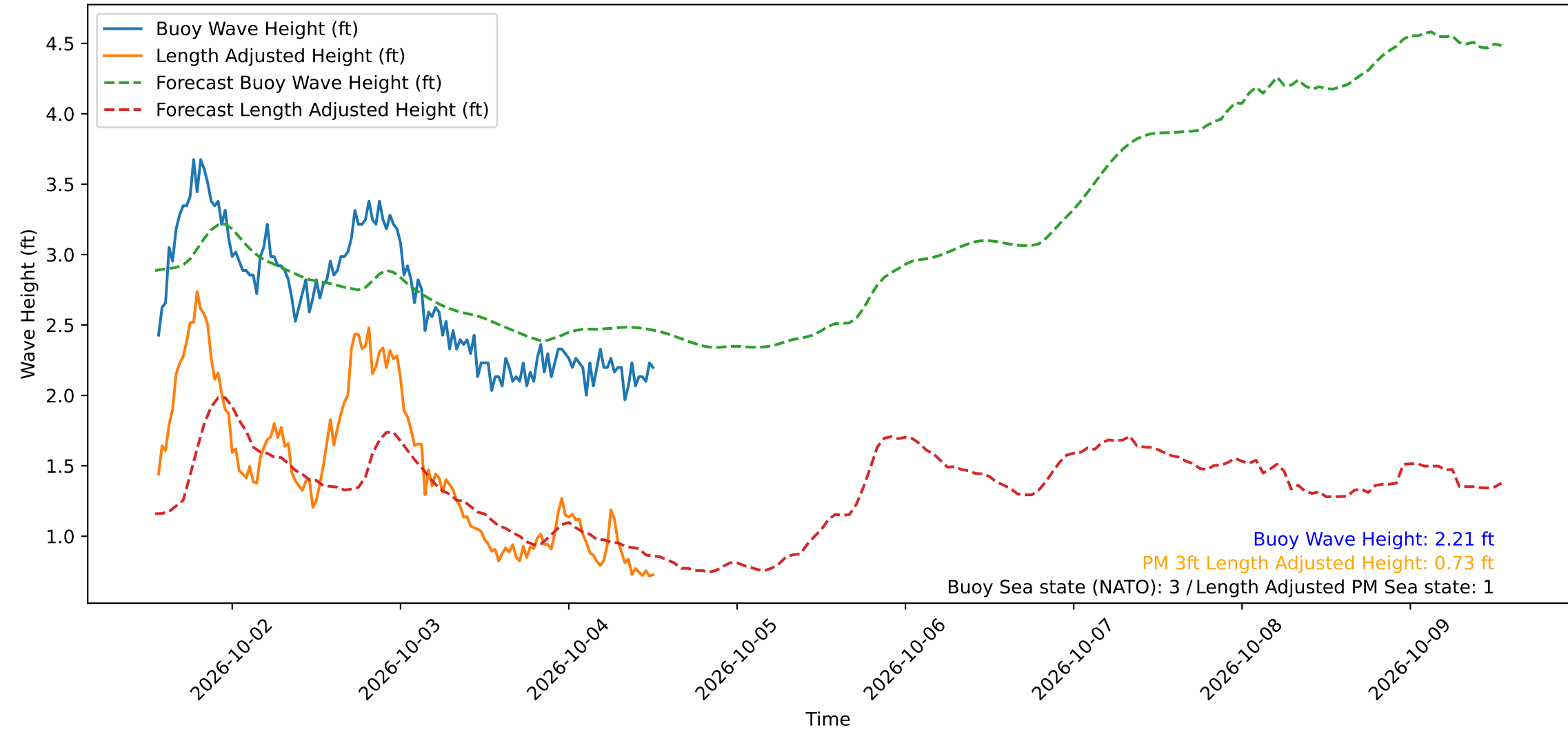
Wave Heights over Time for Green Beach at 2026-10-04 13:01:12
