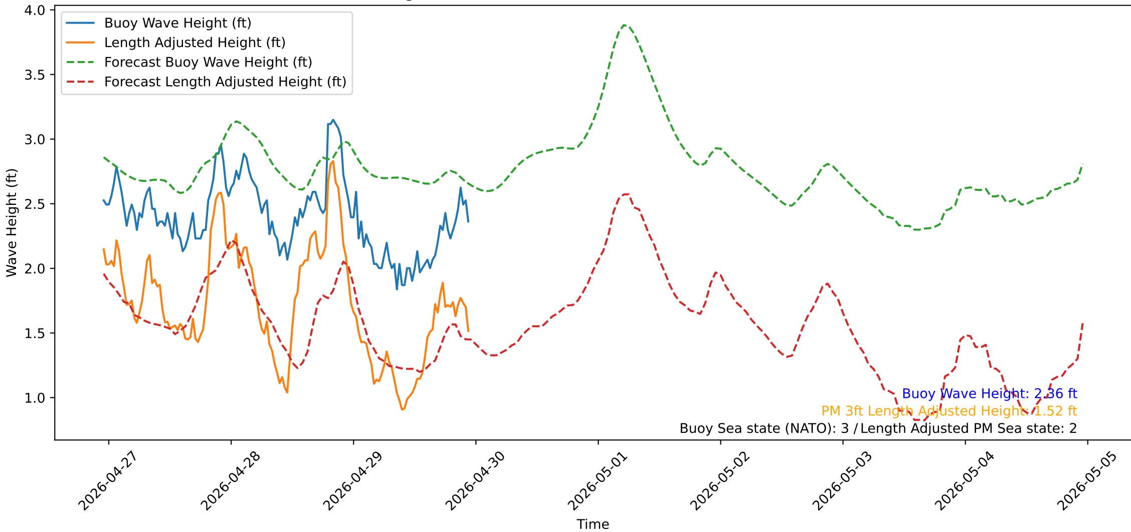
Wave Heights over Time for Green Beach at 2026-04-29 23:11:13
