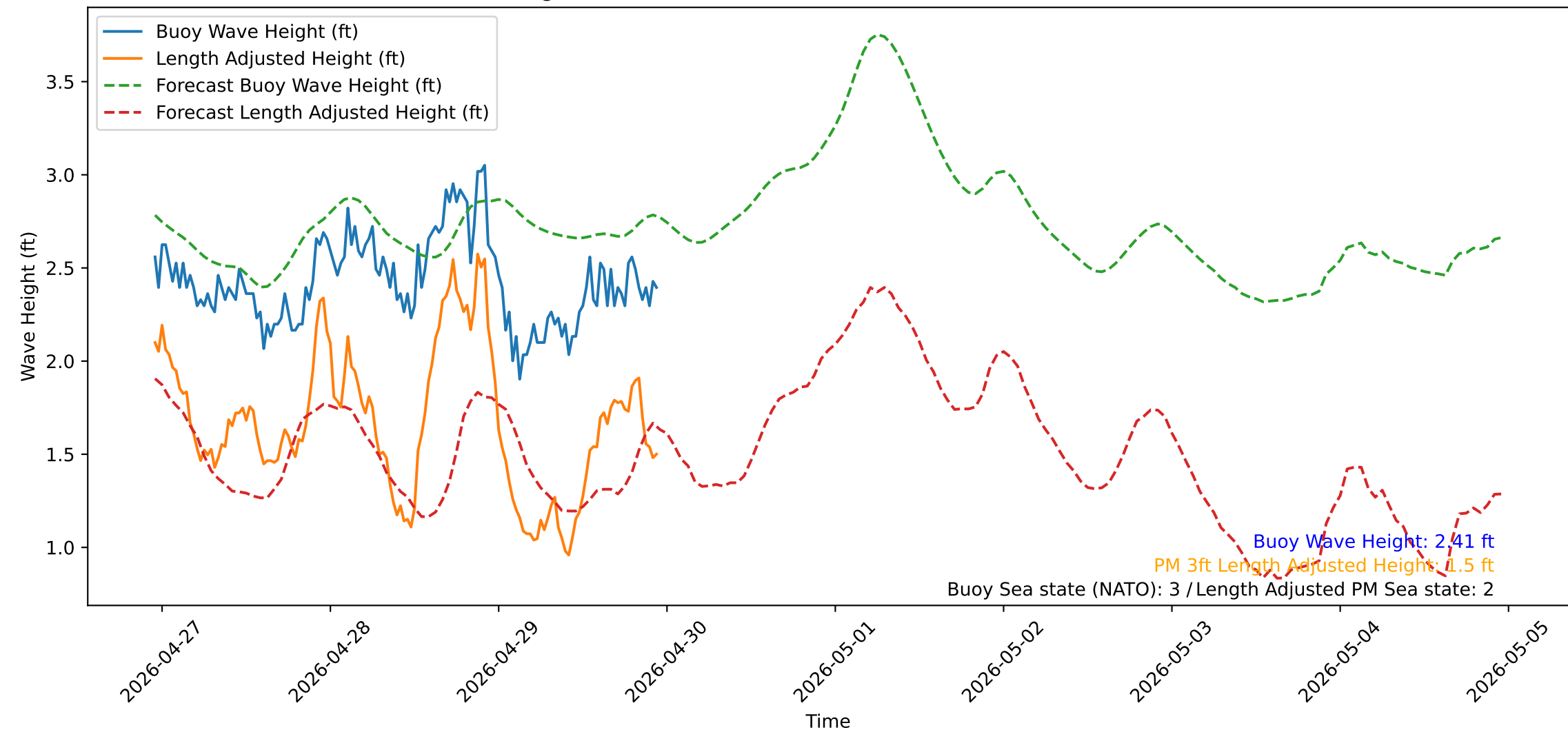
Wave Heights over Time for Oceanside Harbor at 2026-04-29 23:10:32
