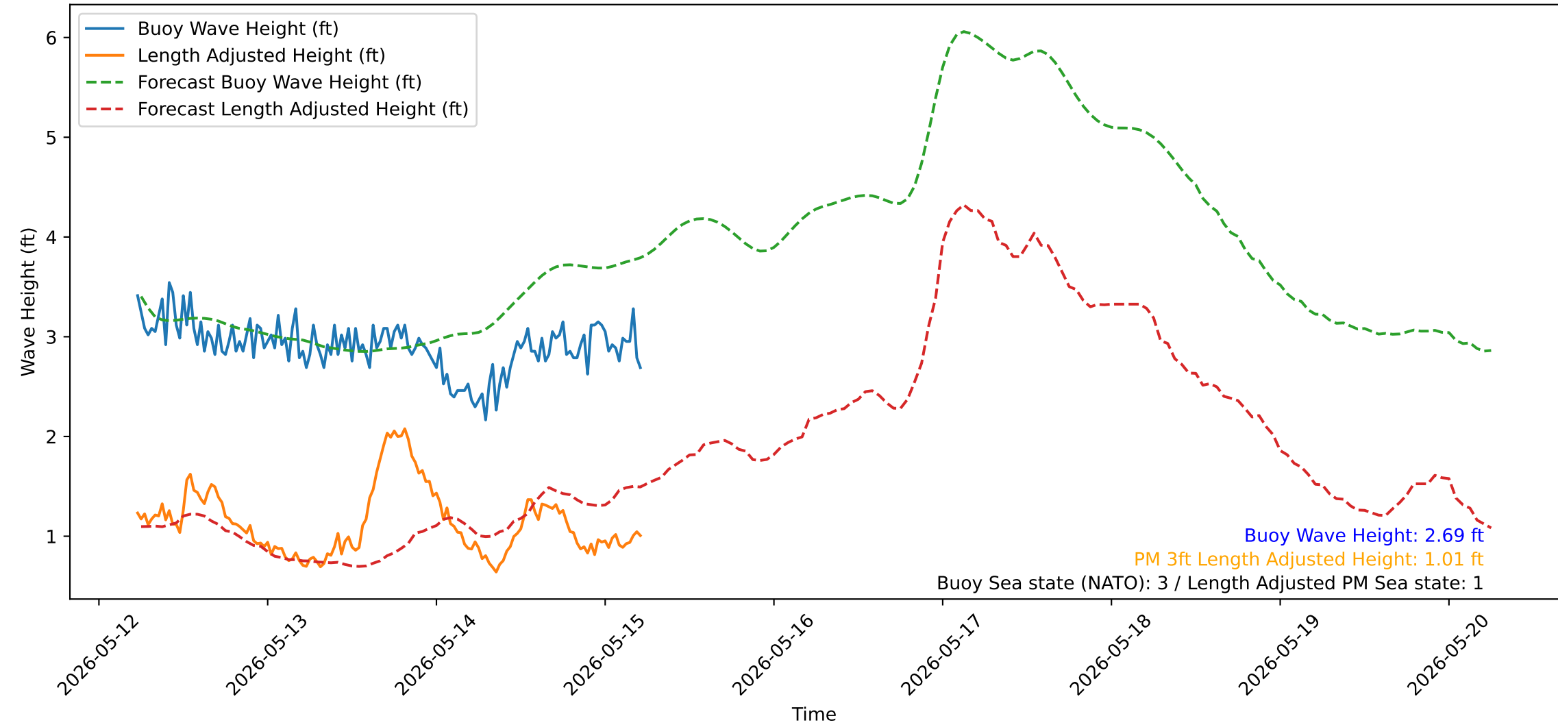
Wave Heights over Time for Oceanside Harbor at 2026-05-15 05:40:32
