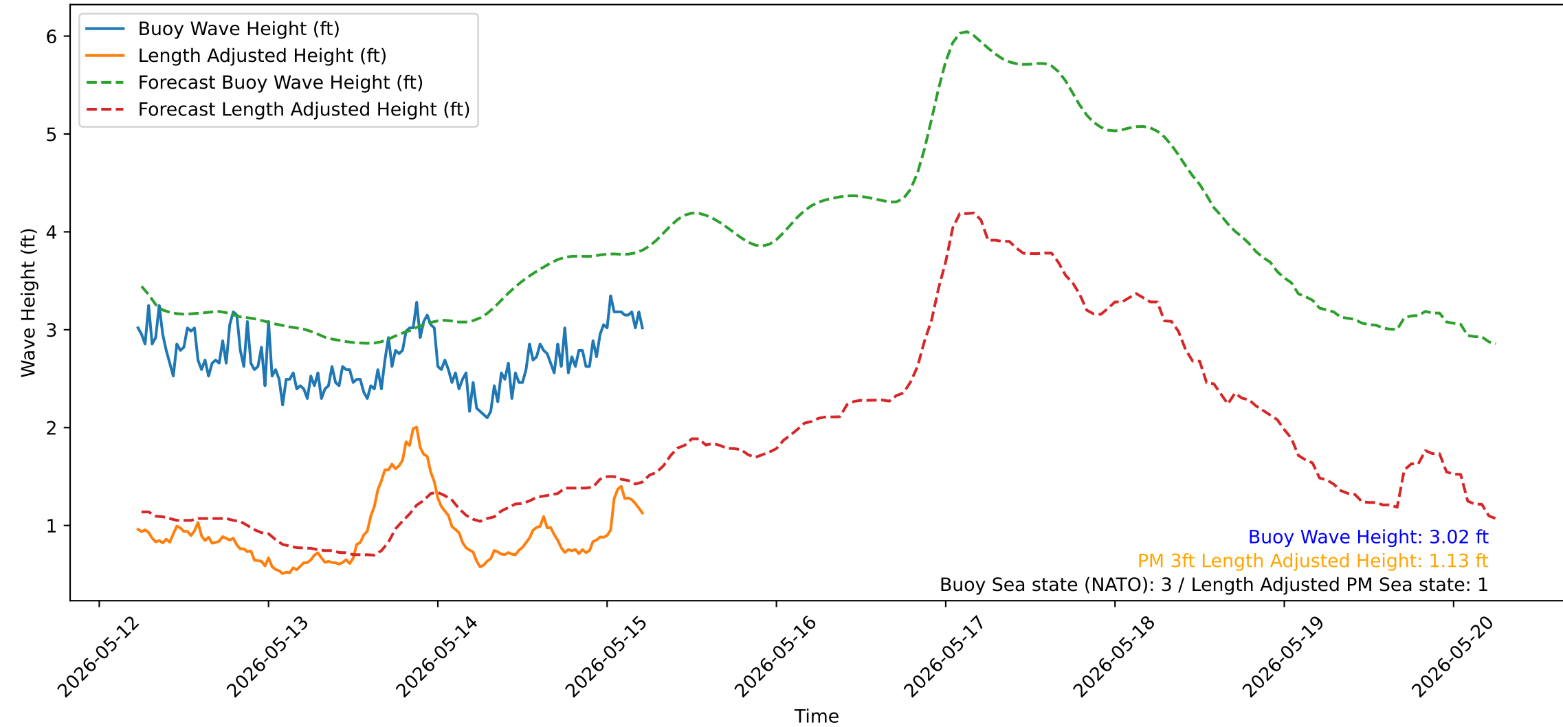
Wave Heights over Time for Green Beach at 2026-05-15 05:41:14
