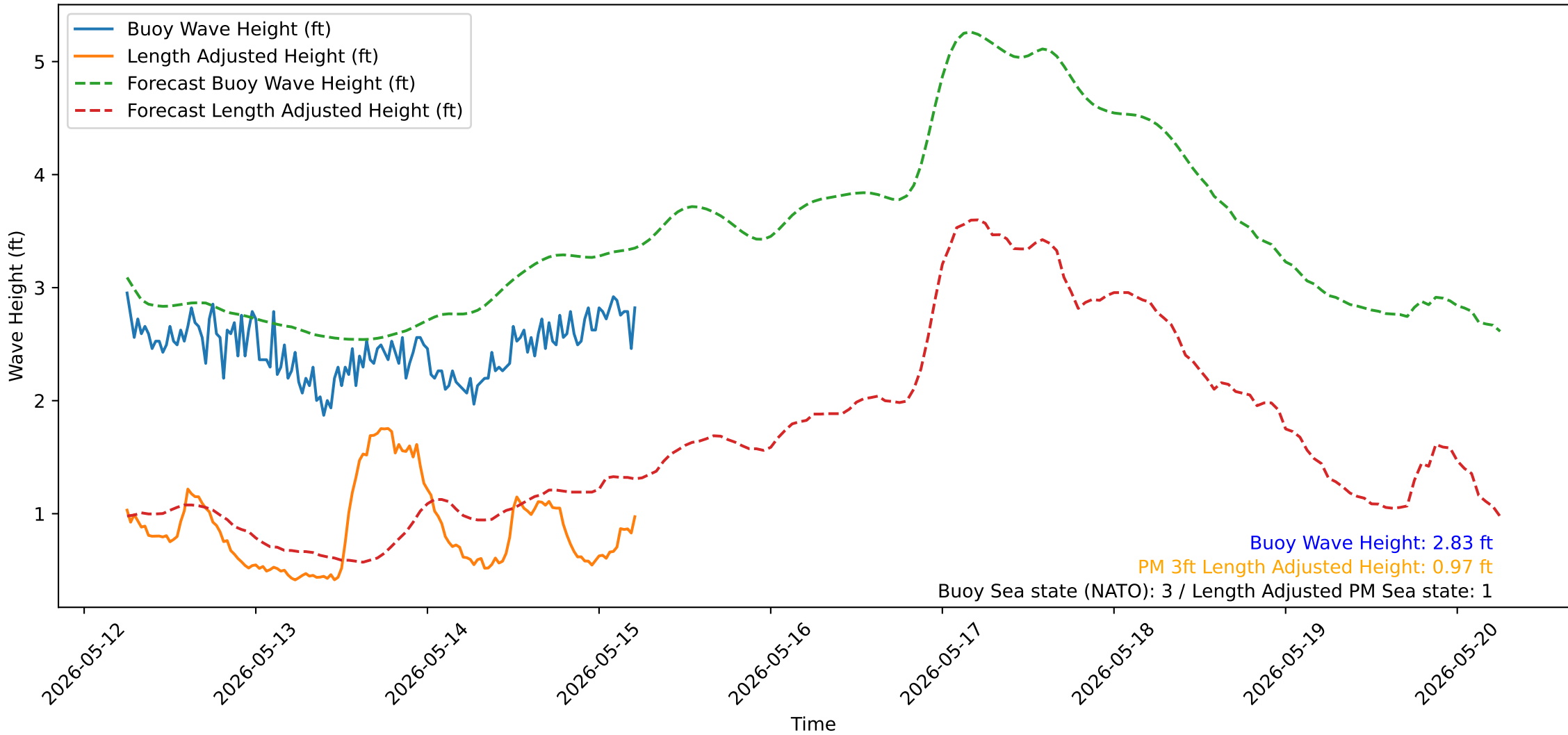
Wave Heights over Time for Red Beach at 2026-05-15 05:40:51
