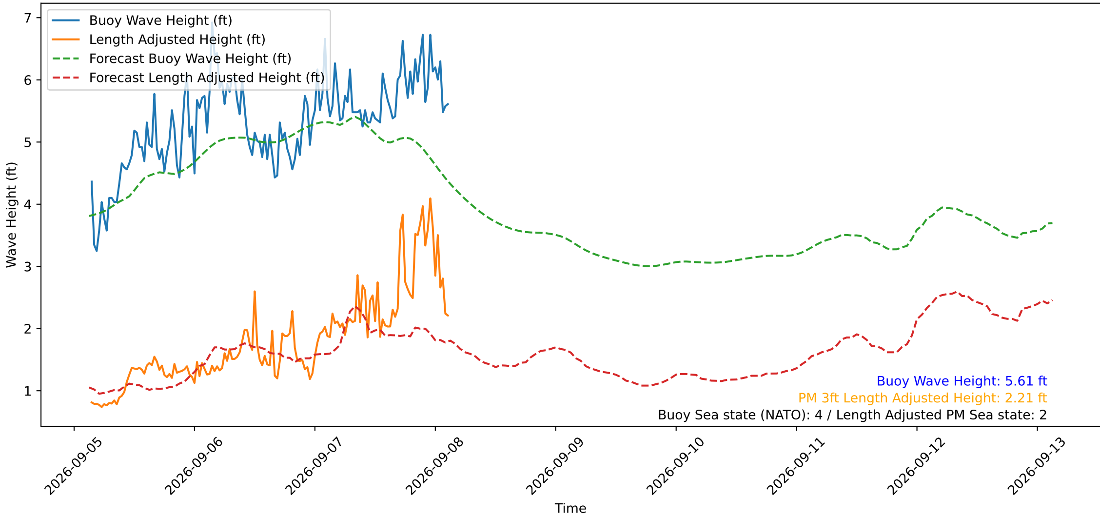
Wave Heights over Time for Red Beach at 2026-09-08 03:20:49
