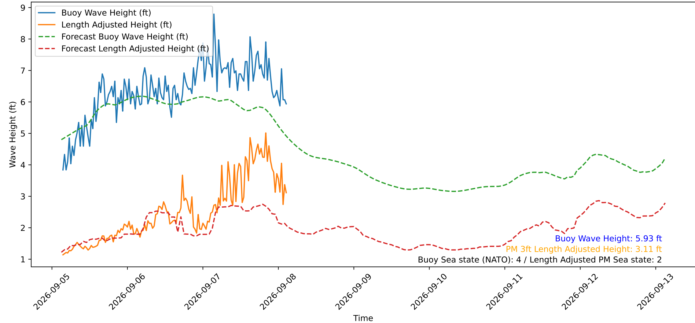
Wave Heights over Time for Green Beach at 2026-09-08 03:21:13
