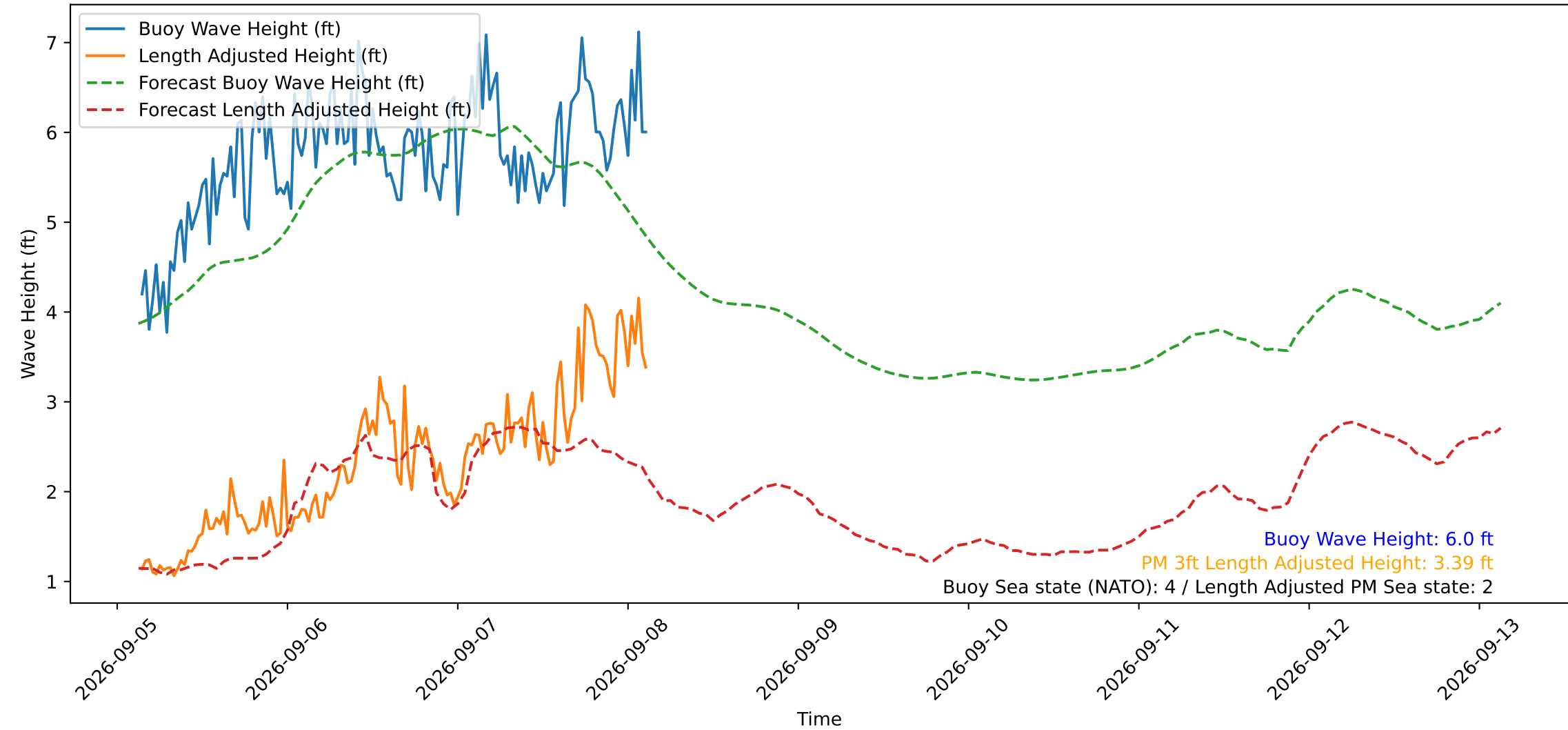
Wave Heights over Time for Oceanside Harbor at 2026-09-08 03:20:29
