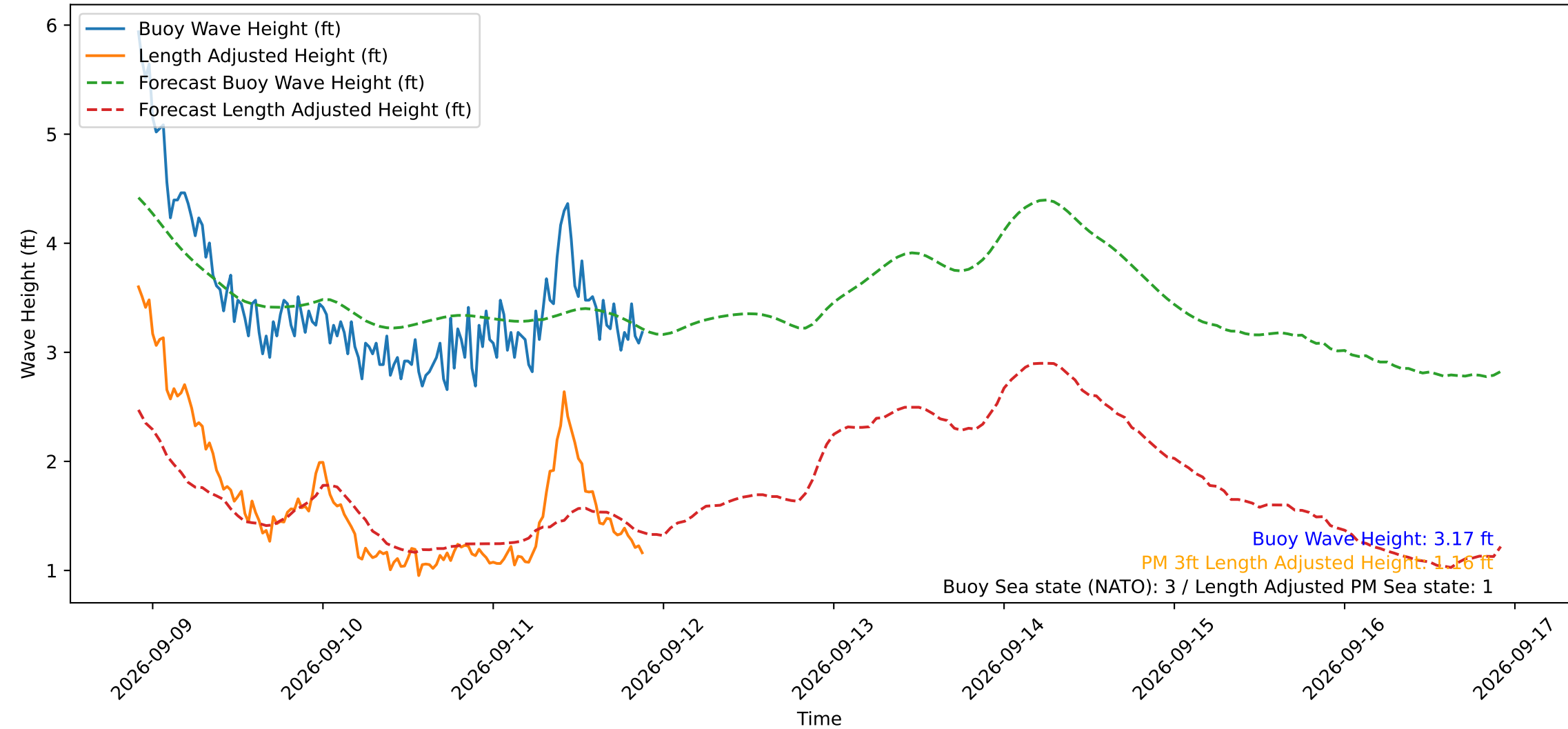
Wave Heights over Time for Oceanside Harbor at 2026-09-11 21:50:30
