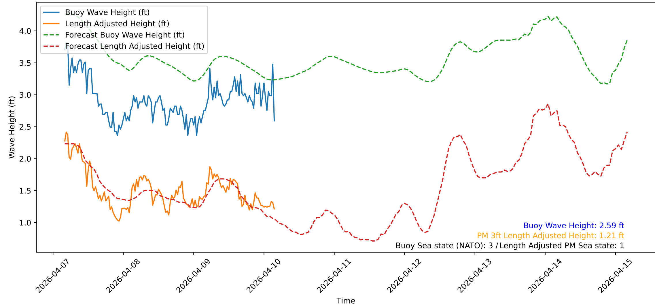
Wave Heights over Time for Green Beach at 2026-04-10 04:11:12
