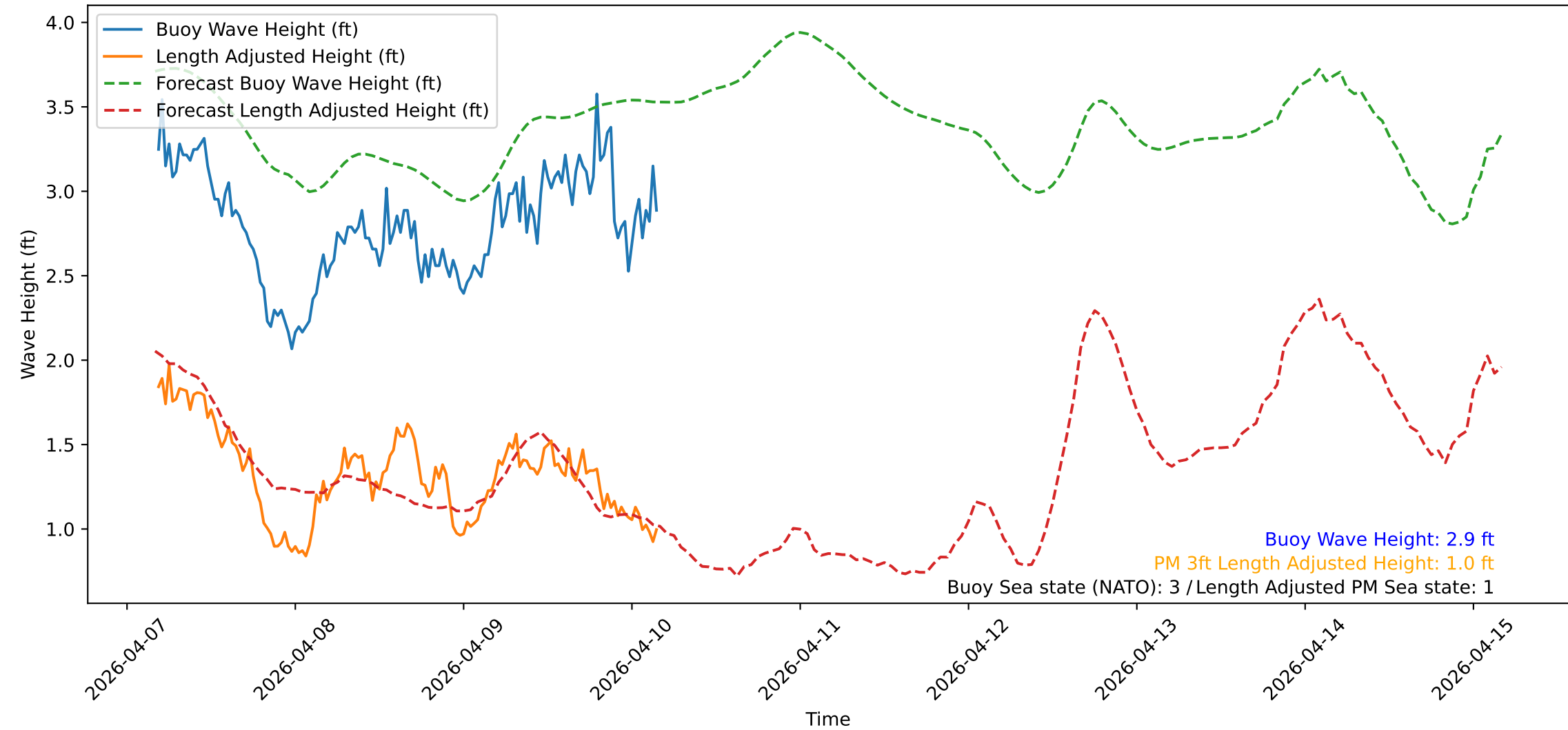
Wave Heights over Time for Red Beach at 2026-04-10 04:10:50
