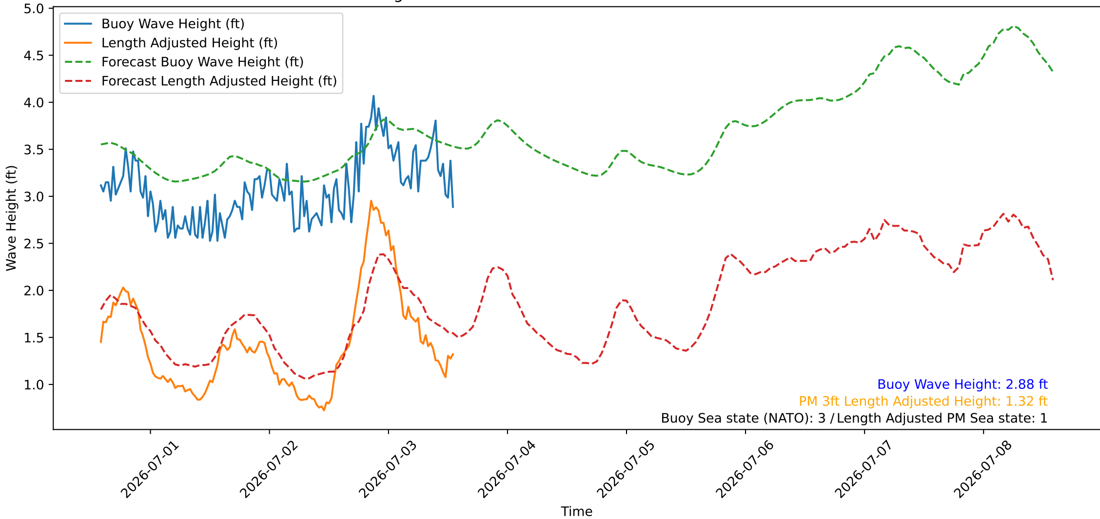
Wave Heights over Time for Green Beach at 2026-07-03 14:01:09
