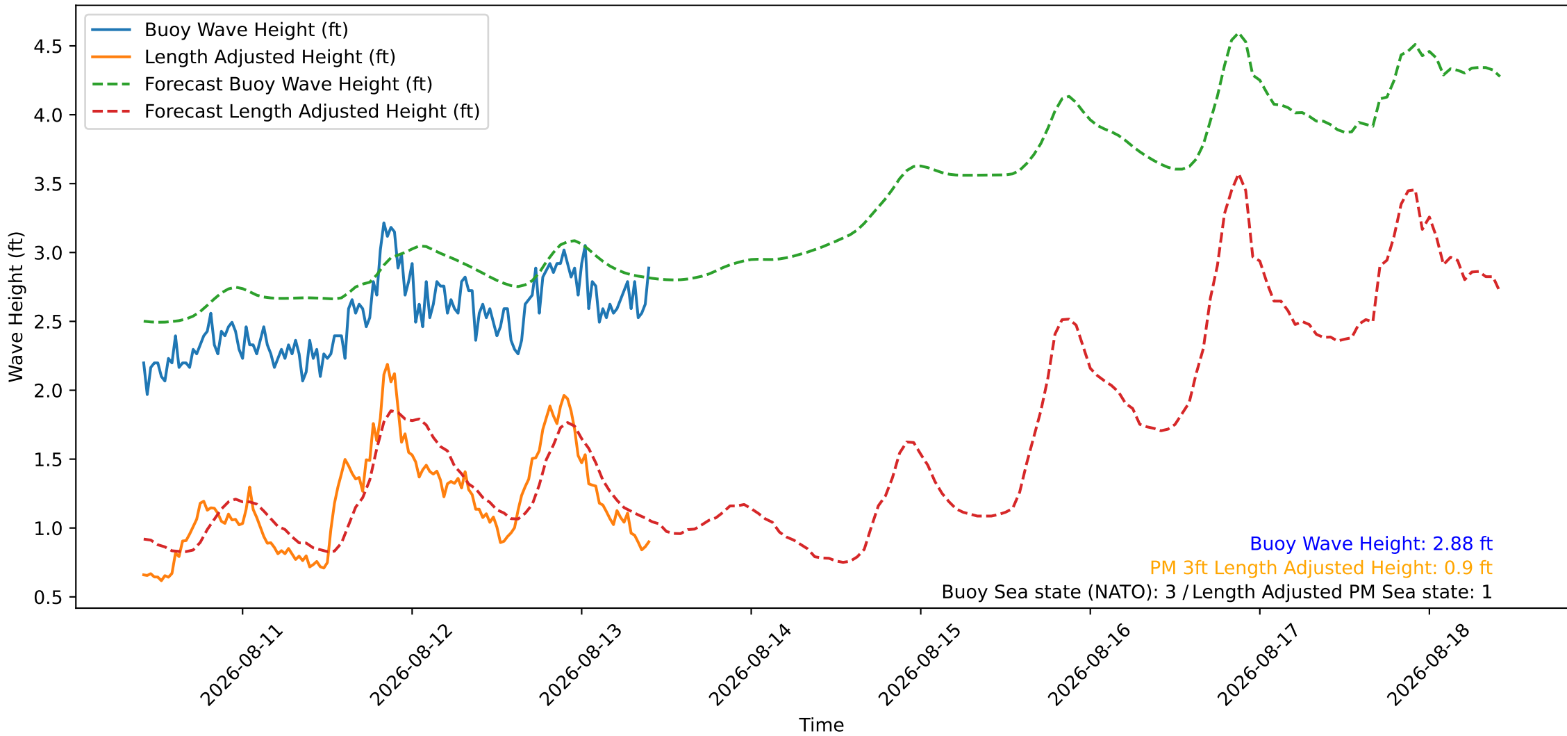
Wave Heights over Time for Green Beach at 2026-08-13 10:11:08
