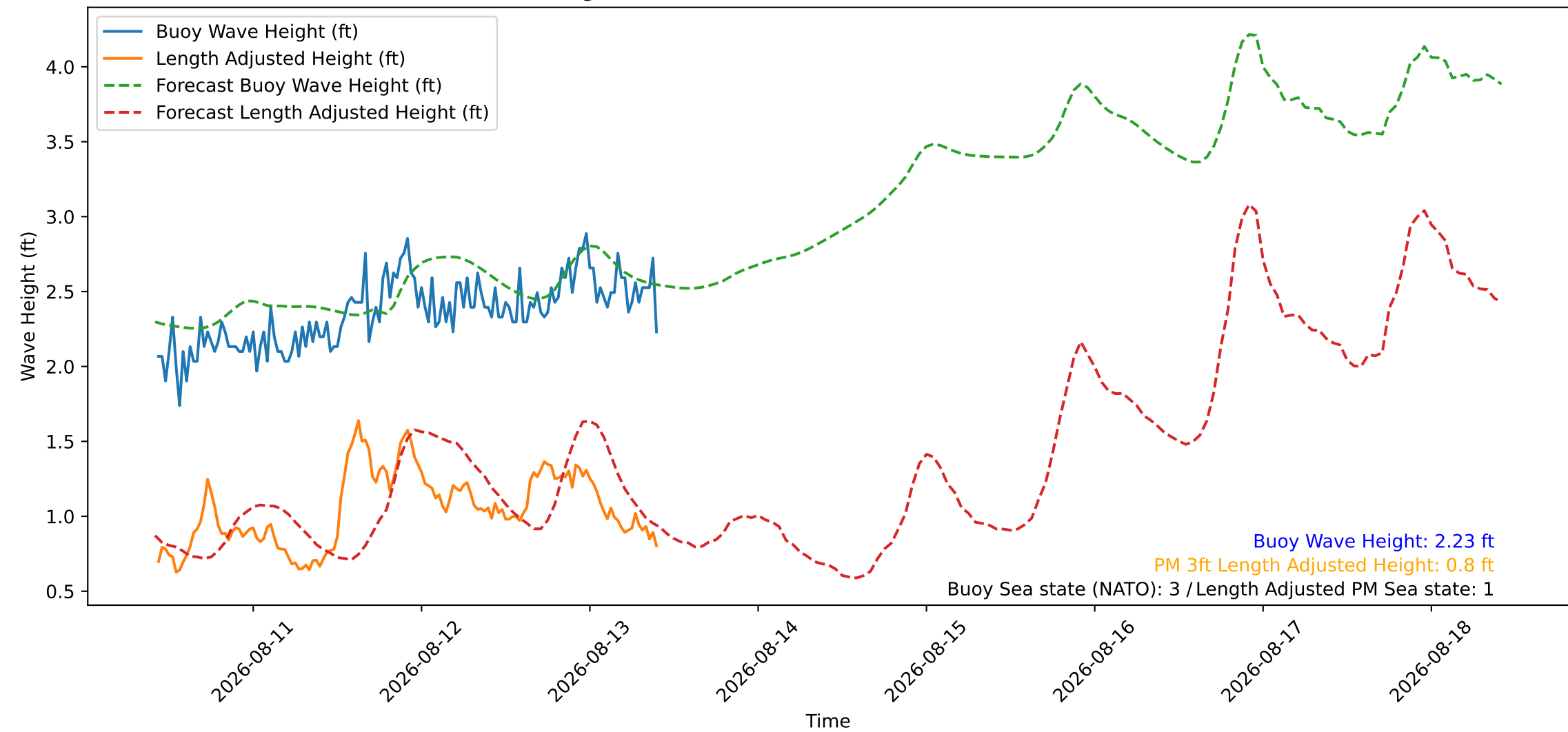
Wave Heights over Time for Red Beach at 2026-08-13 10:10:45
