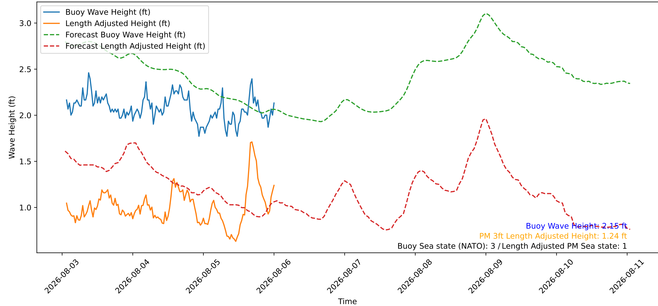
Wave Heights over Time for Red Beach at 2026-08-06 01:10:45
