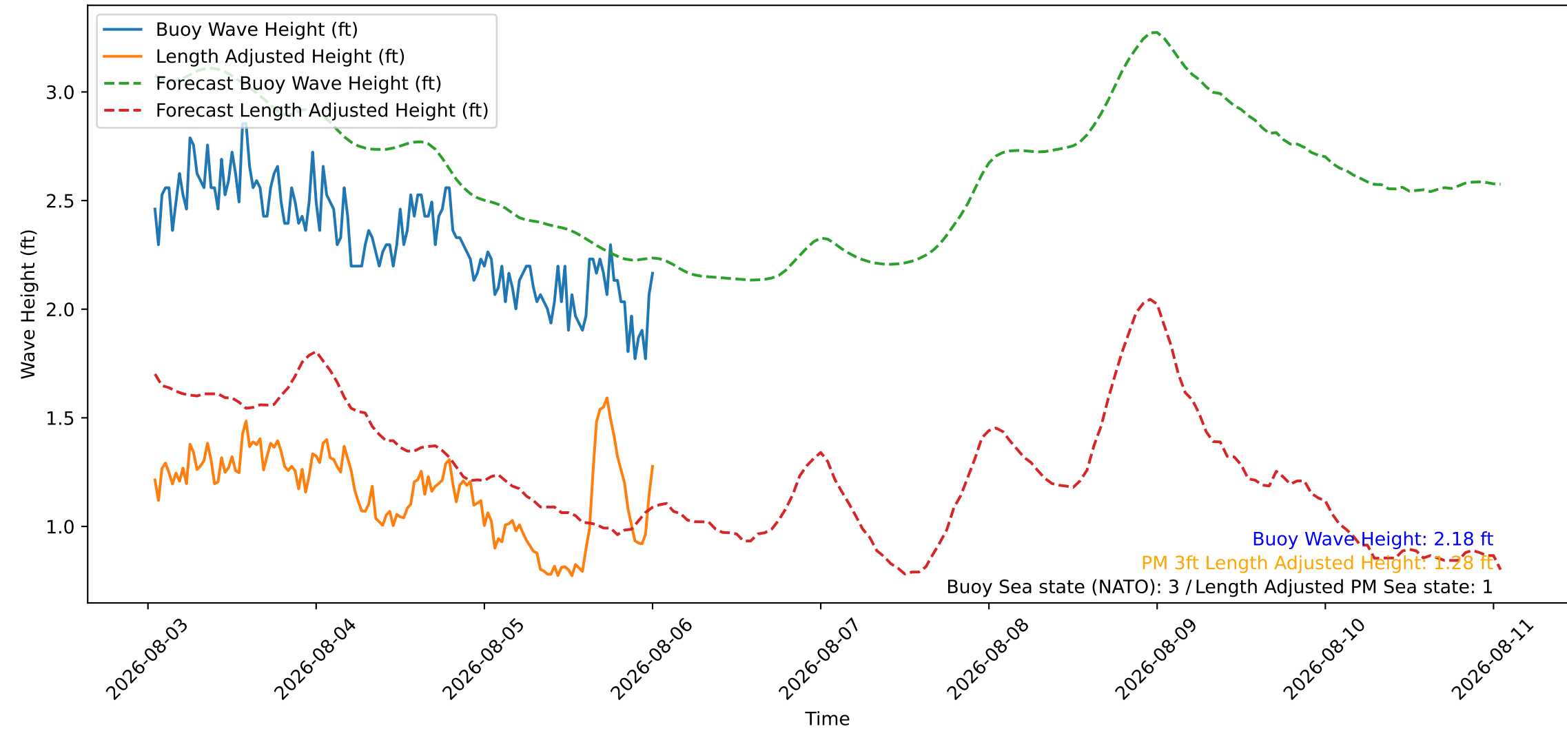
Wave Heights over Time for Oceanside Harbor at 2026-08-06 01:10:26
