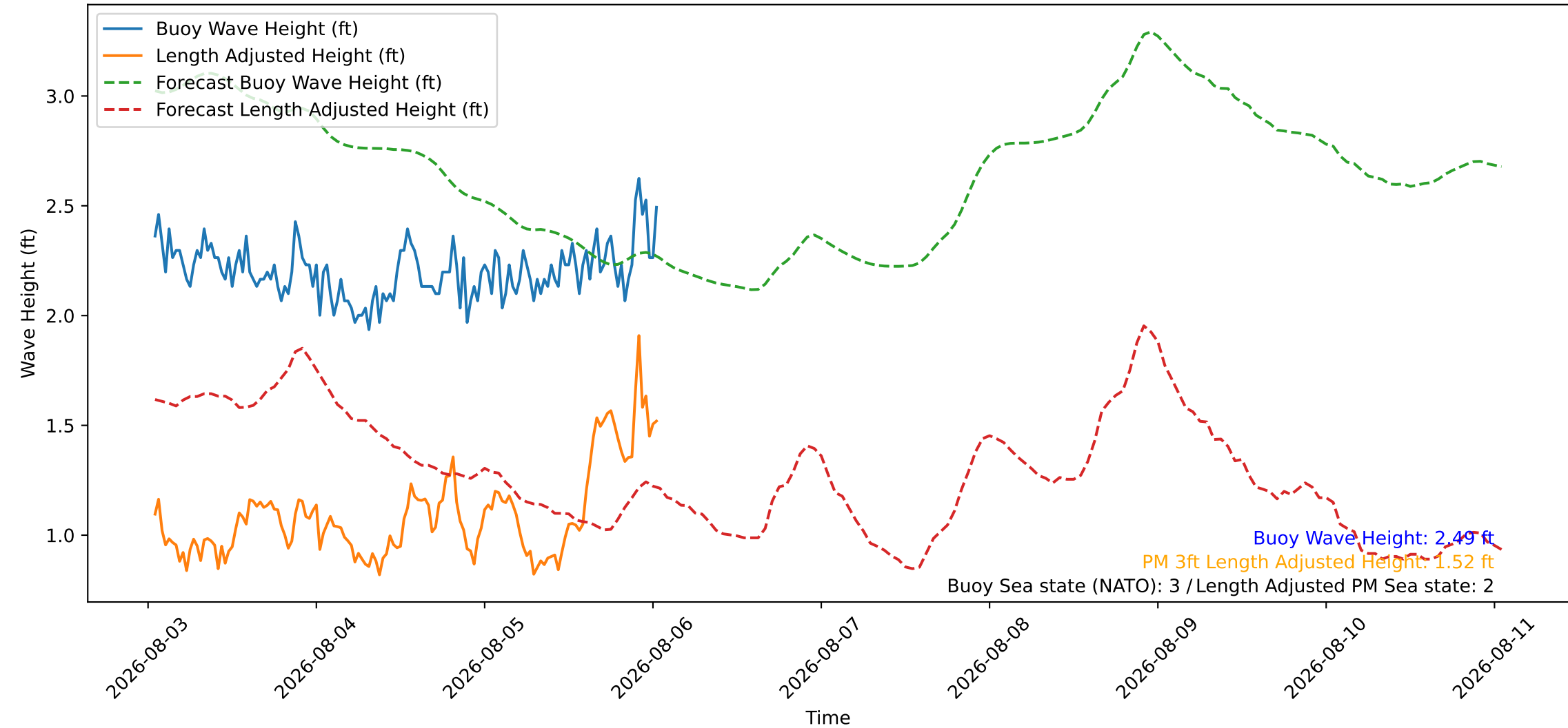
Wave Heights over Time for Green Beach at 2026-08-06 01:11:08
