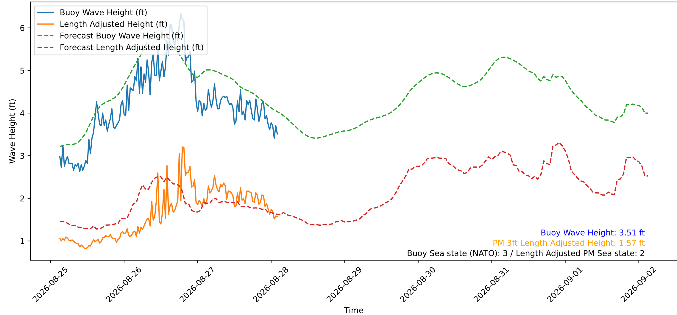
Wave Heights over Time for Green Beach at 2026-08-28 02:51:14
