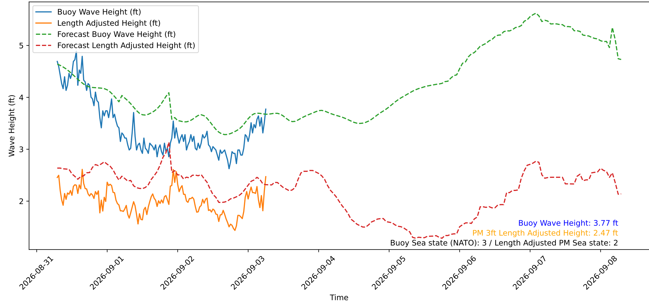
Wave Heights over Time for Oceanside Harbor at 2026-09-03 06:50:29
