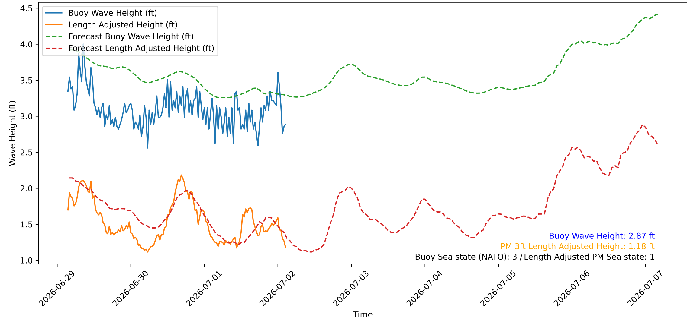
Wave Heights over Time for Oceanside Harbor at 2026-07-02 03:30:26
