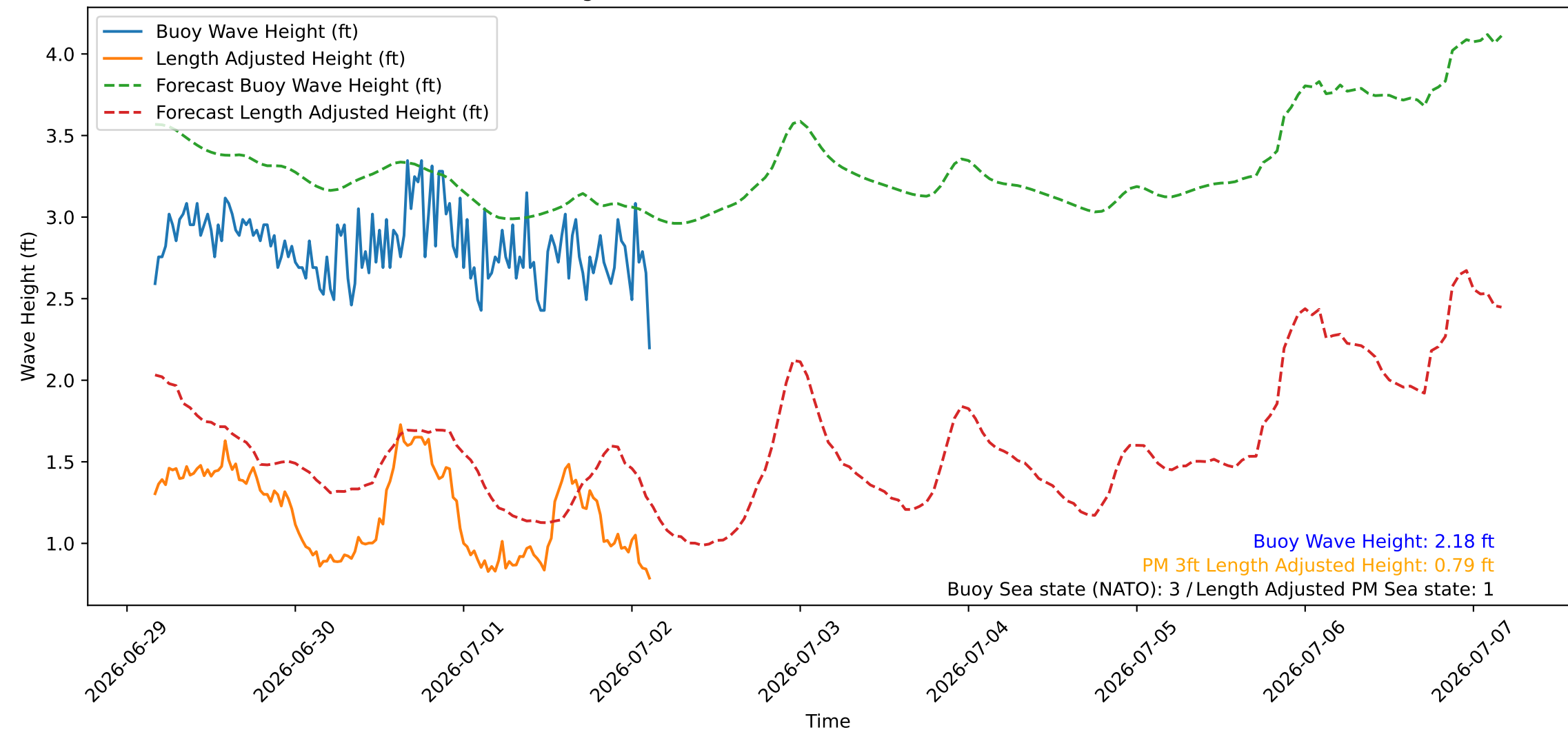
Wave Heights over Time for Red Beach at 2026-07-02 03:30:45
